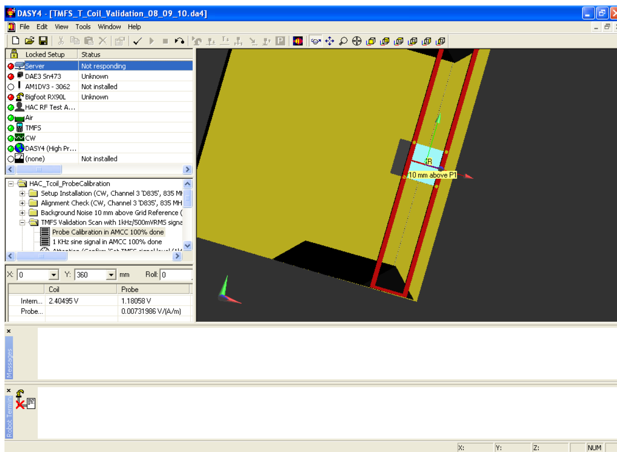
Figure 6.1. DASY4 ABM probe calibration
