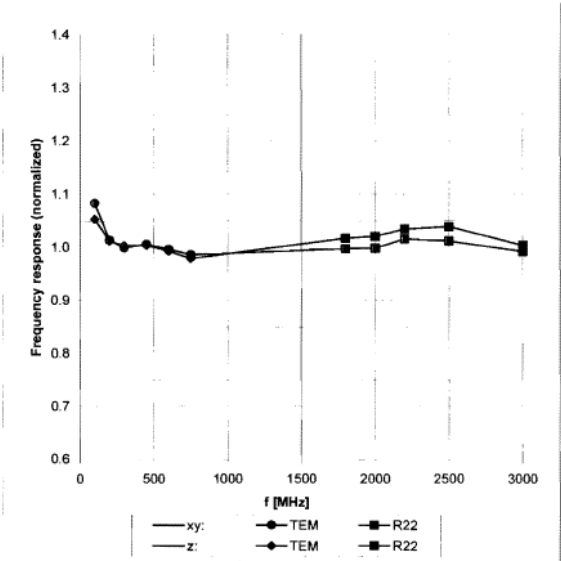
Frequency Response of H-Field (TEM-Cell:ifi110 EXX, Waveguide R22)
