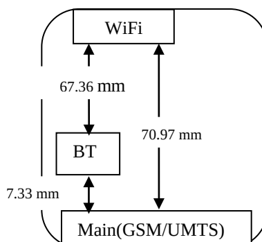
Figure 1.9.1. Back view of device showing closet distance between antenna pairs
