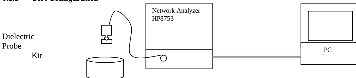
Figure 6.2.1. Test configuration
