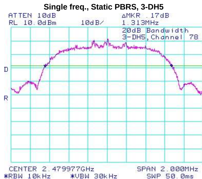
Figure 2-6: 20 dB Bandwidth
