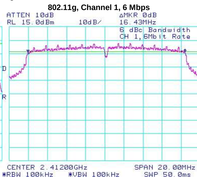
Figure 3-4: 6 dB Bandwidth
