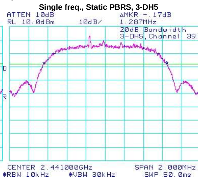
Figure 2-5: 20 dB Bandwidth
