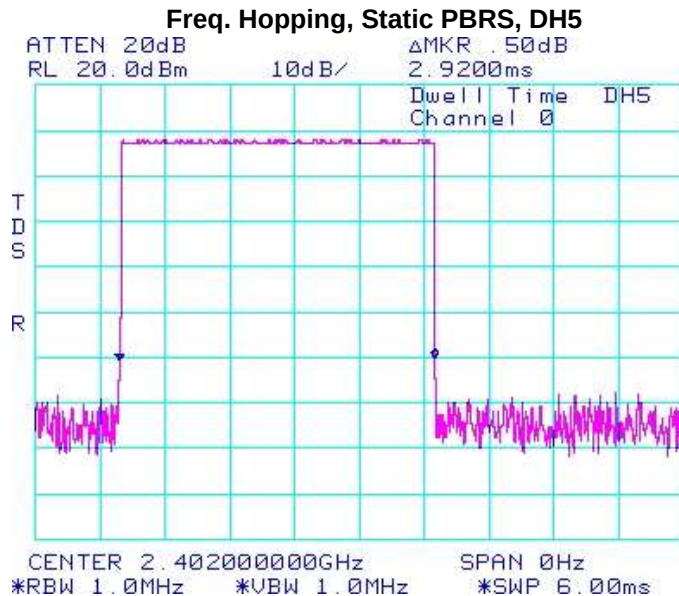
Figure 2-19: Time of Occupancy (Dwell Time)
