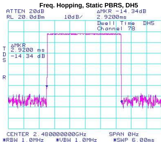
Figure 2-21: Time of Occupancy (Dwell Time)
