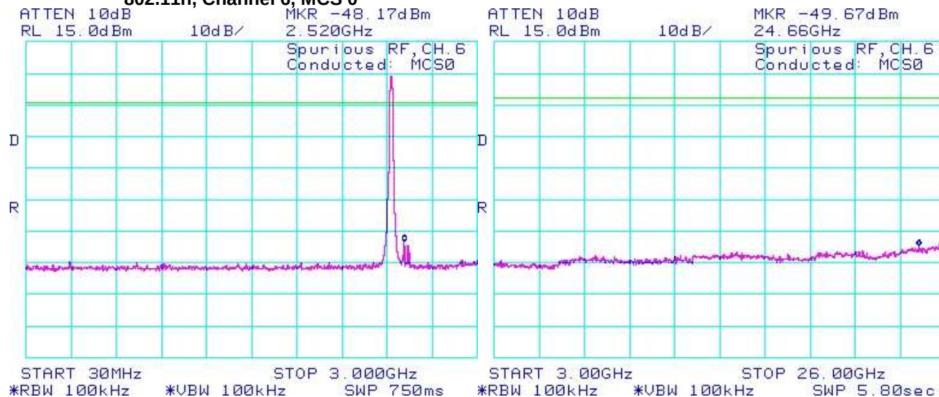
Figure 3-32: Spurious Conducted RF Emissions
