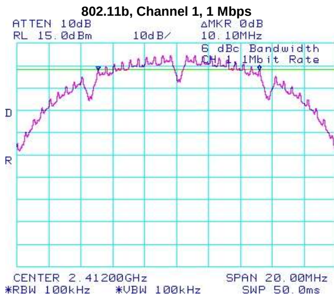
Figure 3-1: 6 dB Bandwidth
