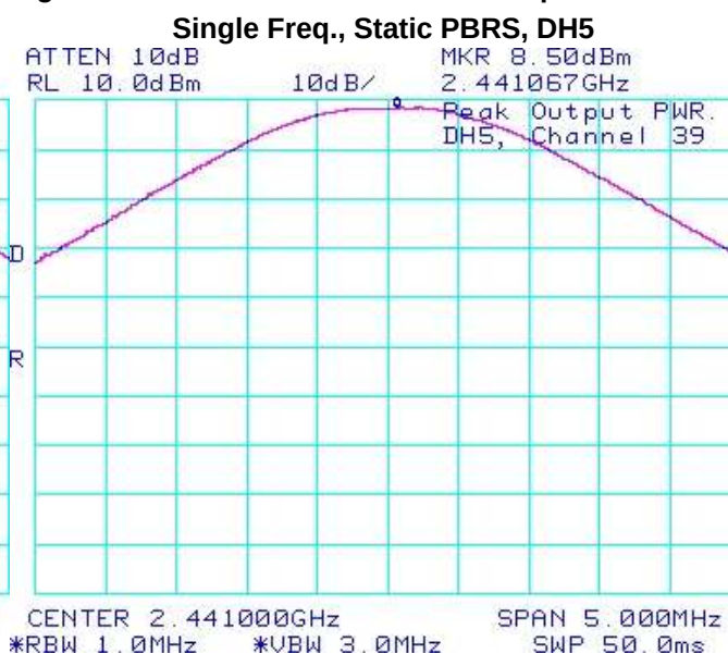
Figure 2-23: Max. Peak Conducted Output Power
