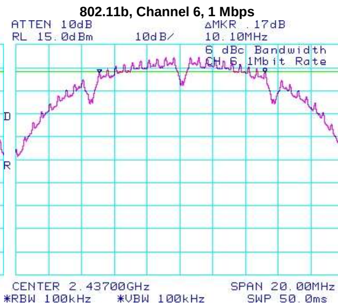
Figure 3-2: 6 dB Bandwidth
