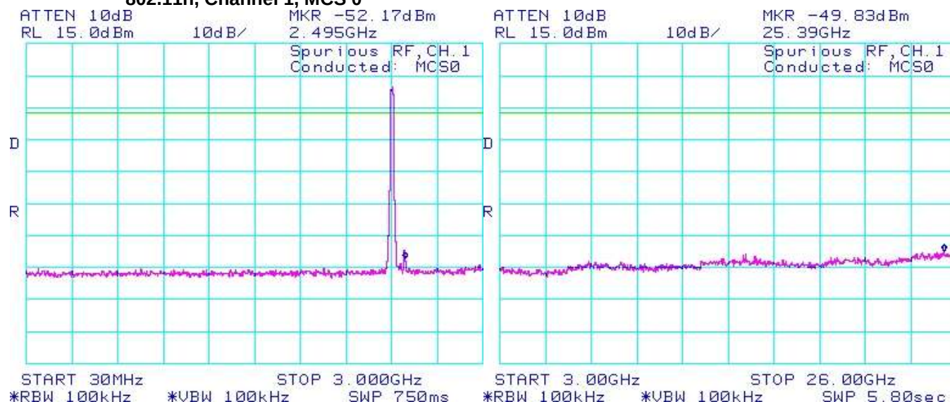
Figure 3-31: Spurious Conducted RF Emissions
