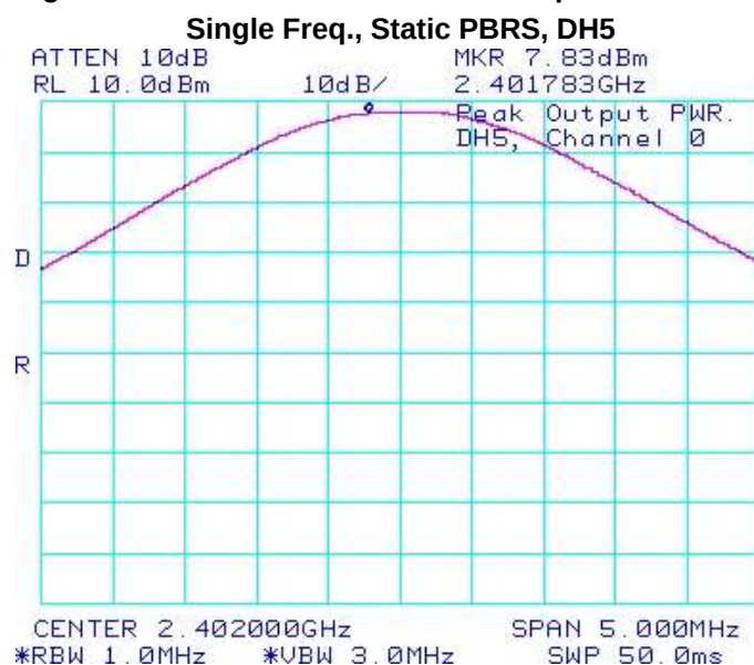
Figure 2-22: Max. Peak Conducted Output Power
