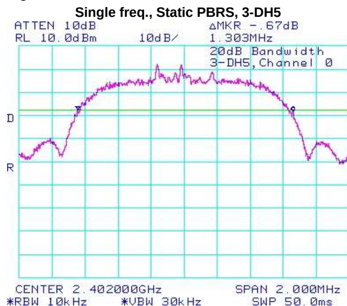
Figure 2-4: 20 dB Bandwidth
