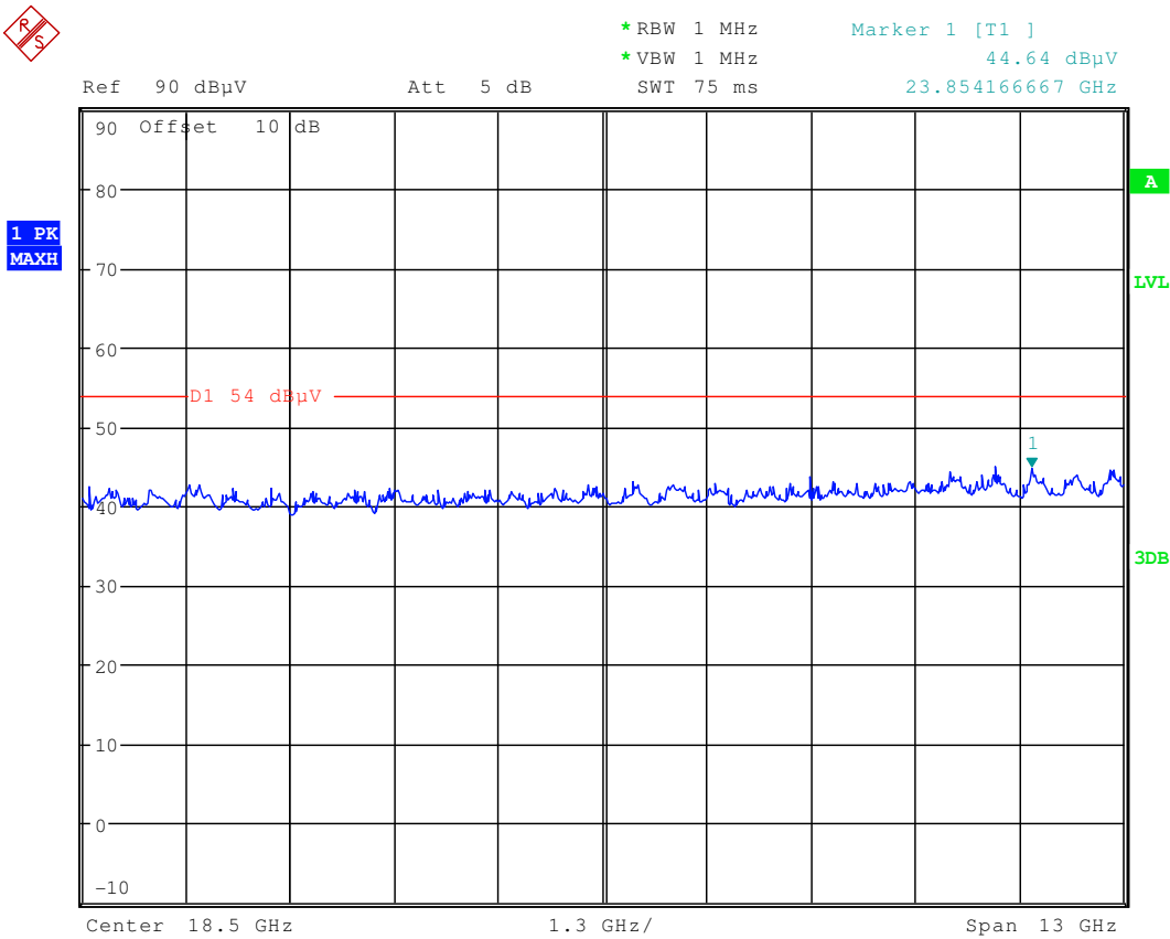
Plot 4: 12- 25 GHz (valid for all channels)
