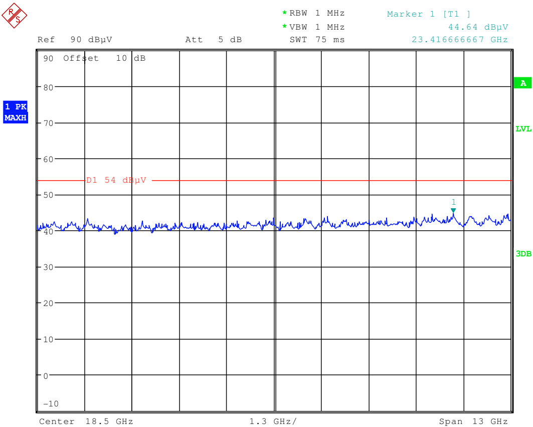
Plot 3: 12- 25 GHz (valid for all channels)
