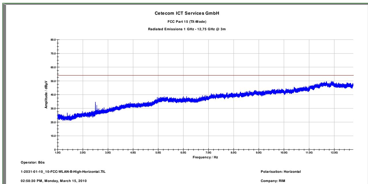
Plot 9: 1 – 12.75 GHz horizontal (high channel)
