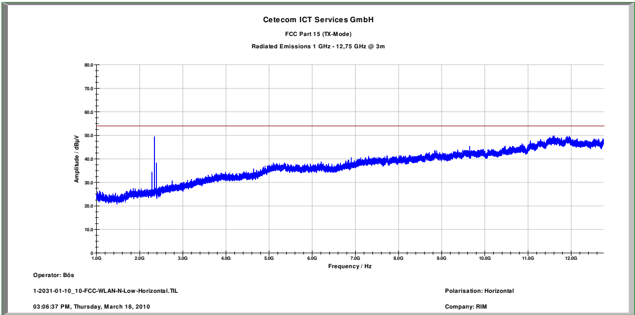
Plot 2: 1 – 12.75 GHz horizontal/vertical (lowest channel)
