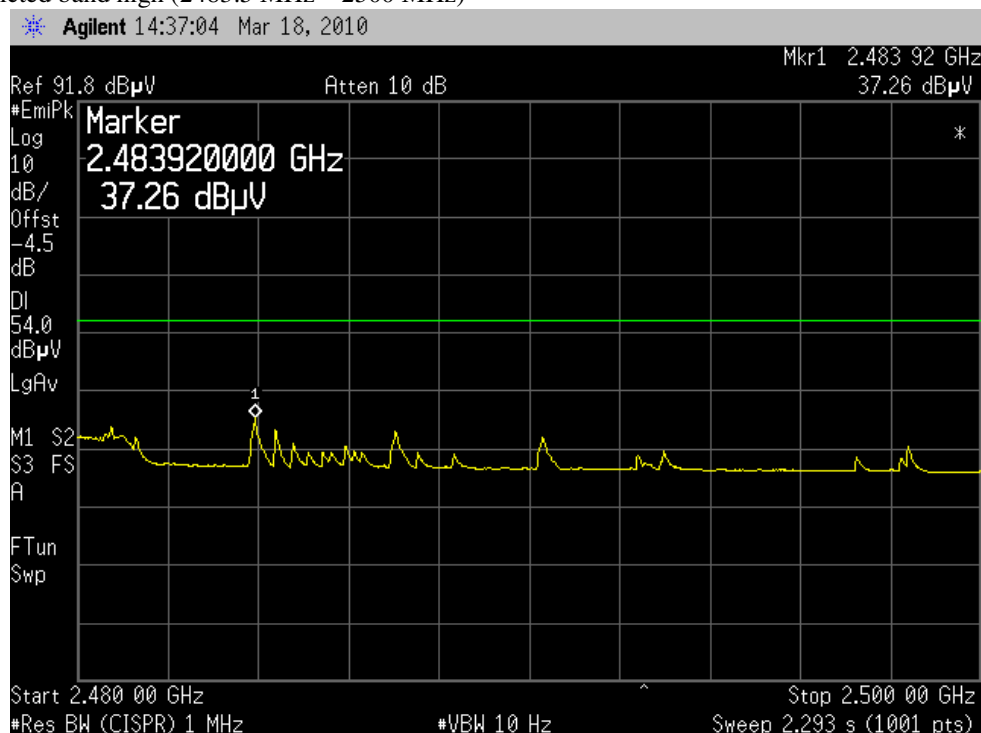
Plot 11: Restricted band high (2483.5 MHz – 2500 MHz)
