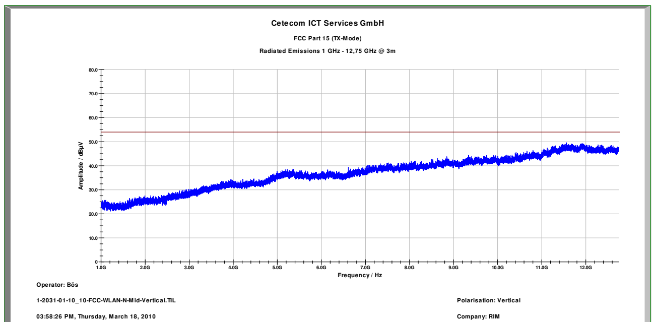
Plot 5: 1 – 12.75 GHz horizontal/vertical (middle channel)
