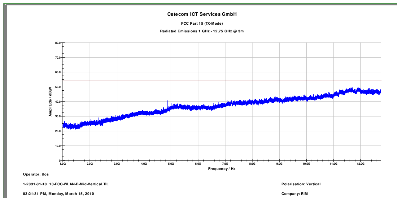
Plot 7: 1 – 12.75 GHz vertical (middle channel)
