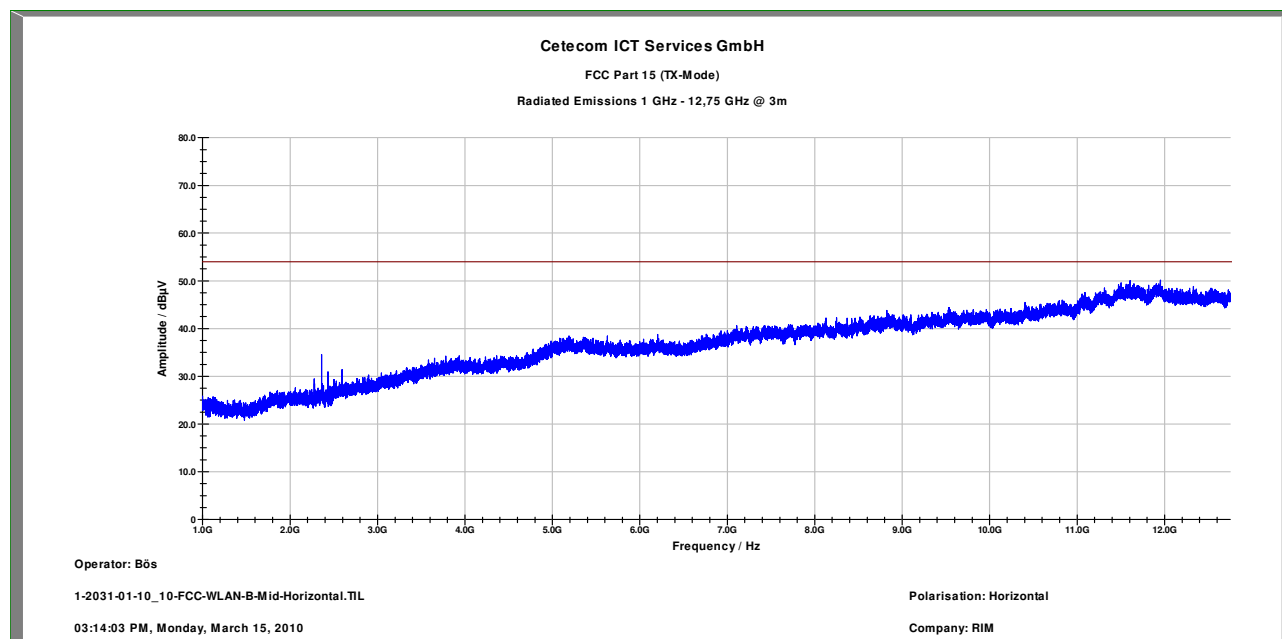
Plot 6: 1 – 12.75 GHz horizontal (middle channel)
