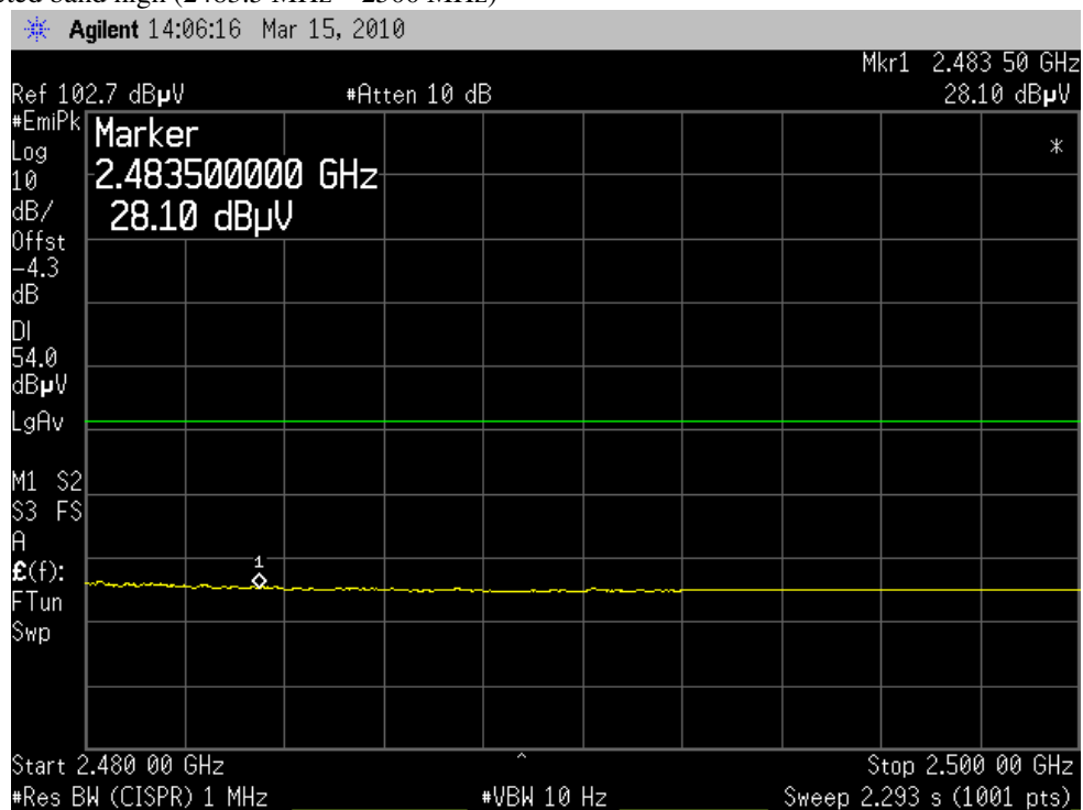
Plot 7: Restricted band high (2483.5 MHz – 2500 MHz)
