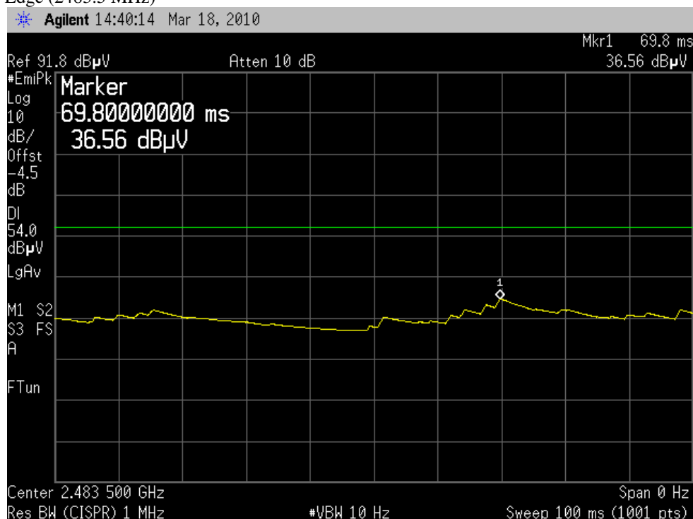
Plot 12: Band Edge (2483.5 MHz)
