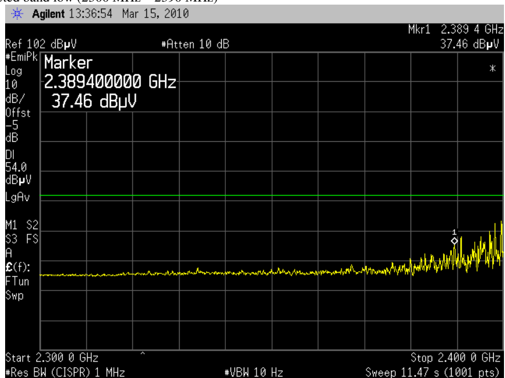
Plot 5: Restricted band low (2300 MHz – 2390 MHz)
