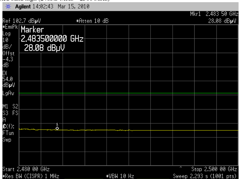
Plot 3: Restricted band high (2483.5 MHz – 2500 MHz)
