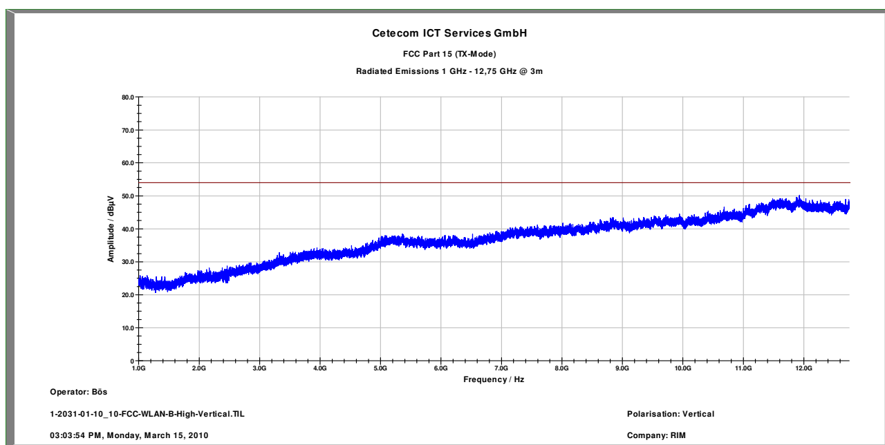
Plot 10: 1 – 12.75 GHz vertical (high channel)
