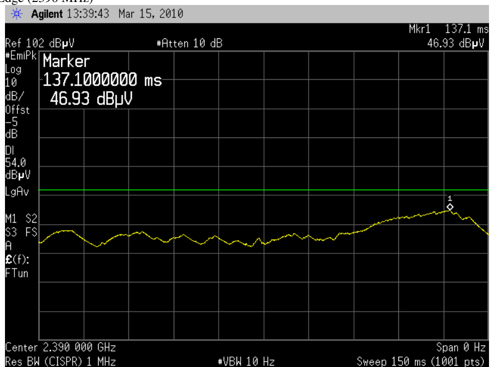
Plot 6: Band Edge (2390 MHz)
