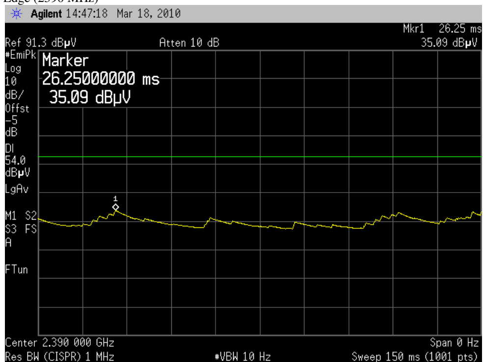
Plot 10: Band Edge (2390 MHz)
