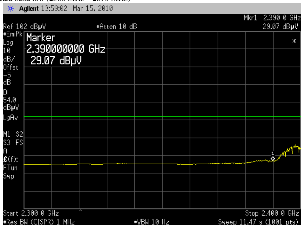
Plot 1: Restricted band low (2300 MHz – 2390 MHz)
