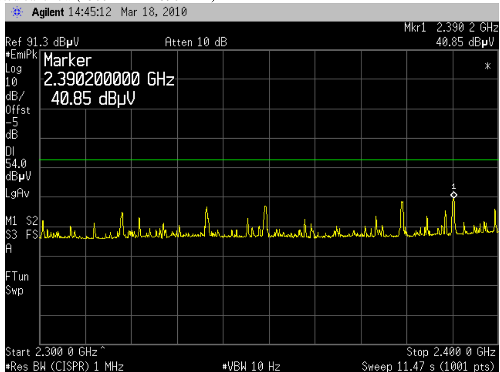
Plot 9: Restricted band low (2300 MHz – 2390 MHz)
