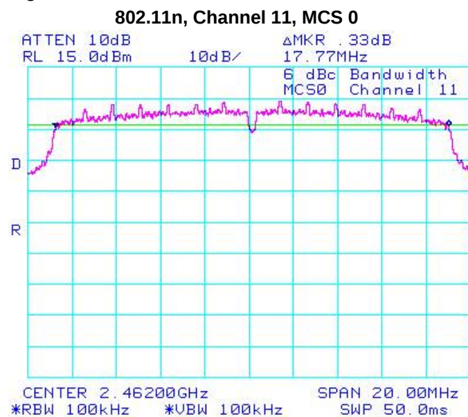
Figure 4-9: 6 dB Bandwidth
