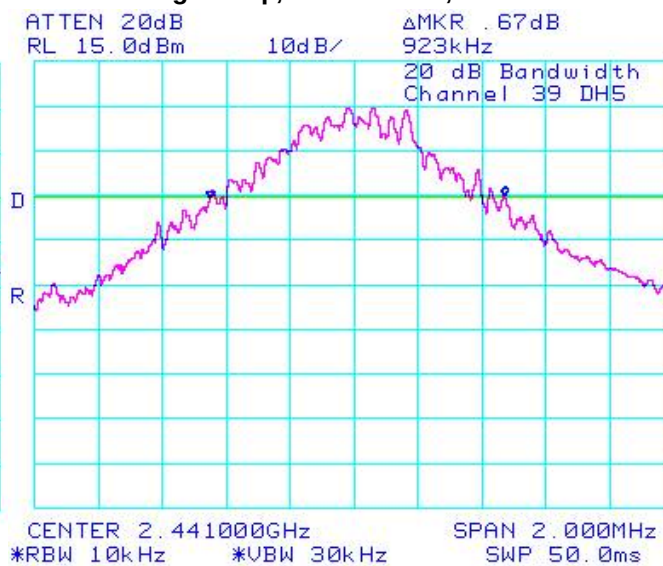
Figure 3-2: 20 dB Bandwidth
