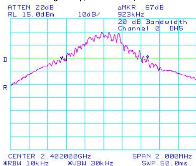
Figure 3-1: 20 dB Bandwidth
