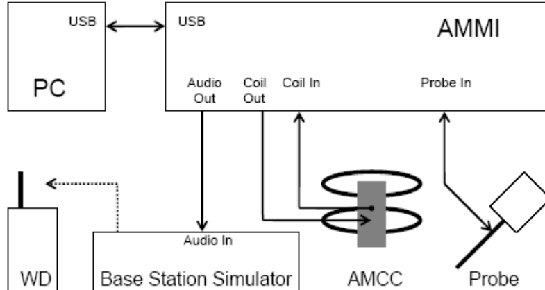
Figure 5.3. T-Coil set up cabling
