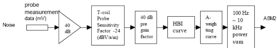
Figure 6.3. ABM2 measurement flow chart
