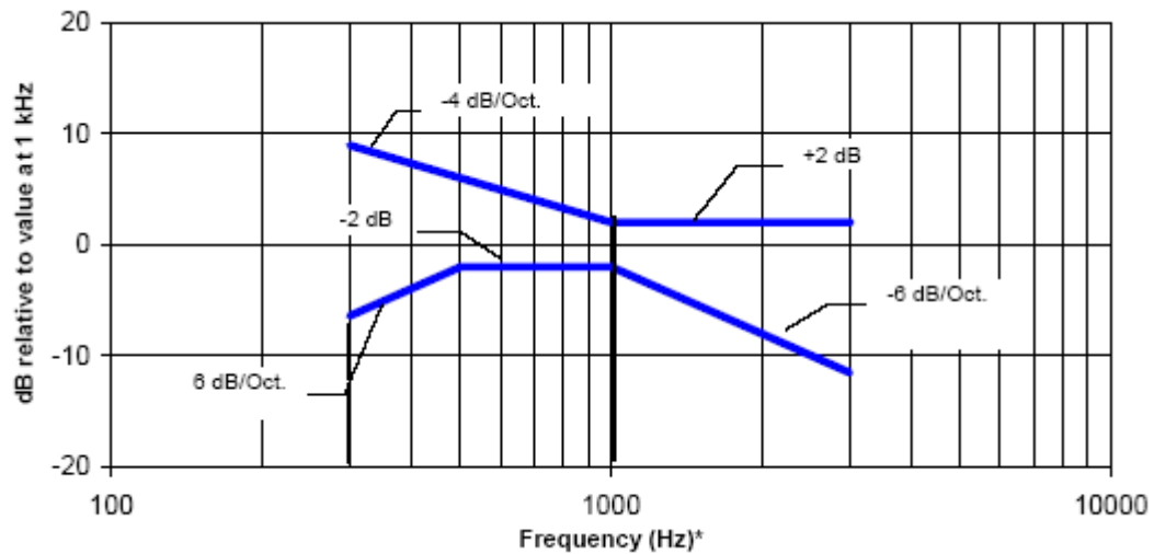
Figure 6.5. Magnetic field frequency response for WDs with a field between 10 dB and -13 dB (A/m) at 1 kHz
