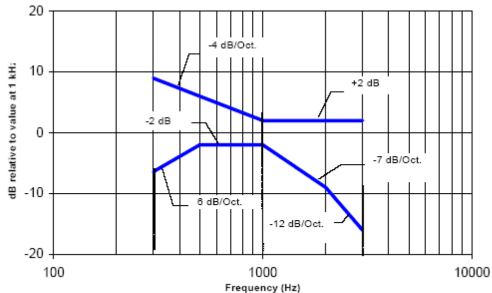
Figure 6.6. Magnetic field frequency response for WDs with a field that exceeds -10 dB(A/m) at 1 kHz
