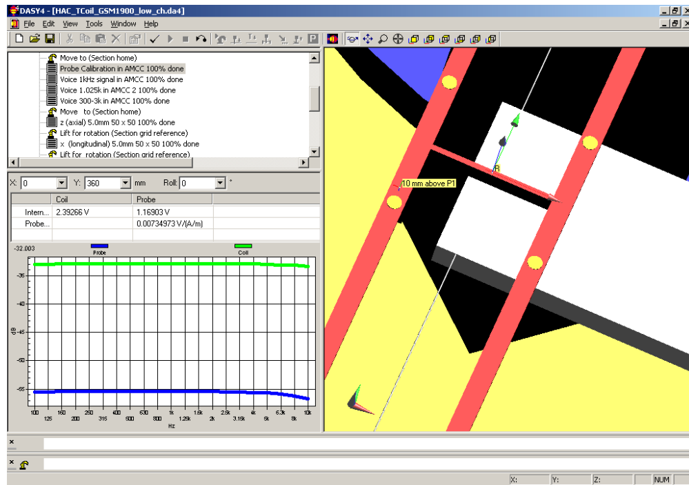
Figure 6.1. DASY4 ABM probe calibration
