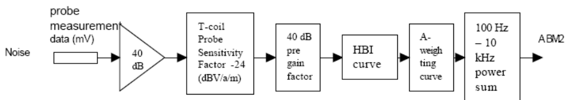
Figure 6.3. ABM2 measurement flow chart
