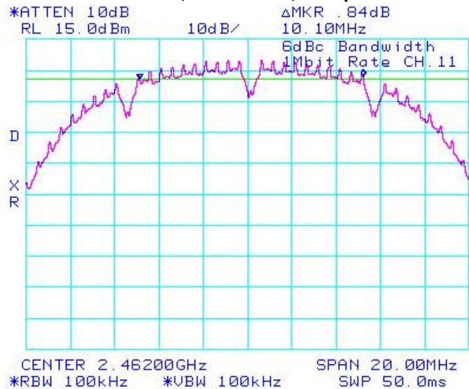
Figure 4-3: 6 dB Bandwidth
