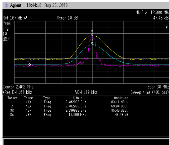
Figure 2-3: Band-Edge Compliance of RF Rad. Emissions.
