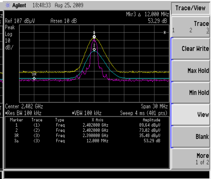
Figure 2-4: Band-Edge Compliance of RF Rad. Emissions
