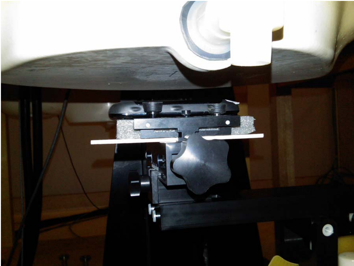
Figure E12. Body-worn configuration (No Holster, 25 mm away, back facing phantom)
