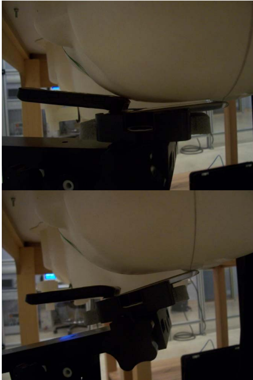
Figure E5. Head configuration (Left Touch/Tilt)
