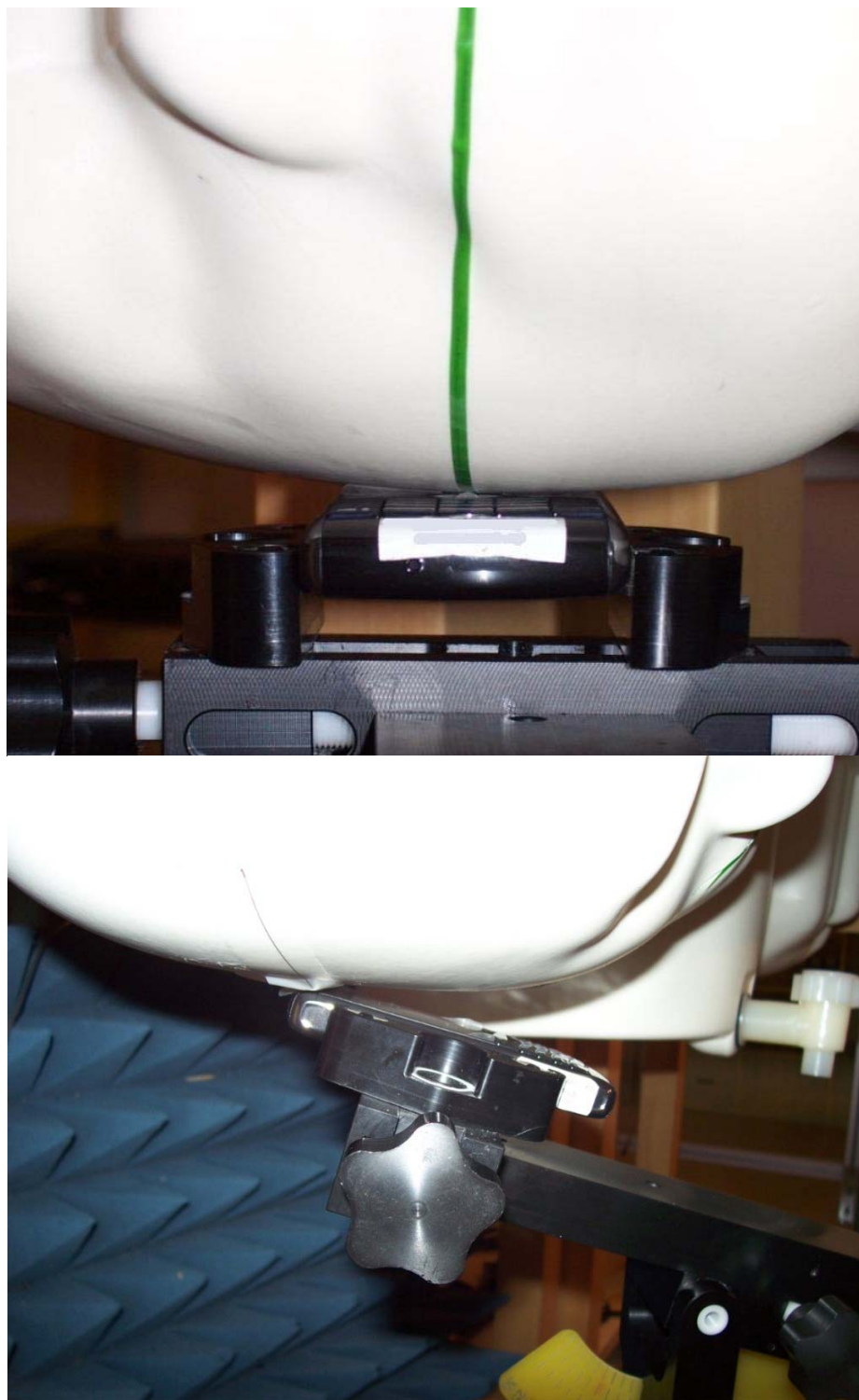
Figure E3. Head configuration (Right Touch/Tilt)
