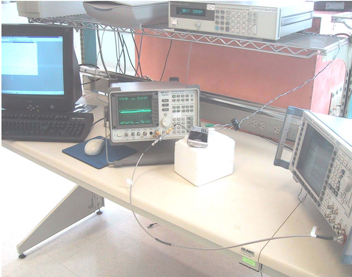
Conducted RF Emission Test Set-up
