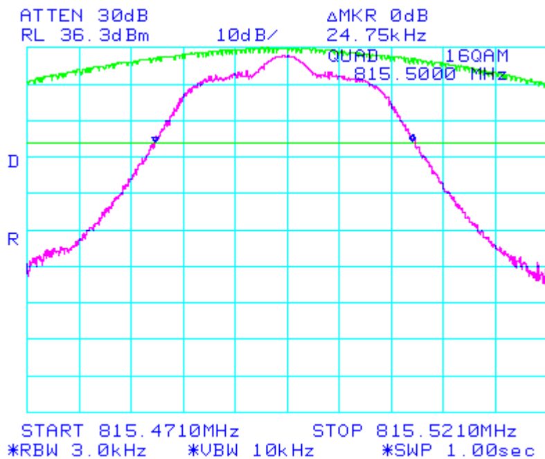
Figure 14: -26 dBc Bandwidth
