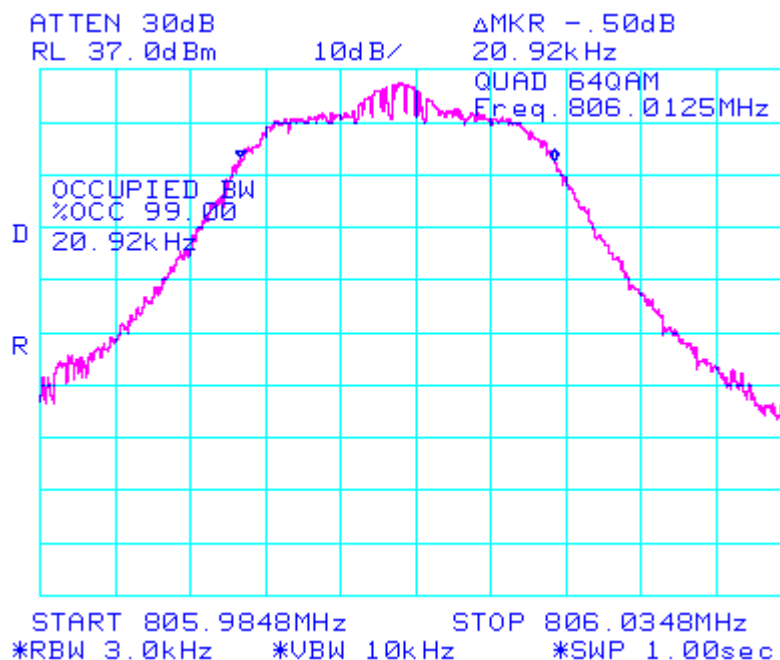
Figure 7: Occupied Bandwidth (99%)
