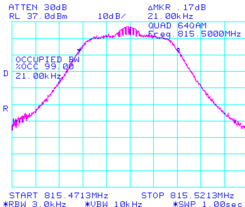
Figure 8: Occupied Bandwidth (99%)
