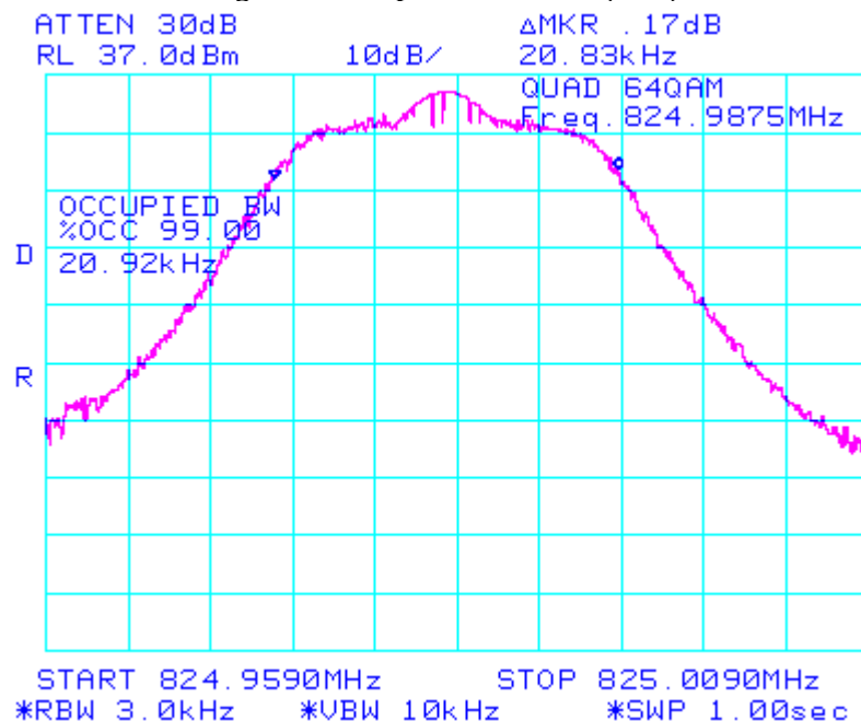
Figure 9: Occupied Bandwidth (99%)
