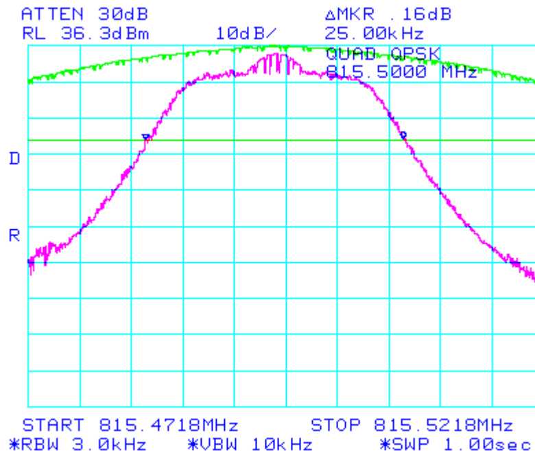
Figure 11: -26 dBc Bandwidth
