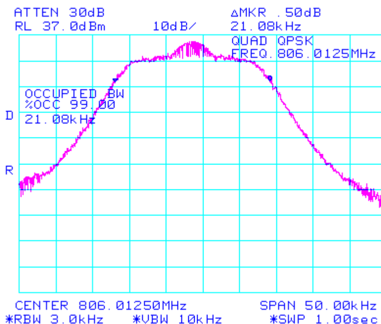
Figure 1: Occupied Bandwidth (99%)
