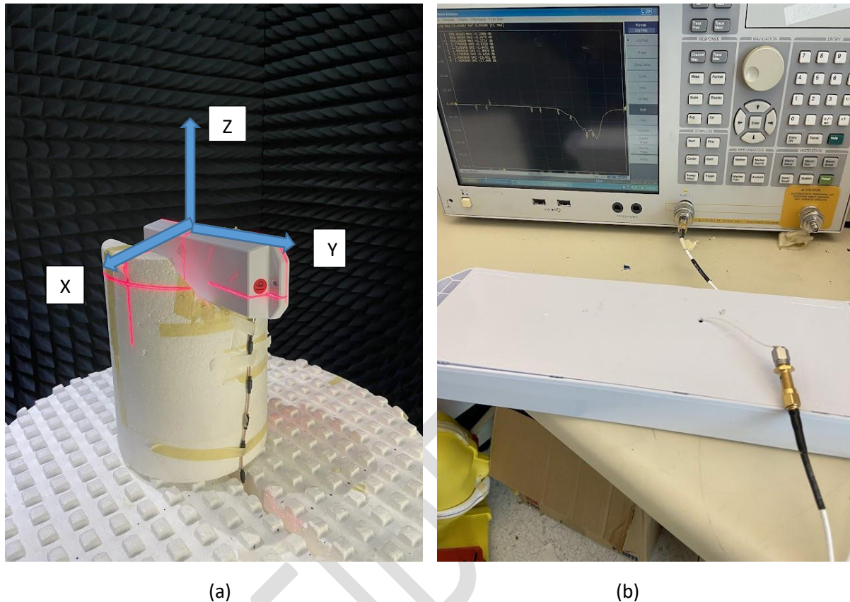
Figure 2. (a) Peak gain, Efficiency and Radiation pattern test setup; (b) Return Loss test setup
