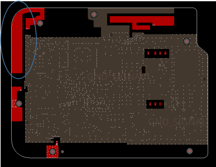
Figure 1. B015 PCB Antenna PCB-63693-003
