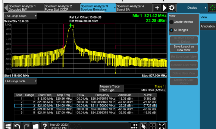
1RB#0 CH 26775 (822.5 MHz)
