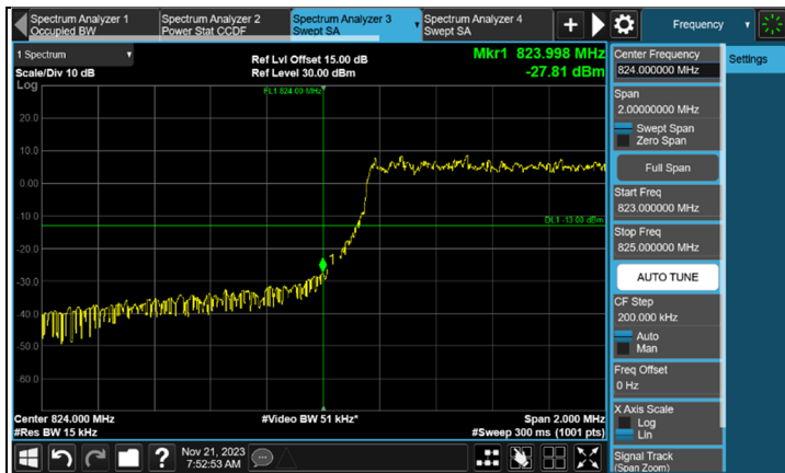
FULL CH 20407 (824.7 MHz)
