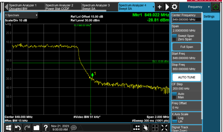
FULL CH 20643 (848.3 MHz)
