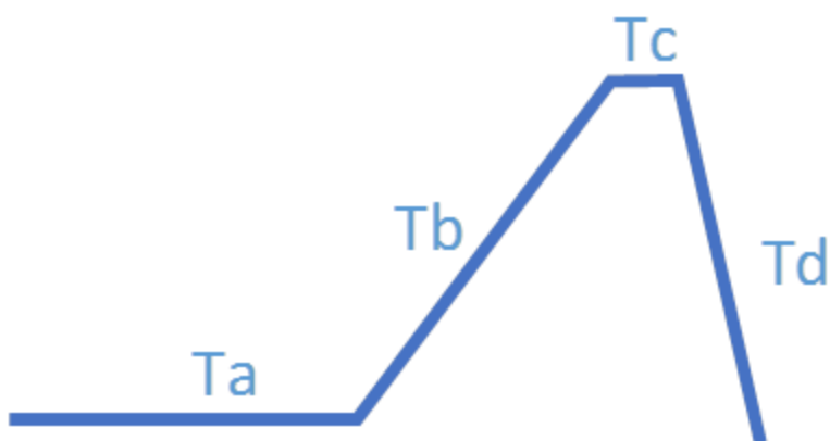
Figure 2-1 – Chirp Profile
