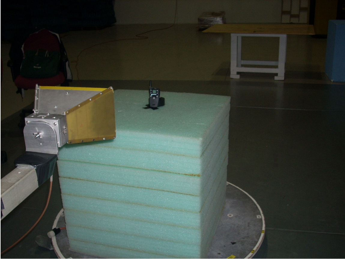
Radiated Measurements Above 1GHz
