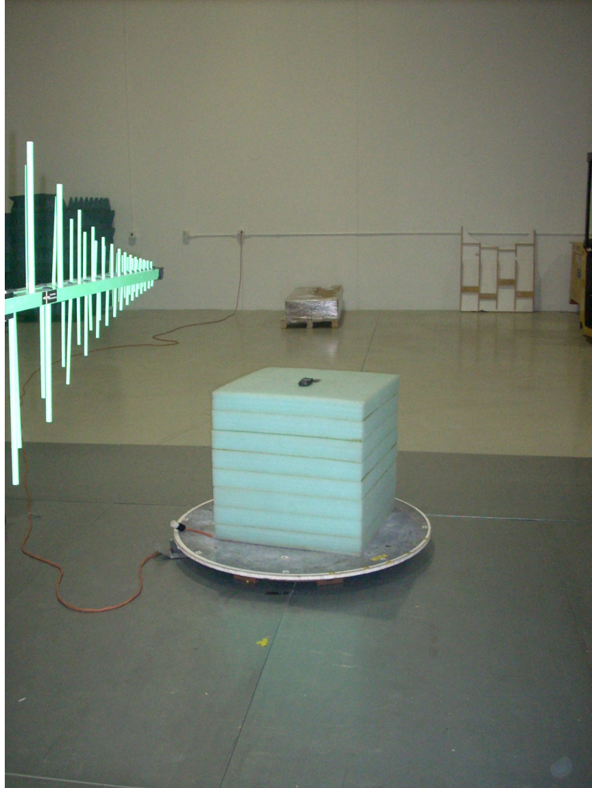
Radiated Measurements Below 1GHz
