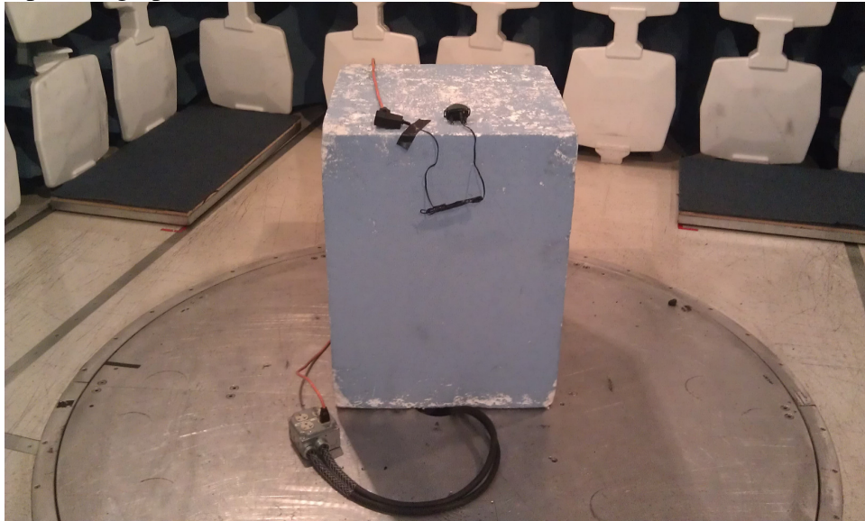
Verification Radiated Emissions Measurements – Anechoic Chamber
