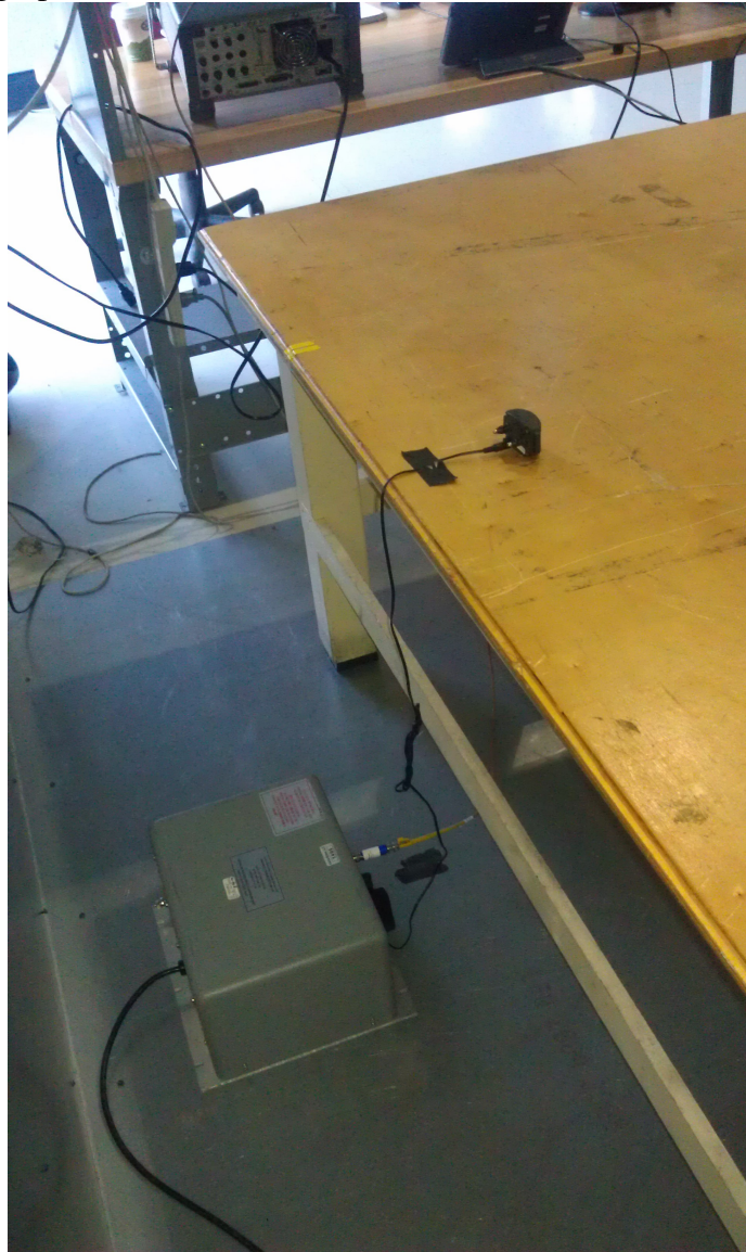
AC Line Conducted Emissions – Rear
