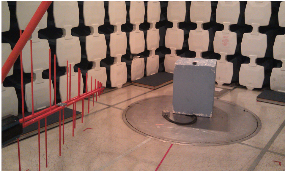
Radiated Emissions Measurements – Below 1GHz – Anechoic Chamber
