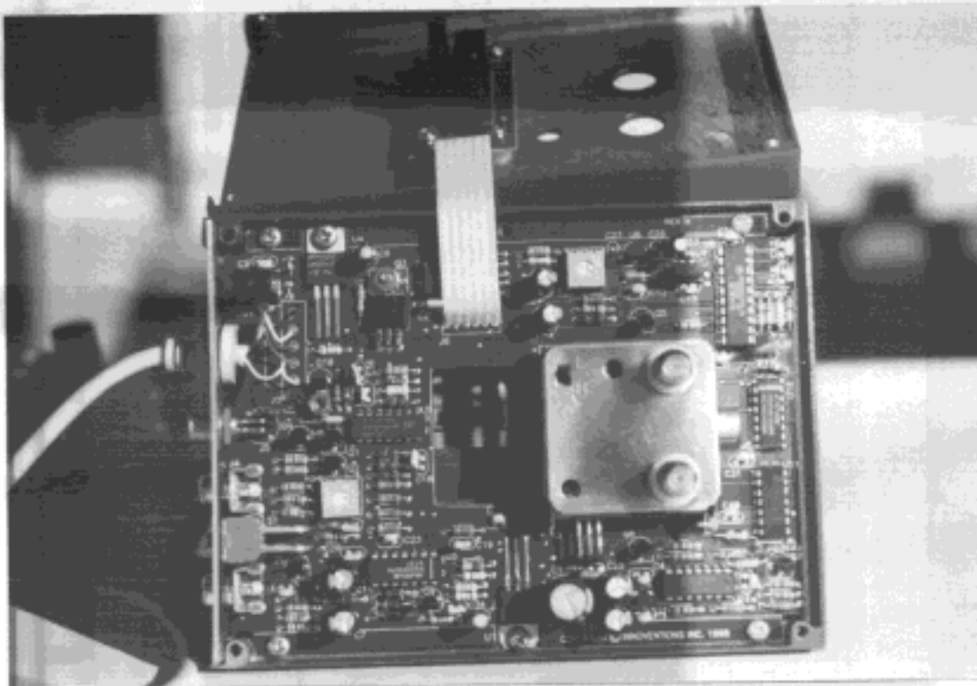
UUT - MAGNI-CAM Interface Box, Top Cover Removed Shows Interface PWB - Component Side
