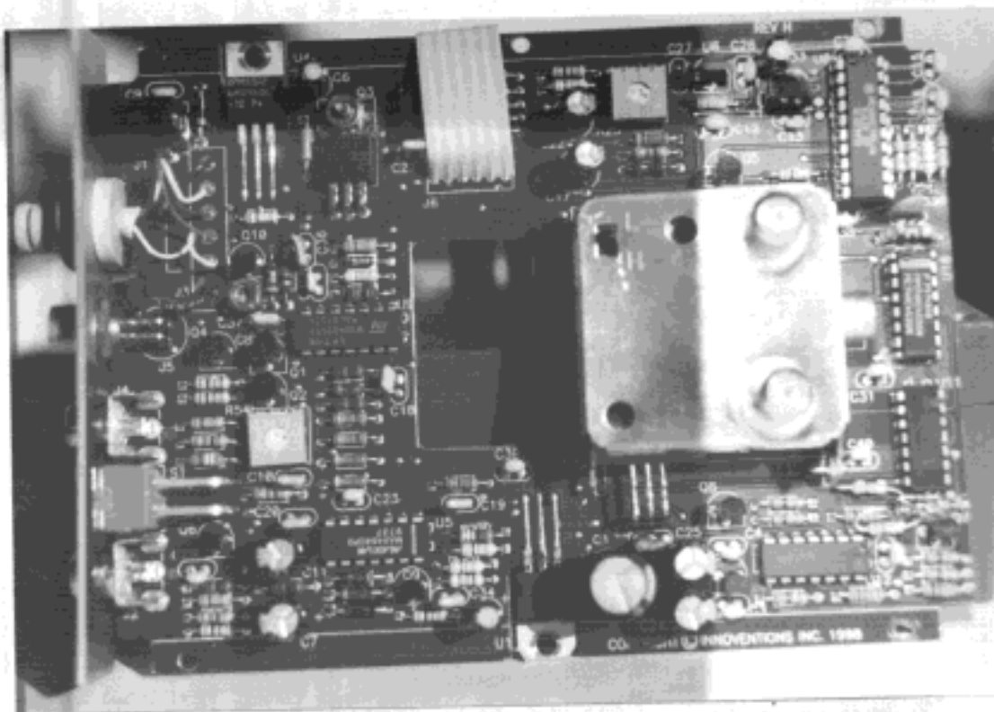
Interface PWB Close-up Component Side showing UUT Sharp E7853 VHF RF Modulator
