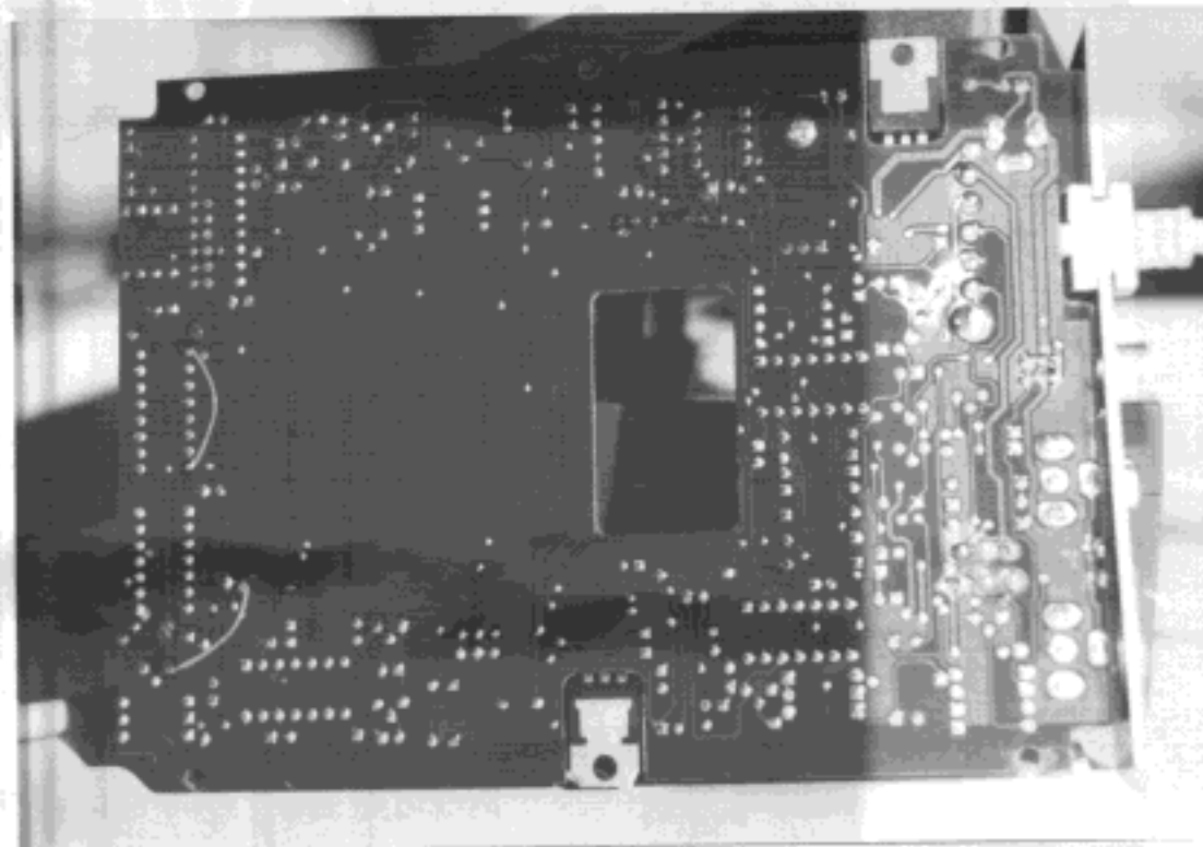
UUT MAGNI-CAM Interface PWB - Foil Side
