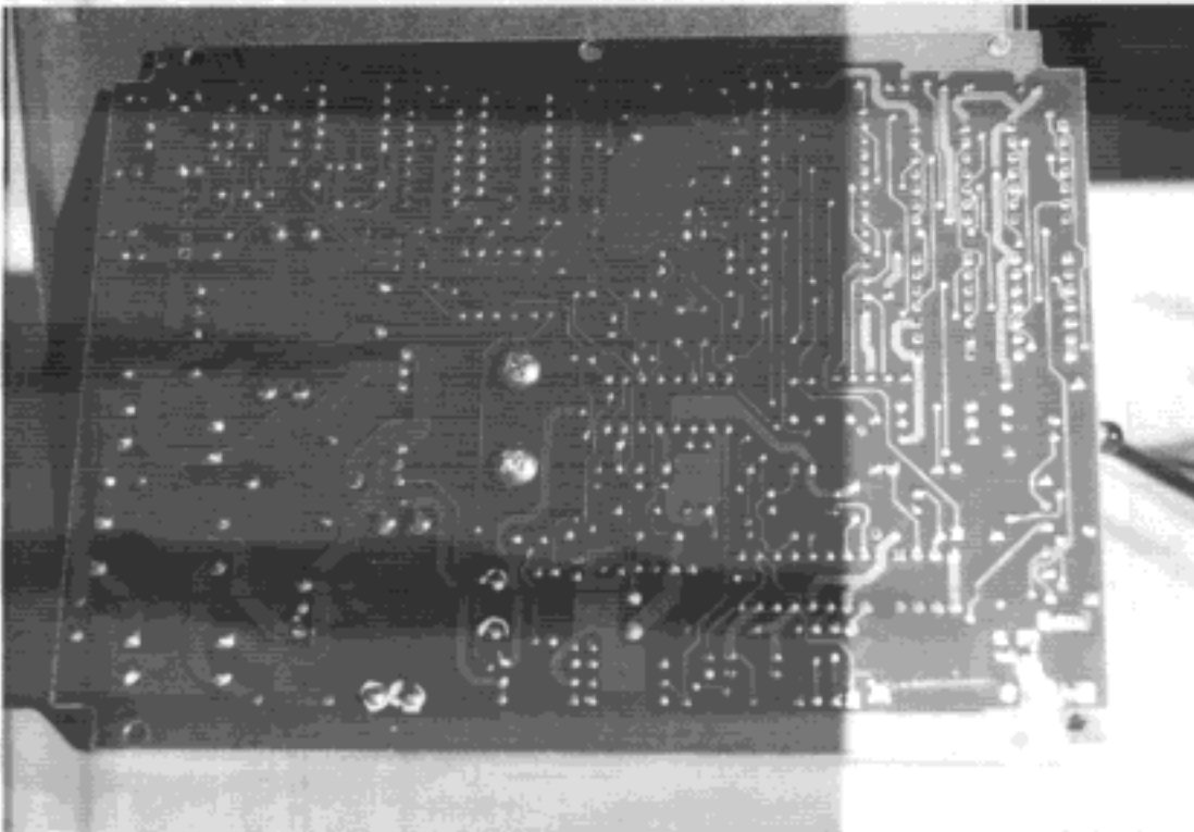
Battery Charger PWB - Foil Side
