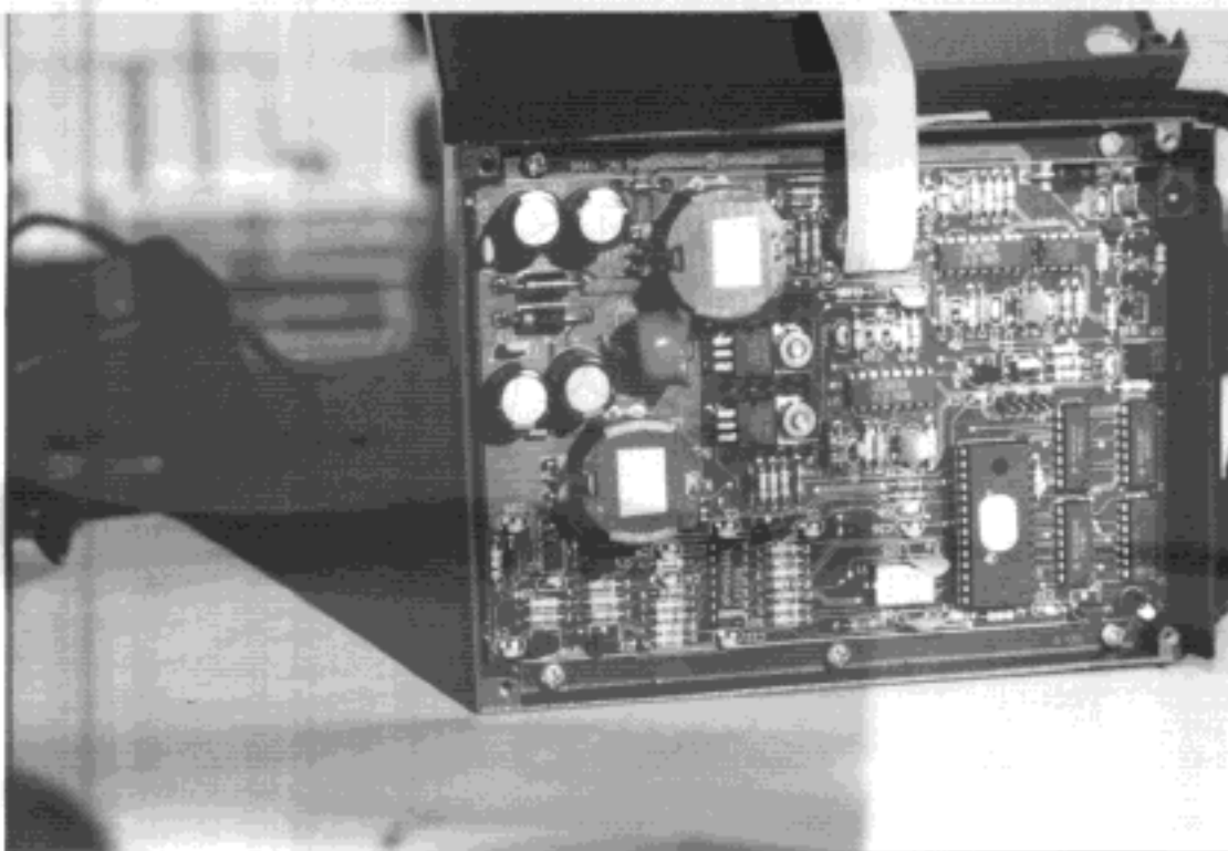
Battery Charger PWB - Component Side
