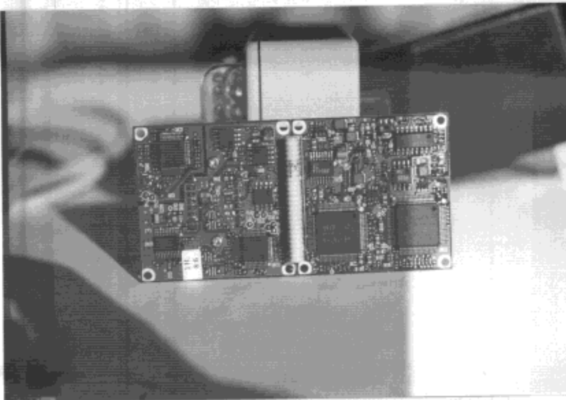
Camera PWB - Foil/Component Bottom Side
