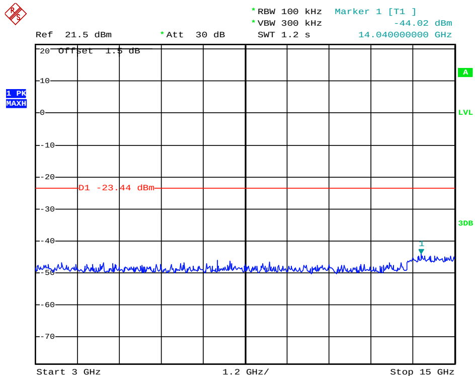
(Plot 4.9.2.C1: Channel 78: 2480MHz @ 8DPSK)
