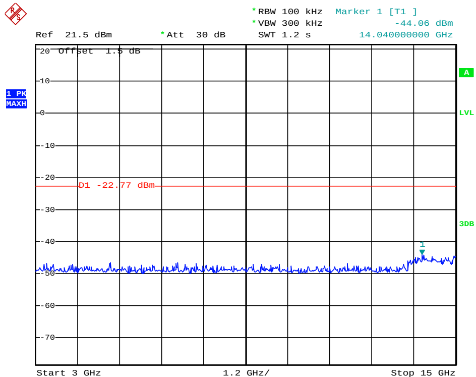
(Plot 4.9.2.A1: Channel 00: 2402MHz @ 8DPSK)
