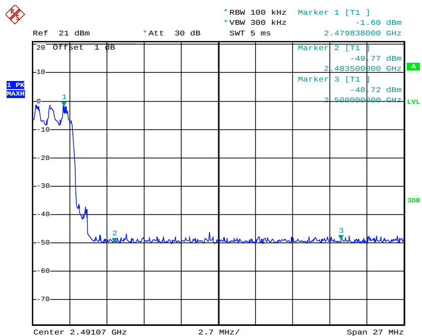
(Plot 4.5.2.3 C: Channel 78: 2480MHz @ \pi/4 DQPSK)
