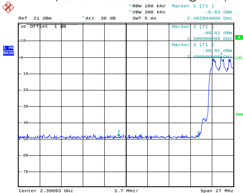
(Plot 4.5.2.2 A: Channel 00: 2402MHz @ 8DPSK)
