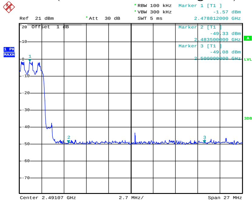
(Plot 4.5.2.2 C: Channel 78: 2480MHz @ 8DPSK)
