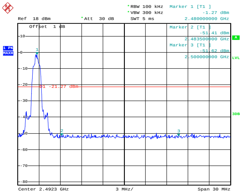
(Plot 4.5.2.2 B: Hopping Mode @ 8DPSK)
