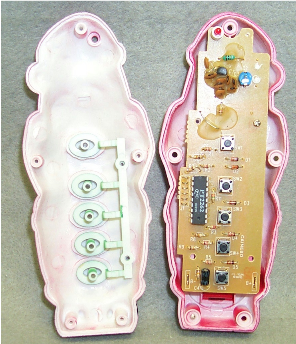
Photo 3. EUT, Cover Opened
