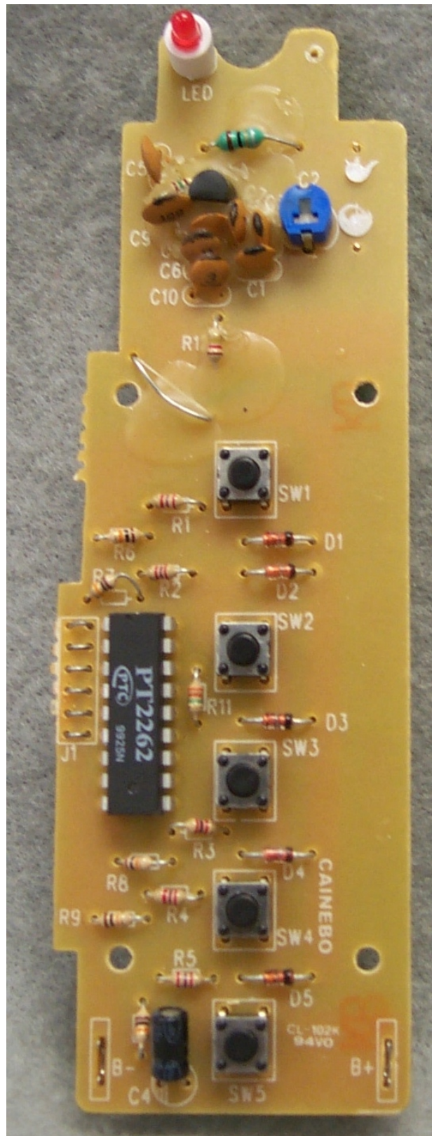
Photo 4. Internal View, Top Side
