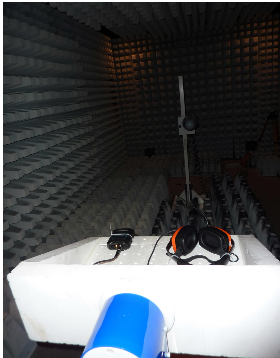
170685Setup06: Final 1 – 13 GHz FAR
