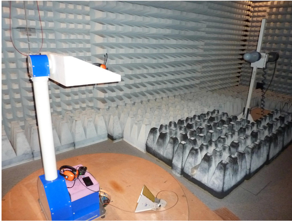
170685Setup05: Final 1 – 13 GHz FAR
