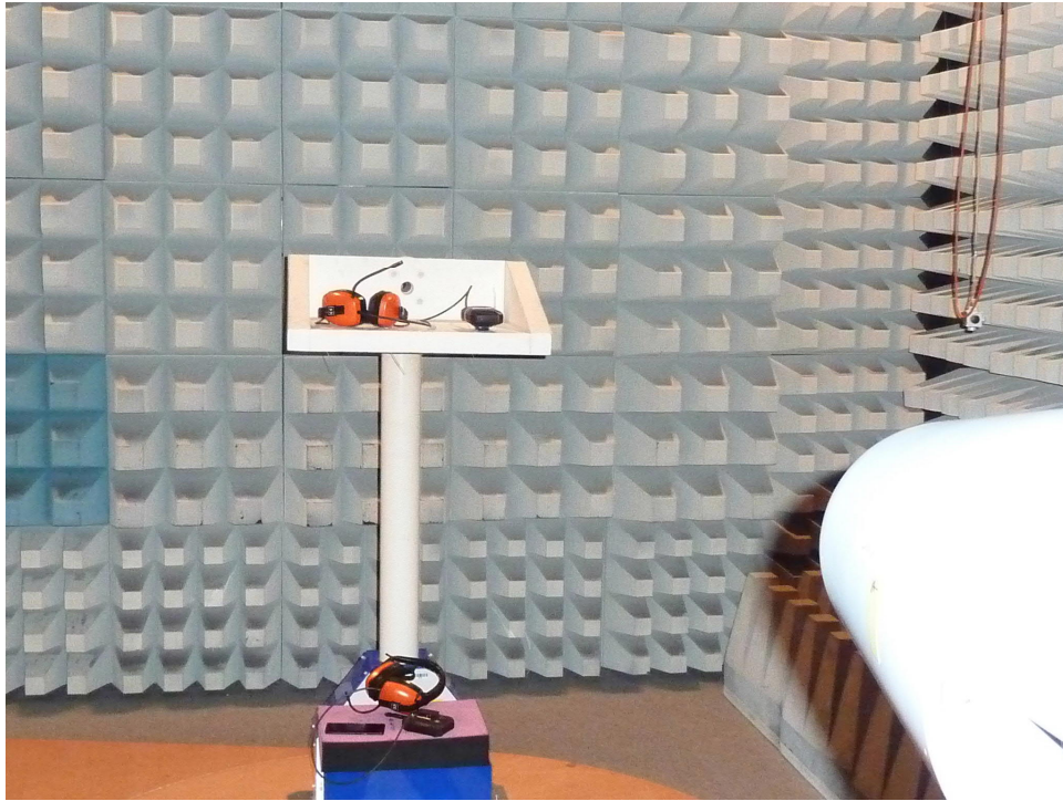
170685Setup09: Final 1 – 13 GHz FAR
