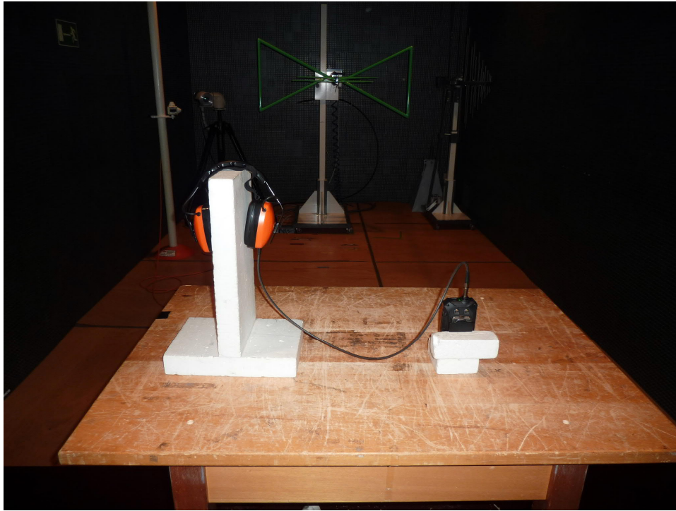
170685Setup01: Preliminary 30 – 1000 MHz FAR
