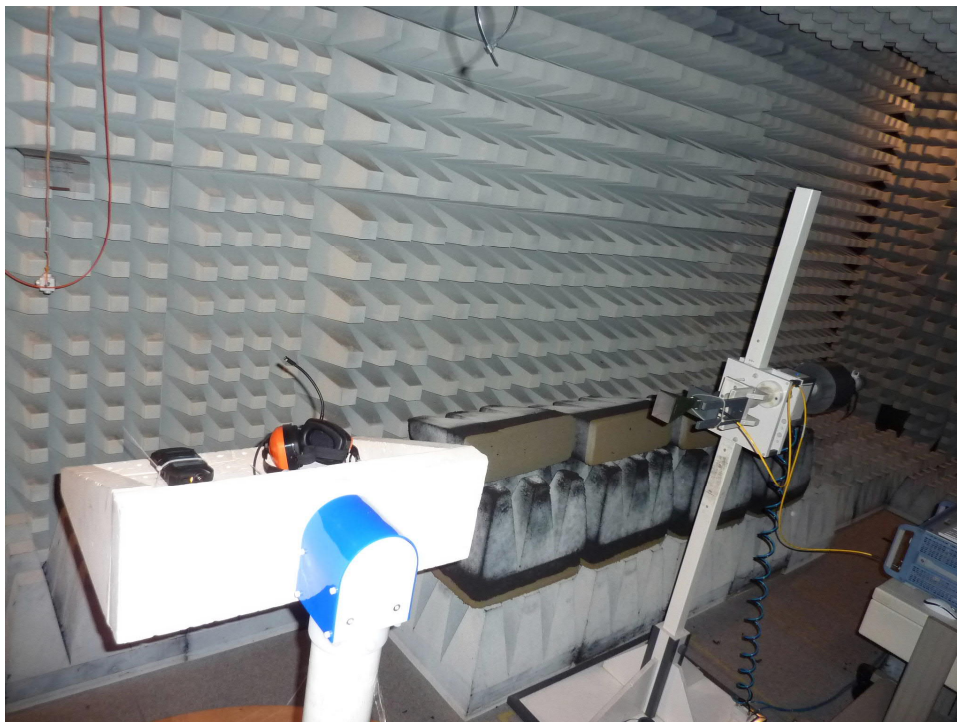
170685Setup15: Final 18 – 25 GHz FAR
