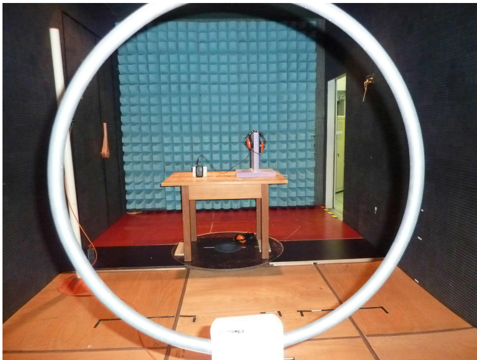
170685Setup17: Preliminary 9 kHz – 30 MHz FAR
