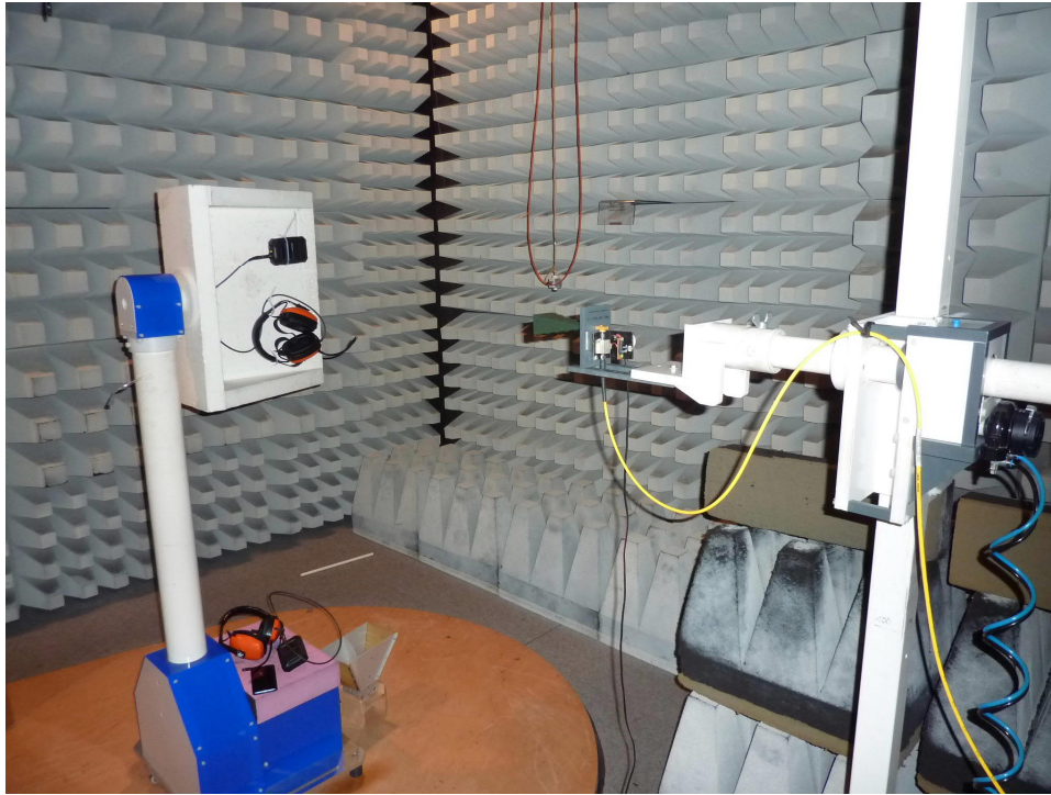
170685Setup13: Final 18 – 25 GHz FAR
