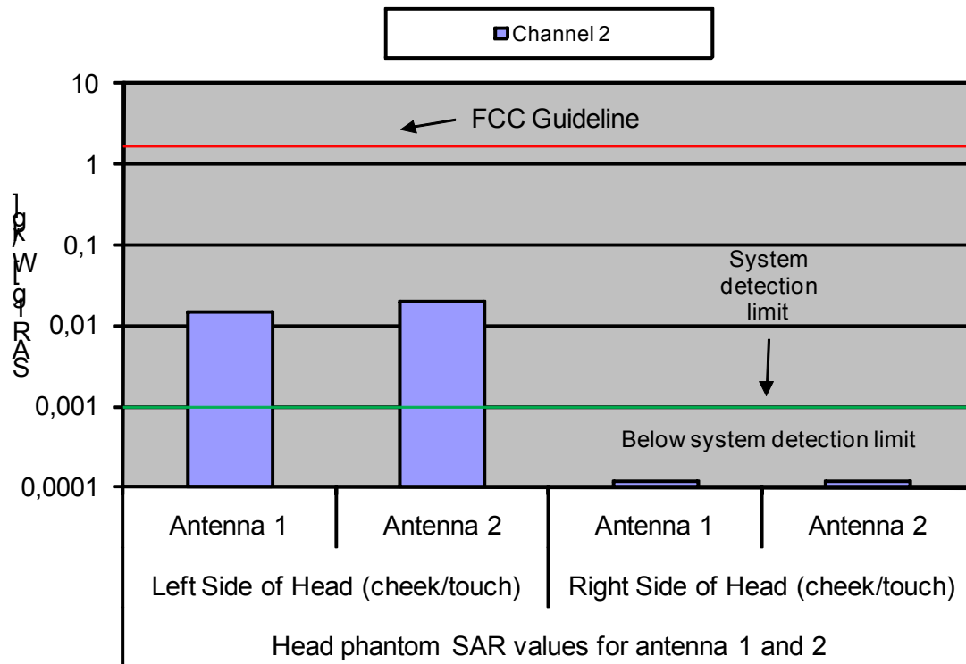
Fig. 8: The measured SAR values for the CeoTronics CT-GateCom II for the US DECT standard in comparison to the FCC exposure limit.
