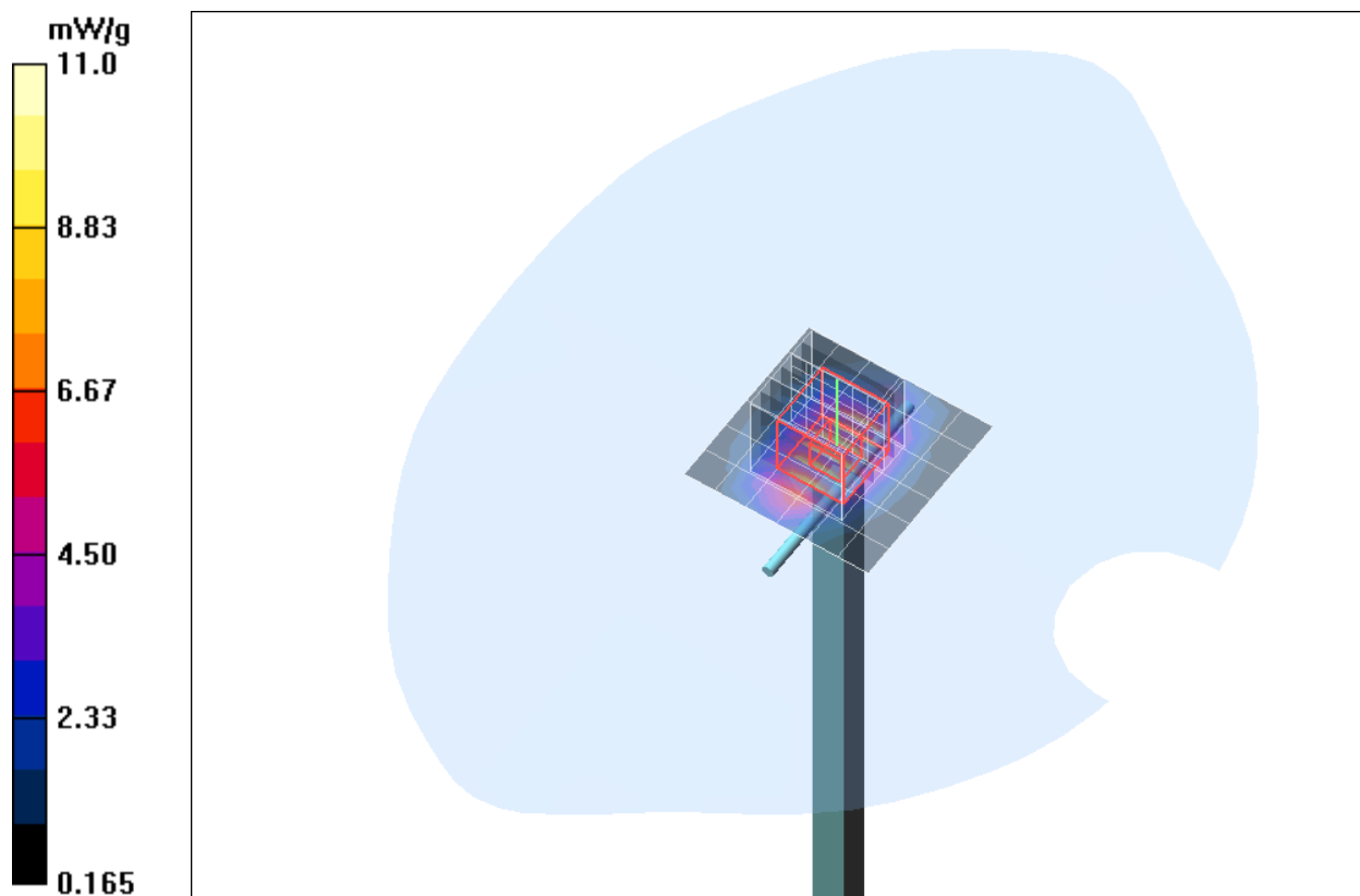
Fig. 9: Validation measurement 1900 MHz Head (May 19, 2011), coarse grid. Ambient Temperature: 21.5° C, Liquid Temperature: 21.3° C.
