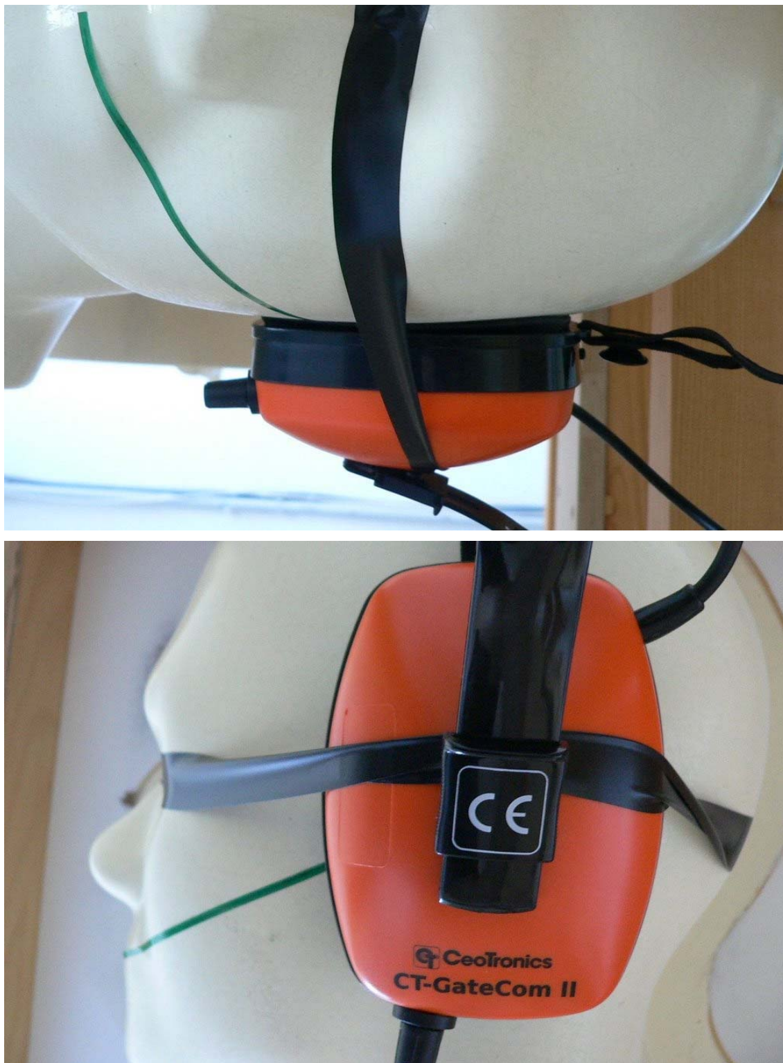
Fig. 13: Cheek position, left side (left earpiece).
