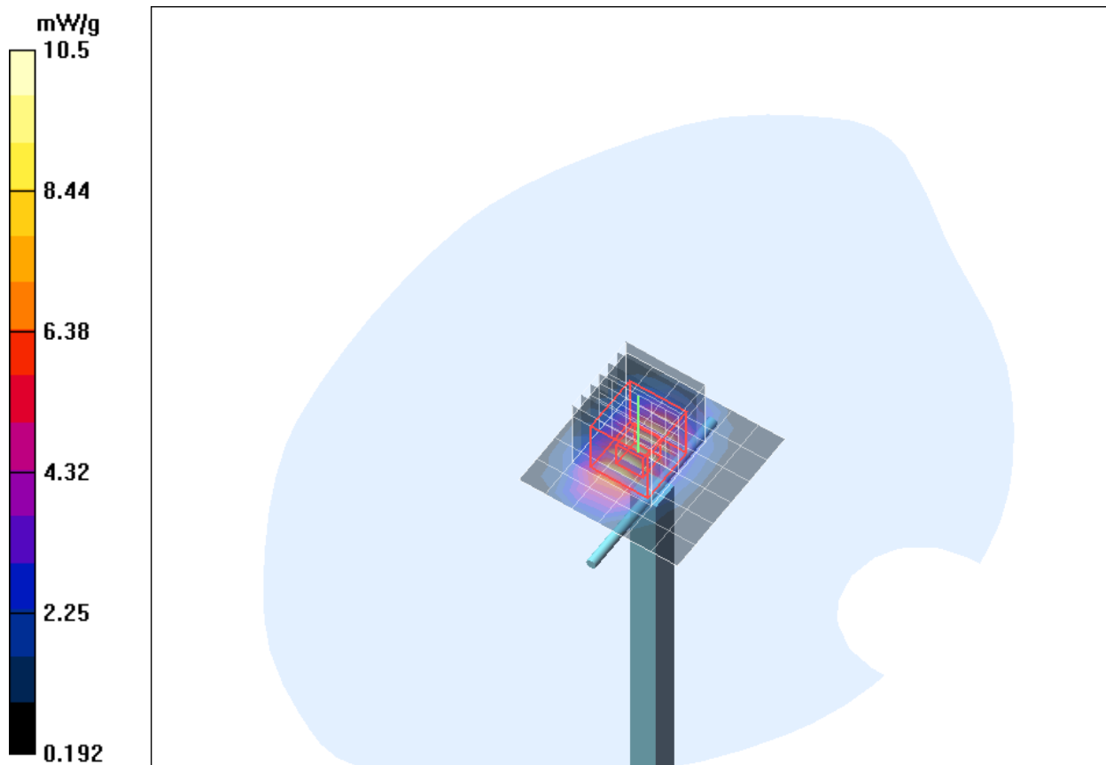
Fig. 9: Validation measurement 1900 MHz body (February 28, 2011), coarse grid. Ambient Temperature: 22.1° C, Liquid Temperature: 21.7° C.
