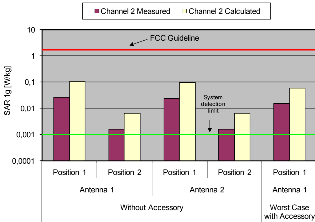
Fig. 8: The measured body phantom SAR values for the CeoTronics CT-DECT GateCom Compact for the US DECT standard in comparison to the FCC exposure limit.
