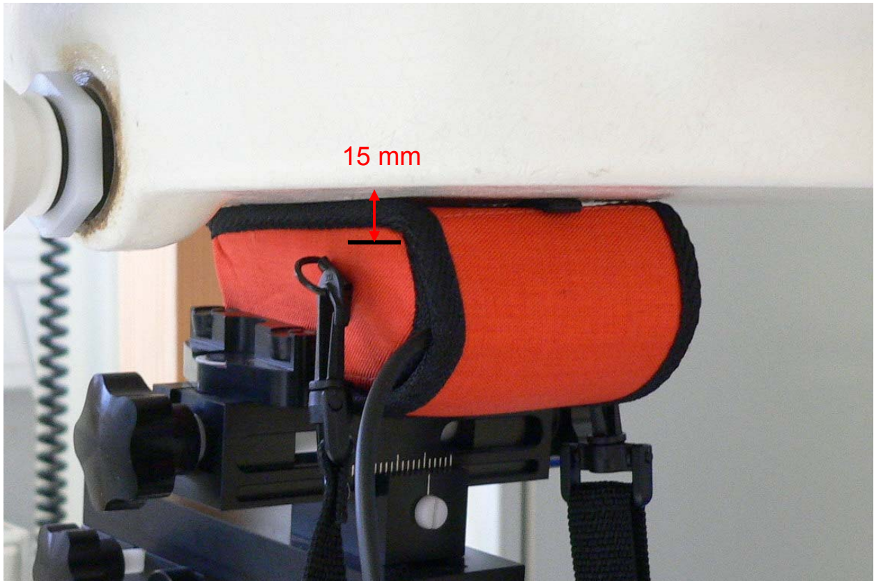
Fig. 16: Body worn, position 2, with used case.
