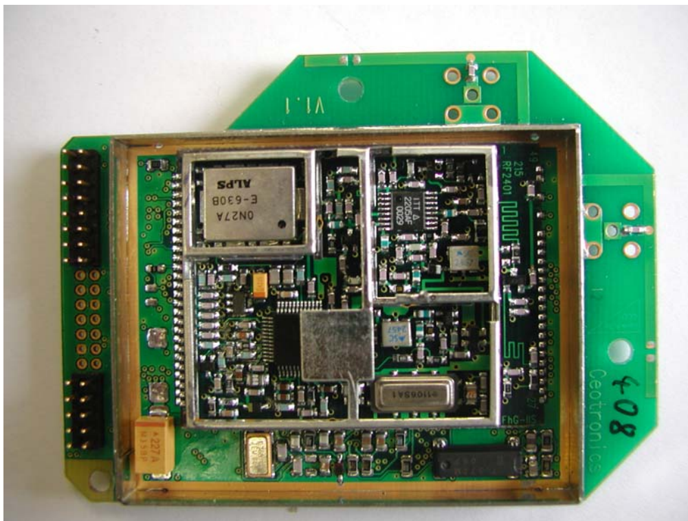
Photo 2: CT-DECT-H24 / Top View Without RF Screening Plate
