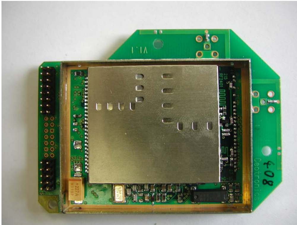
Photo 1: CT-DECT-H24 Headset / Top View Without Screening Plate
