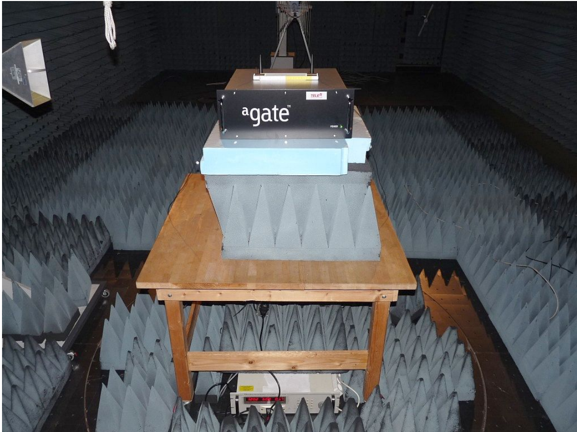
Photo 1: Setup for radiated tests
