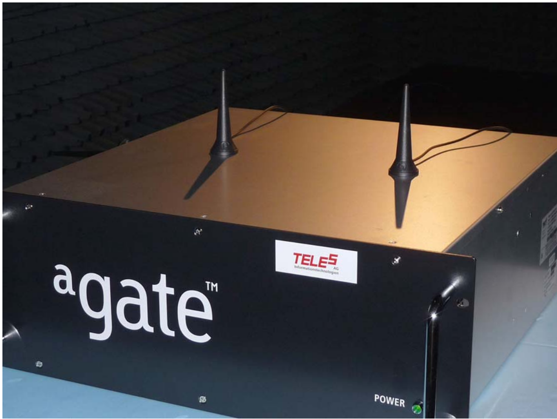
Photo 3: Assembly of both antennas on top of the housing
