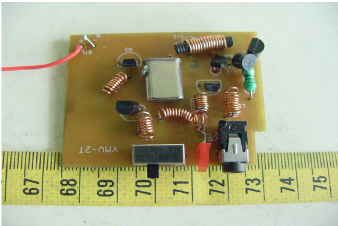
Component View of Microphone PCB
