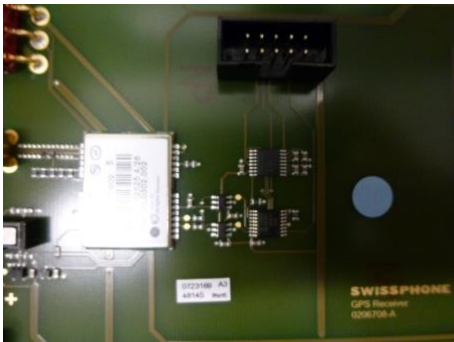
Photo 17: GPS module
