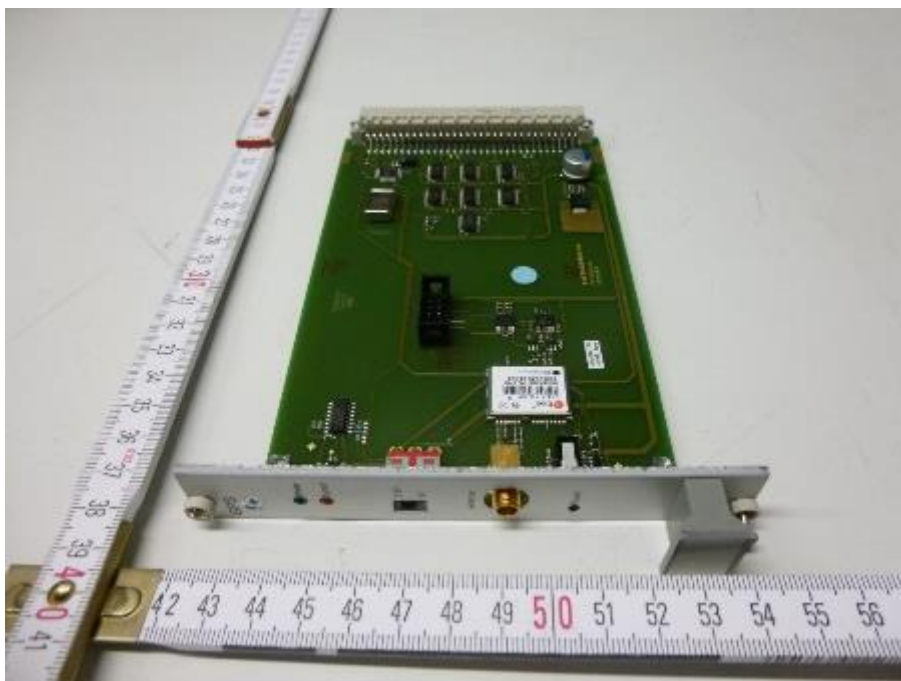
Photo 15: GPS module
