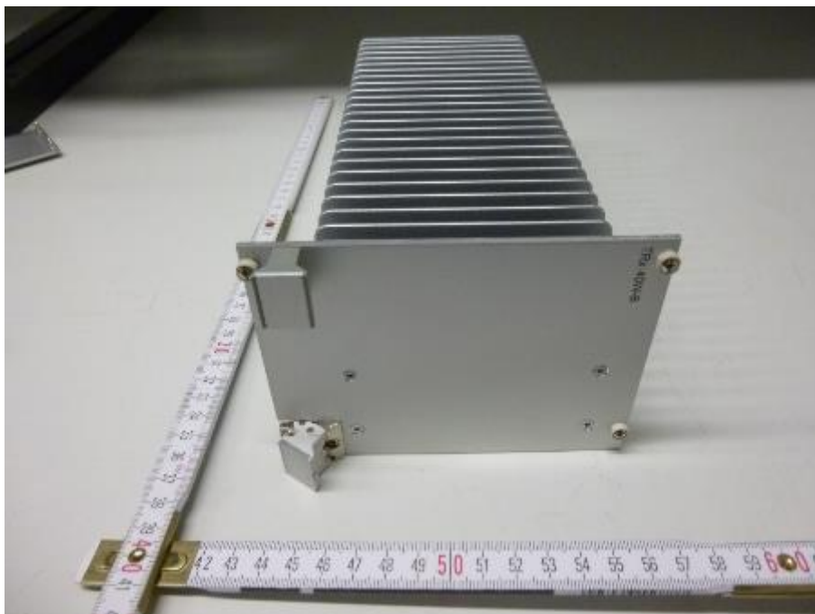
Photo 32: RF module
