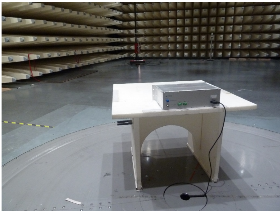
Photo 6: Measurements semi anechoic chamber
