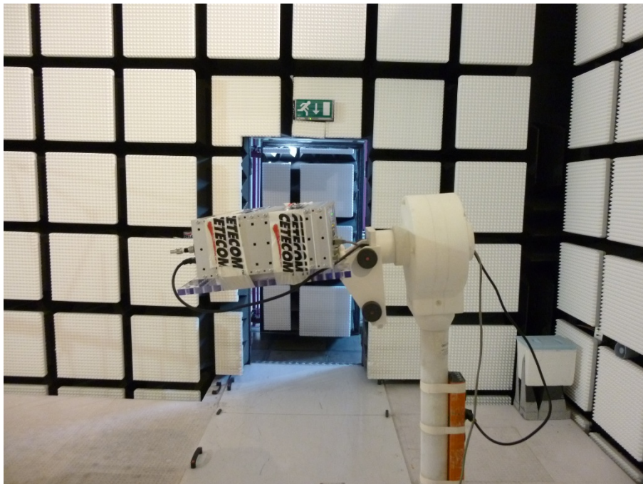
Photo 5: Measurements fully anechoic chamber
