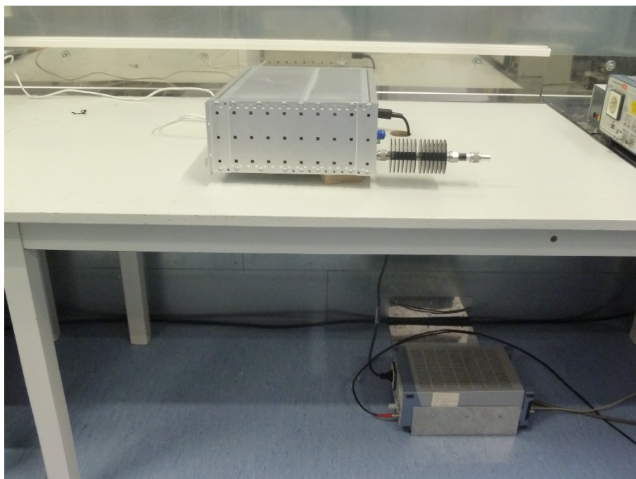
Photo 7: AC-conducted measurements
