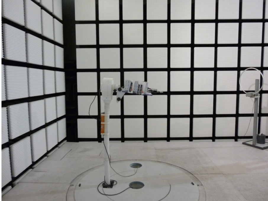
Photo 1: Measurements fully anechoic chamber
