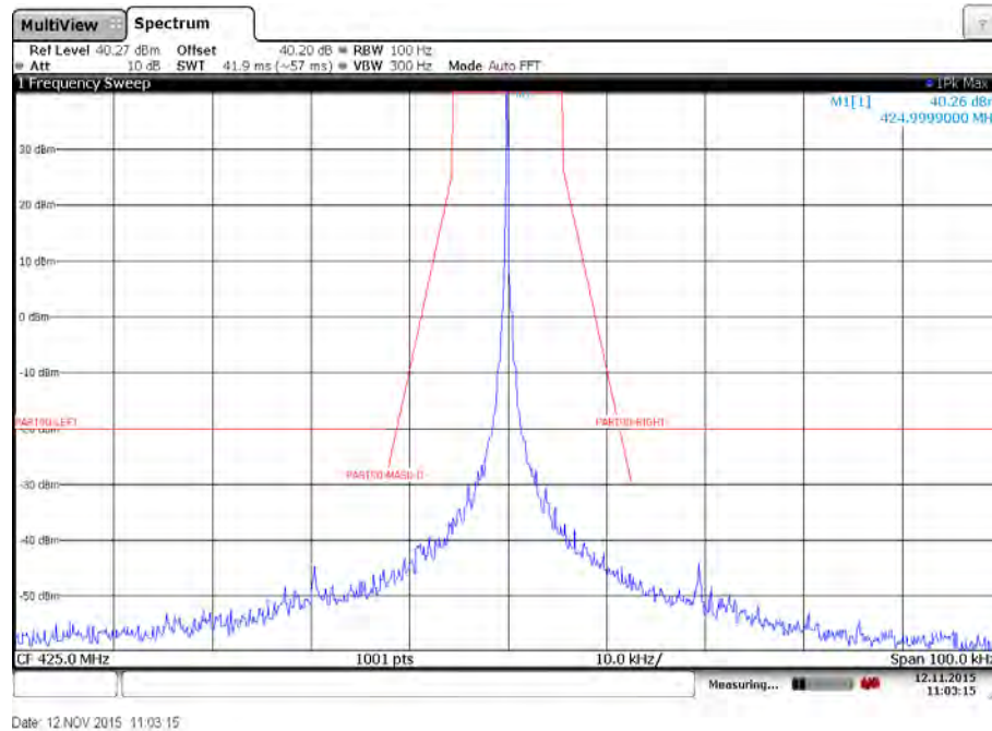
Plot 9: Emission mask D – Mid channel – 512 bits per second – Low power – Carrier unmodulated
