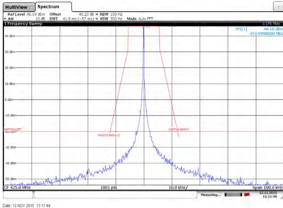
Plot 39: Emission mask D – Mid channel – 4800 bits per second – High power – Carrier unmodulated
