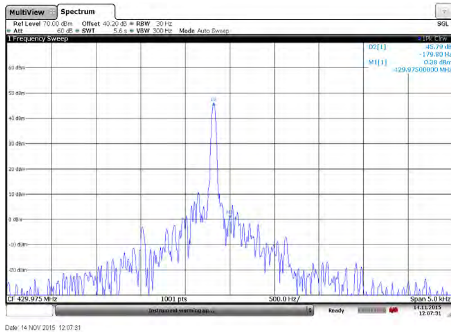
Plot 28: High channel – Temperature: 50°C
