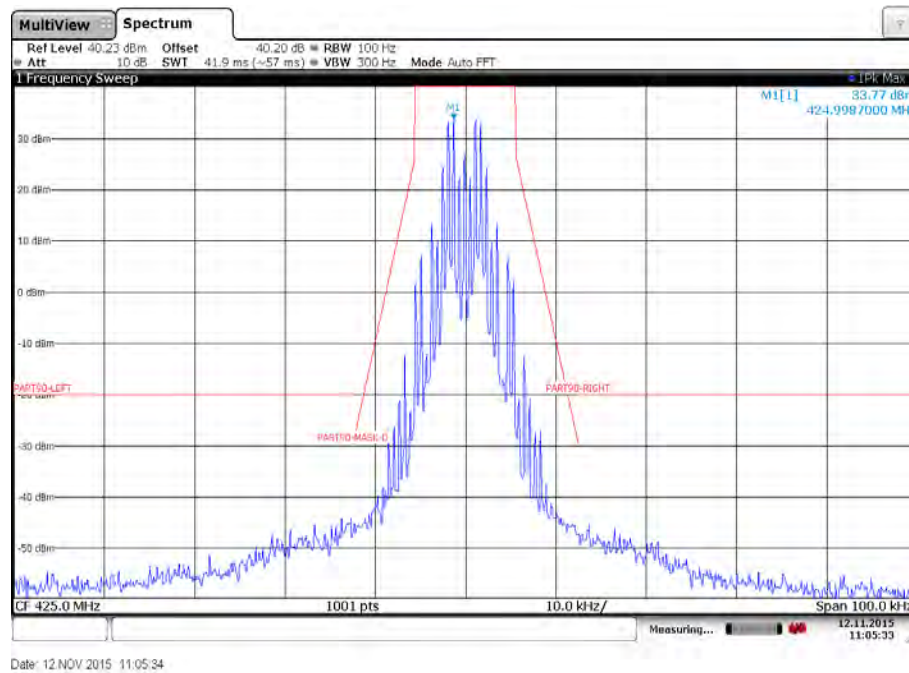
Plot 12: Emission mask D – Mid channel – 1200 bits per second – Low power – Carrier modulated
