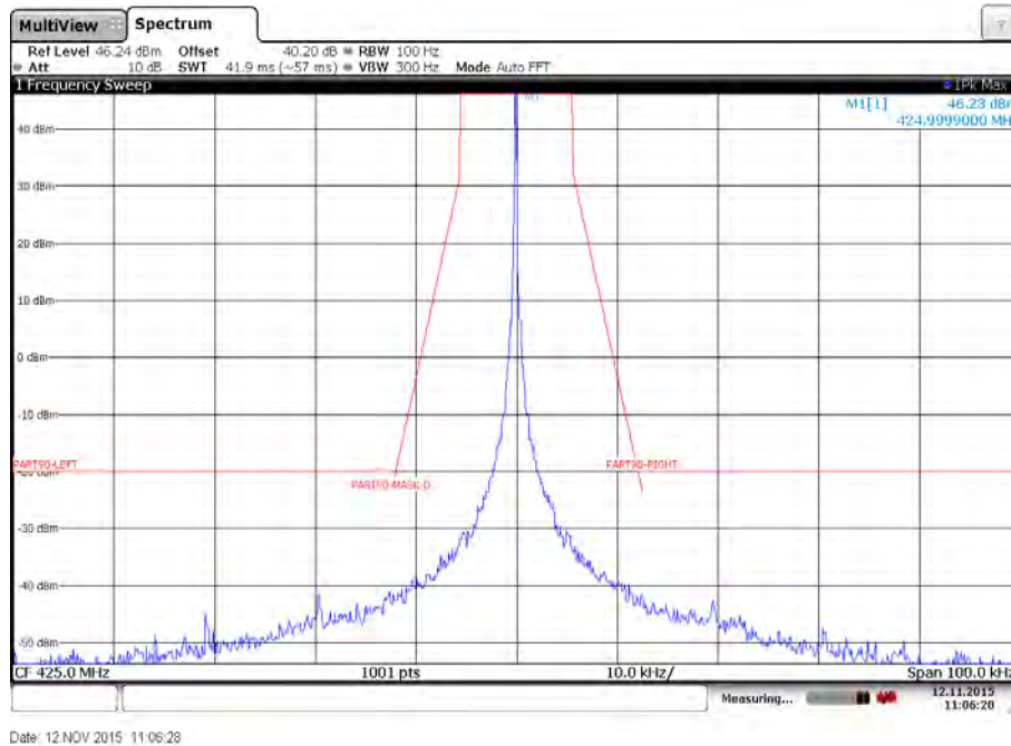
Plot 35: Emission mask D – Mid channel – 1200 bits per second – High power – Carrier unmodulated
