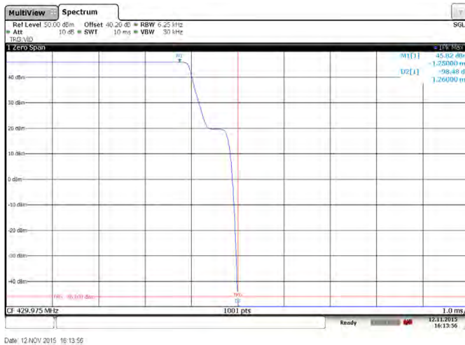
Plot 12: Highest channel – Switch off (zoomed)
