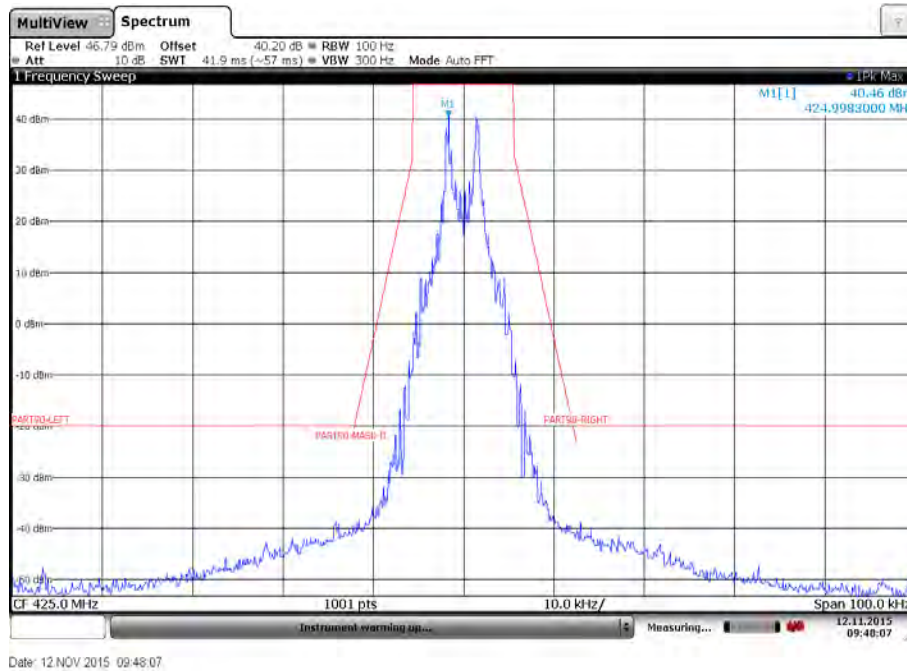
Plot 34: Emission mask D – Mid channel – 512 bits per second – High power – Carrier modulated
