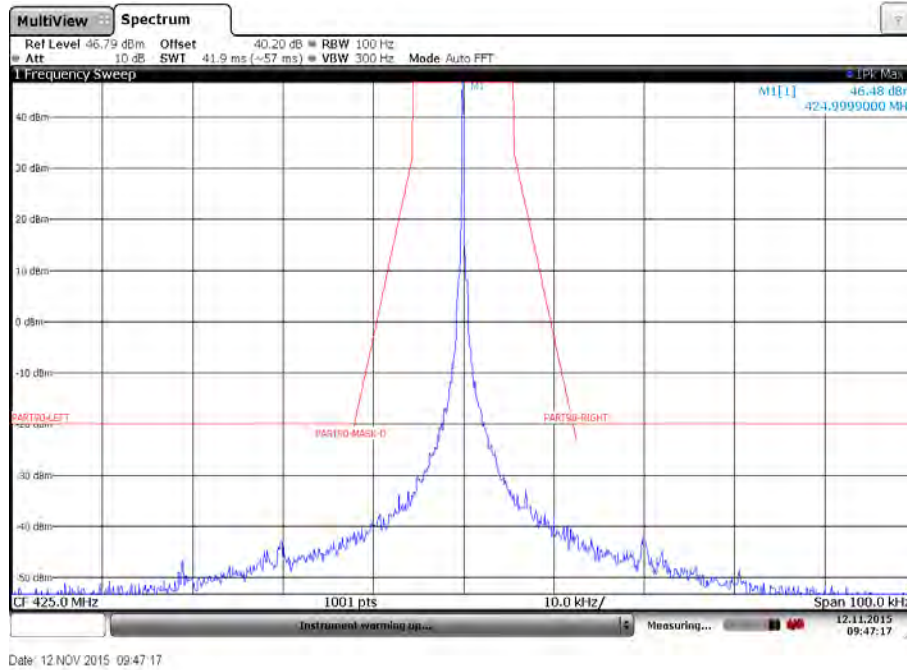
Plot 33: Emission mask D – Mid channel – 512 bits per second – High power – Carrier unmodulated
