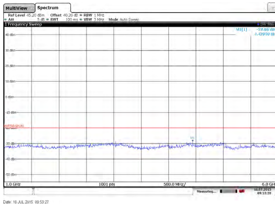
Plot 2: Low channel – Low power – 1 GHz to 6 GHz
