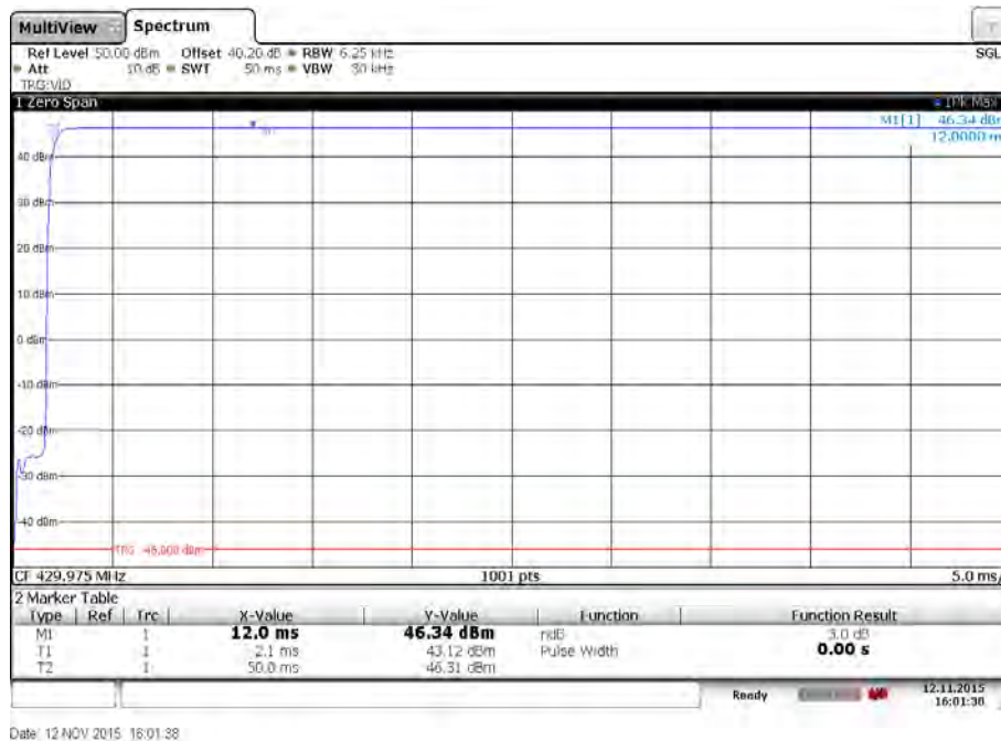
Plot 10: Highest channel – Switch on (zoomed)
