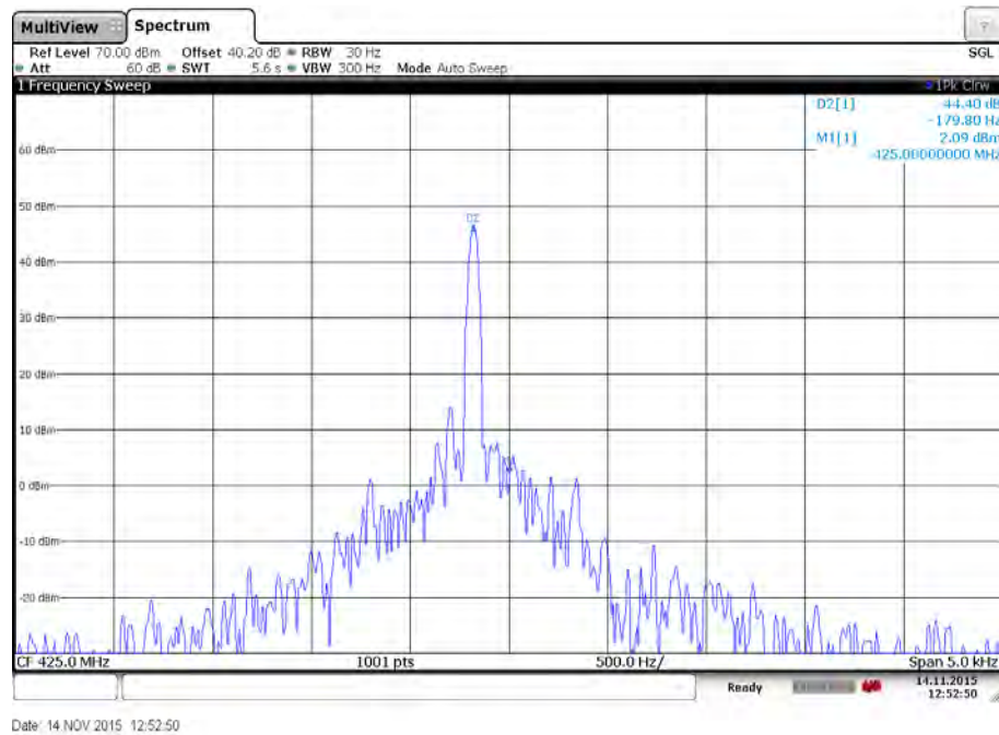
Plot 16: Middle channel – Temperature: 30°C
