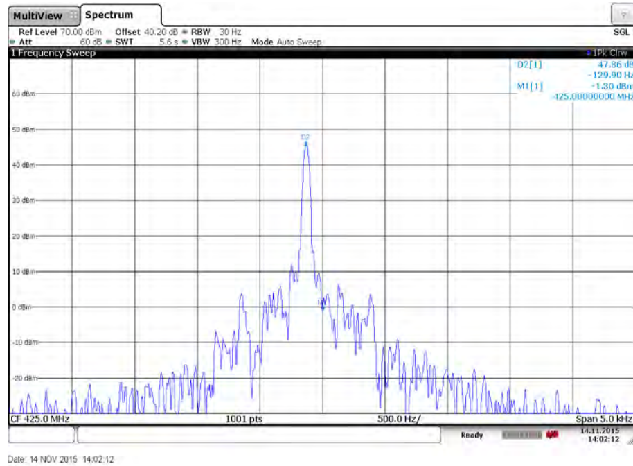
Plot 13: Middle channel – Temperature: 0°C
