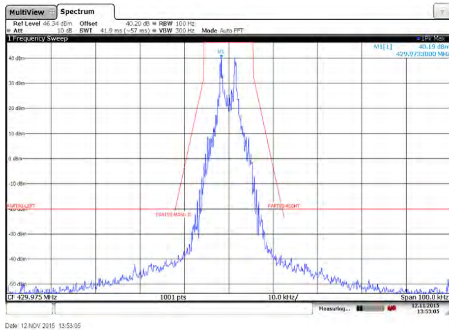
Plot 42: Emission mask D – High channel – 512 bits per second – High power – Carrier modulated
