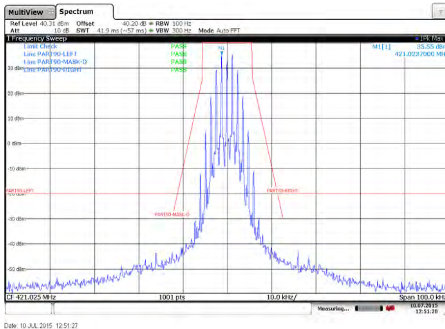
Plot 6: Emission mask D – Low channel – 2400 bits per second – Low power – Carrier modulated
