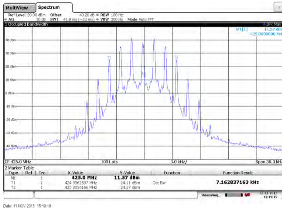
Plot 8: Middle channel / 2400 b bits is per second
