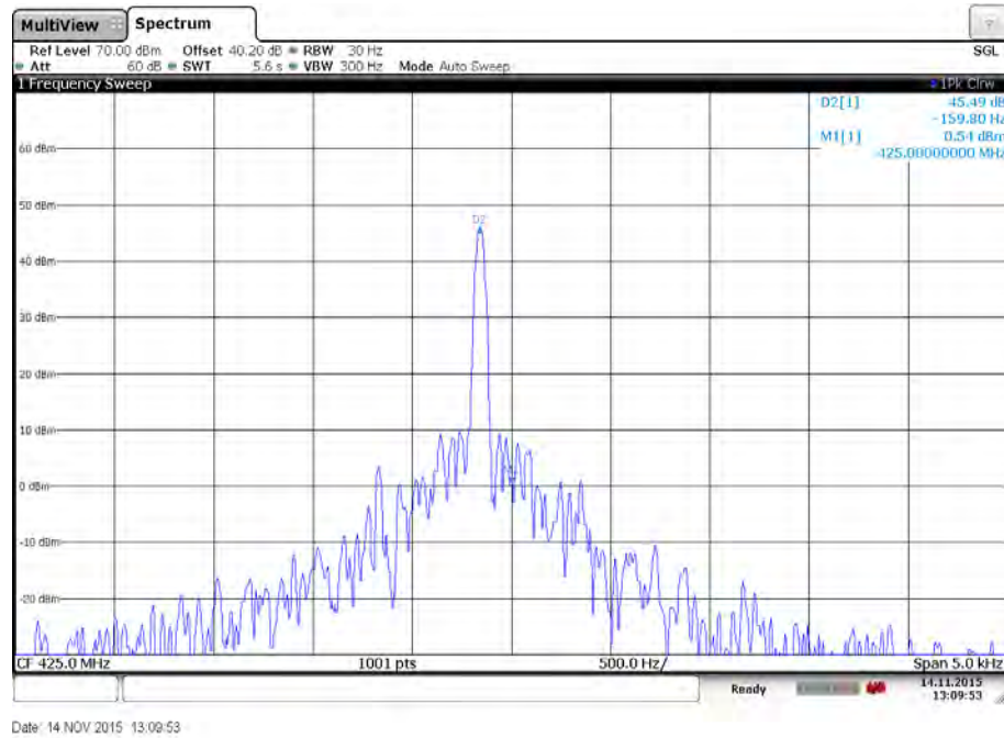
Plot 15: Middle channel – Temperature: 20°C
