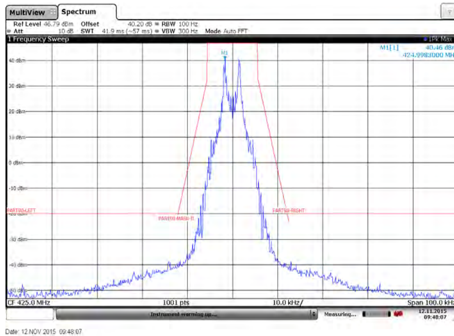
Plot 10: Emission mask D – Mid channel – 512 bits per second – Low power – Carrier modulated
