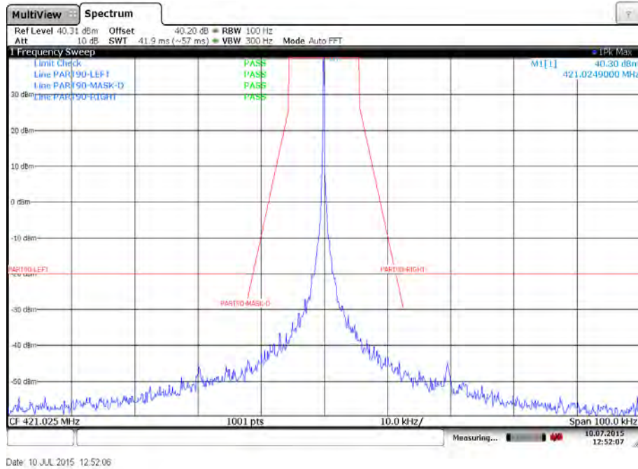
Plot 7: Emission mask D – Low channel – 4800 bits per second – Low power – Carrier unmodulated
