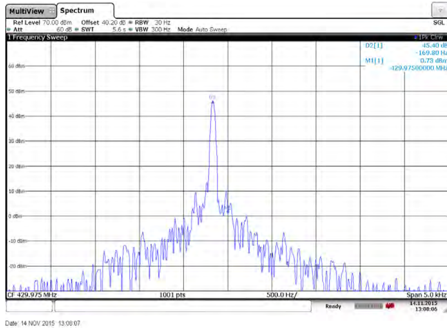
Plot 25: High channel – Temperature: 20°C
