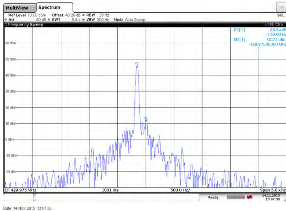
Plot 30: High channel – Temperature: 20°C - 115% Voltage
