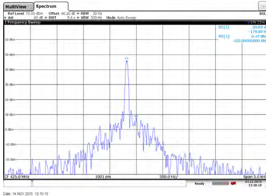
Plot 19: Middle channel – Temperature: 20°C – 85% Voltage
