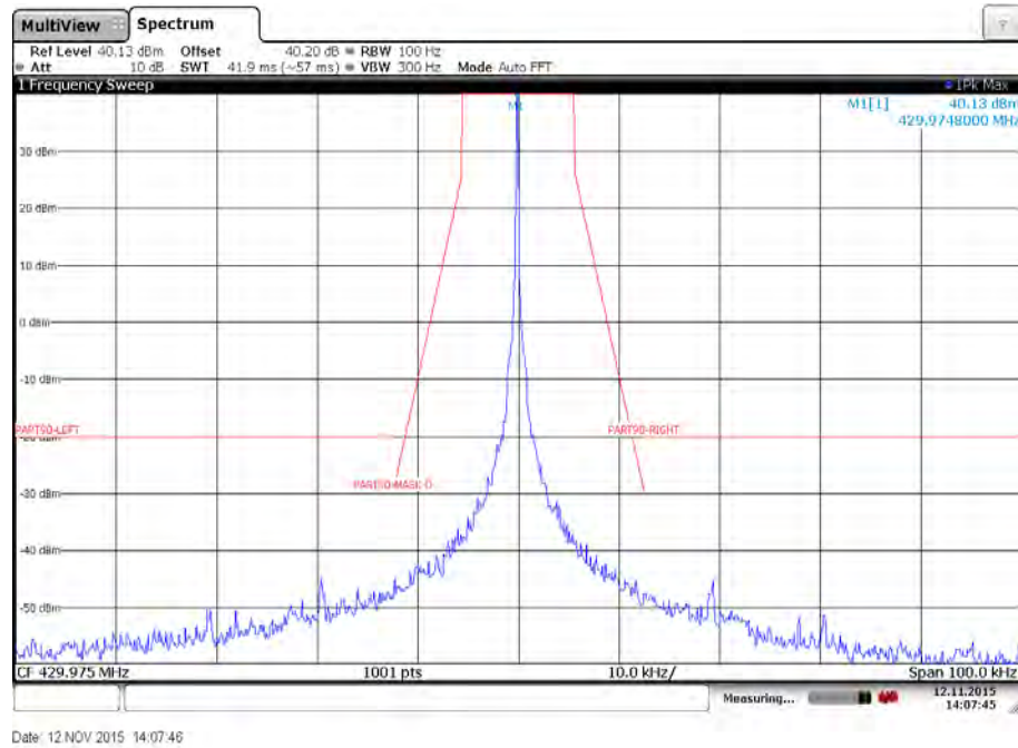
Plot 23: Emission mask D – High channel – 4800 bits per second – Low power – Carrier unmodulated
