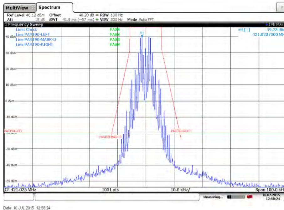
Plot 28: Emission mask D – Low channel – 1200 bits per second – High power – Carrier modulated
