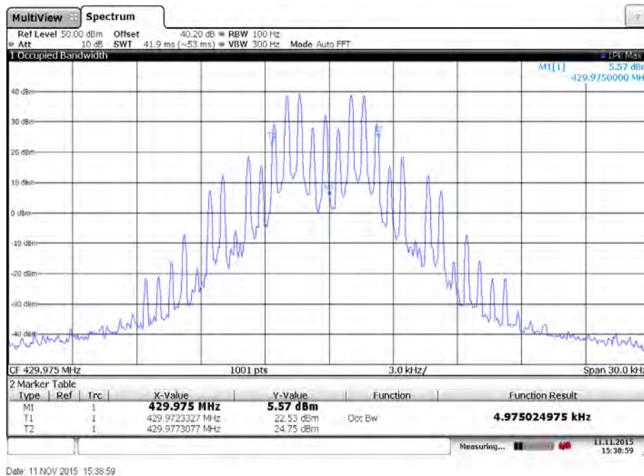
Plot 6: High channel / 1200 bits per second
