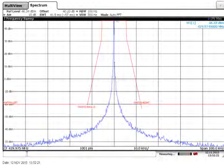
Plot 41: Emission mask D – High channel – 512 bits per second – High power – Carrier unmodulated
