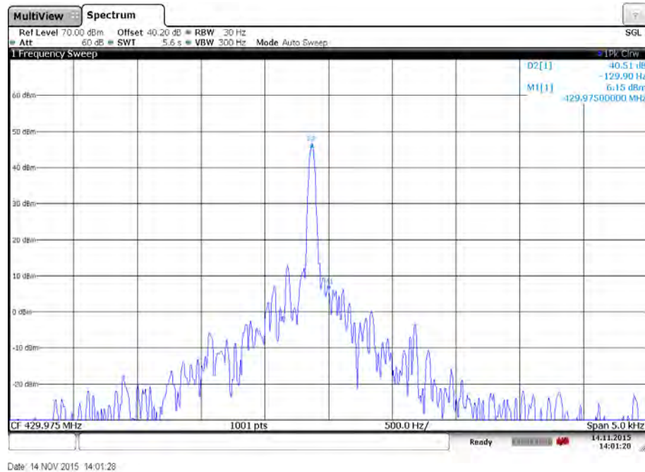
Plot 23: High channel – Temperature: 0°C
