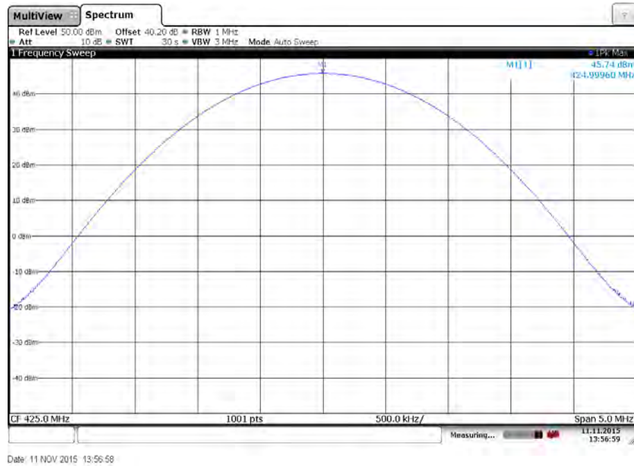
Plot 5: Middle channel – High power
