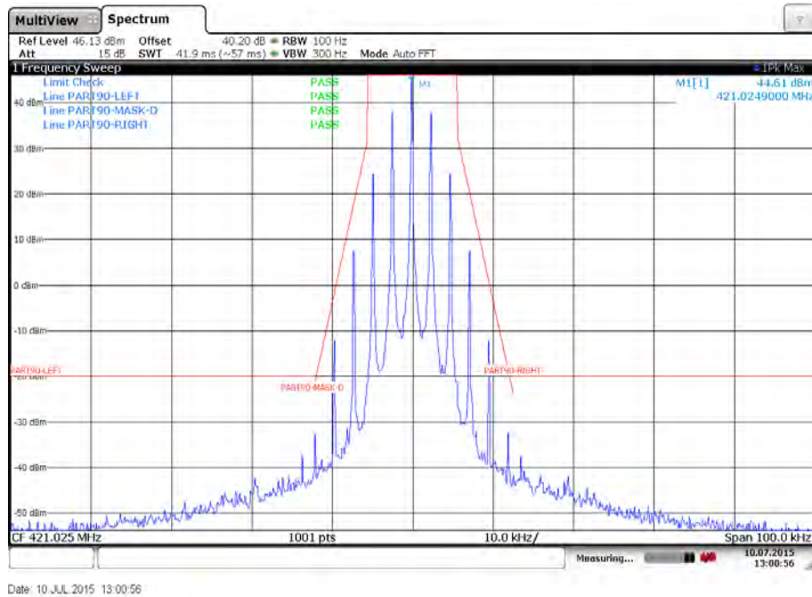
Plot 32: Emission mask D – Low channel – 4800 bits per second – High power – Carrier modulated
