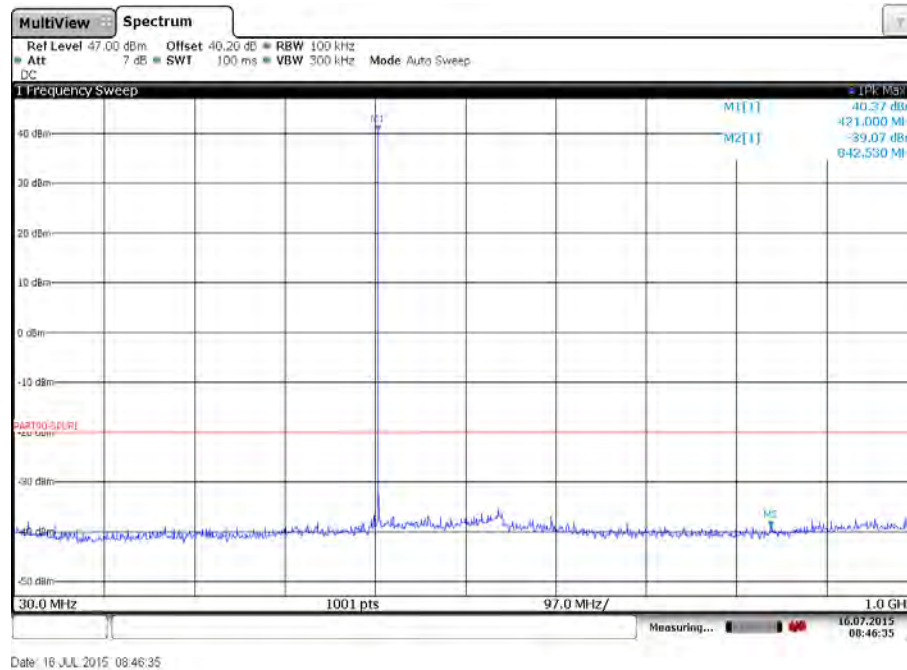
Plot 1: Low channel – Low power - 30 MHz to 1 GHz
