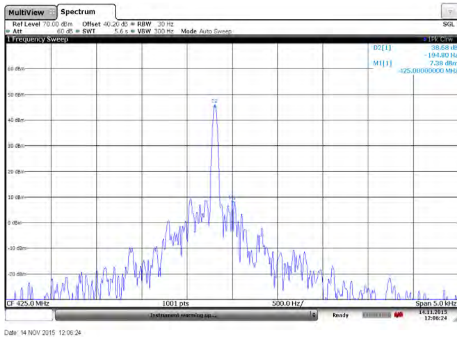
Plot 18: Middle channel – Temperature: 50°C
