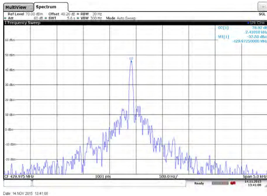
Plot 24: High channel – Temperature: 10°C
