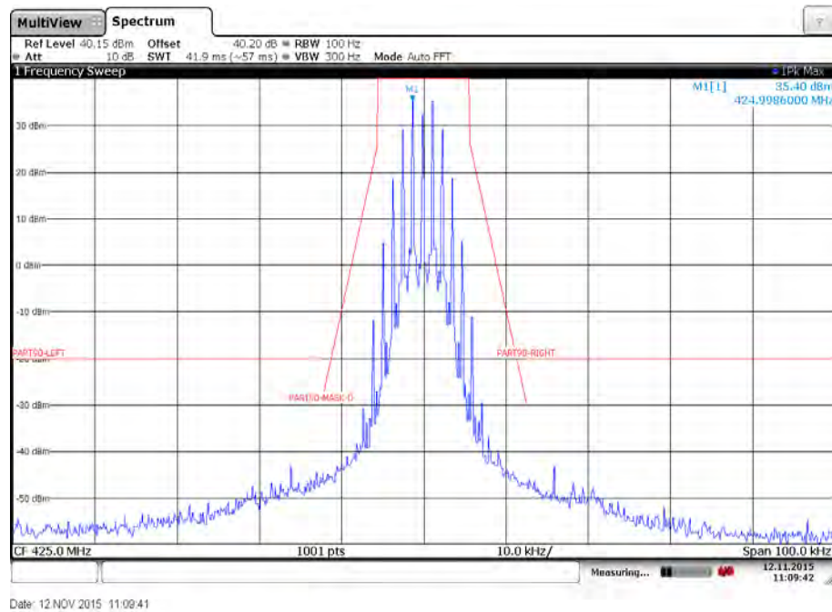
Plot 14: Emission mask D – Mid channel – 2400 bits per second – Low power – Carrier modulated
