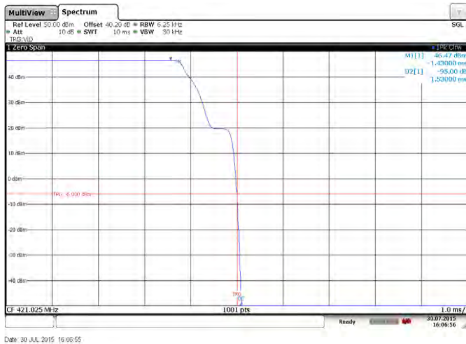
Plot 4: Lowest channel – Switch off (zoomed)
