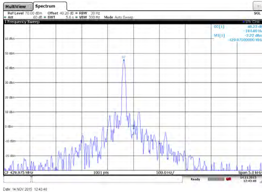
Plot 27: High channel – Temperature: 40°C
