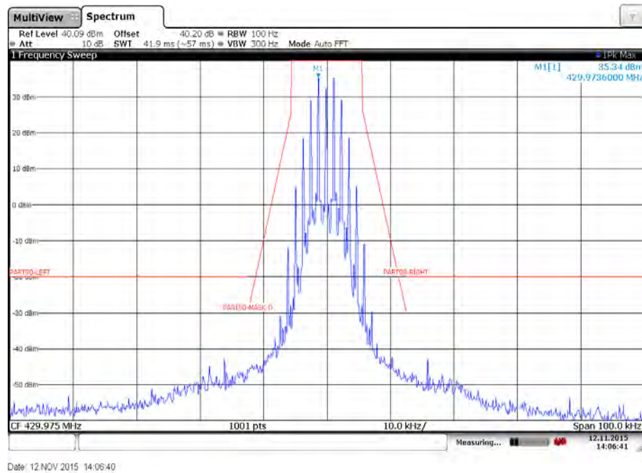
Plot 22: Emission mask D – High channel – 2400 bits per second – Low power – Carrier modulated
