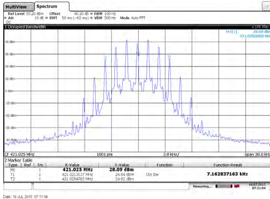
Plot 7: Low channel / 2400 bits per second
