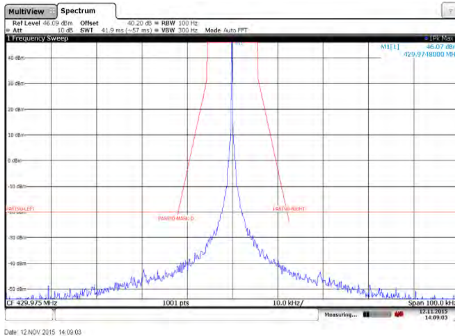
Plot 47: Emission mask D – High channel – 4800 bits per second – High power – Carrier unmodulated
