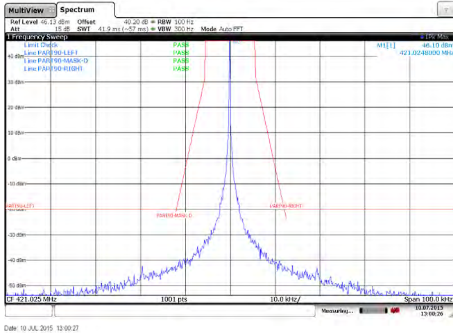
Plot 31: Emission mask D – Low channel – 4800 bits per second – High power – Carrier unmodulated
