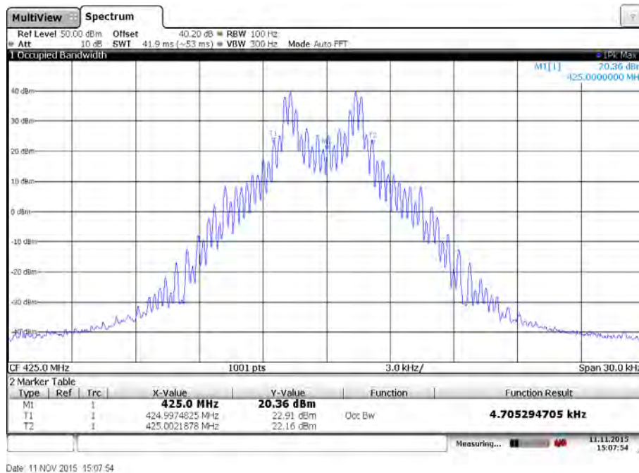
Plot 2: Middle channel / 512 bits per second
