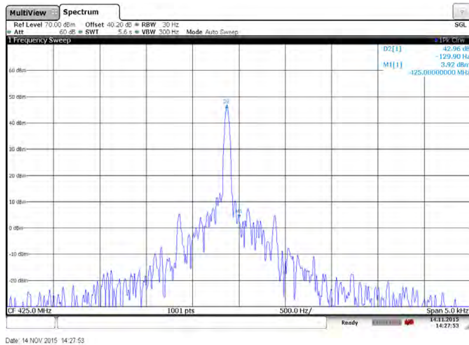
Plot 12: Middle channel – Temperature: -10°C
