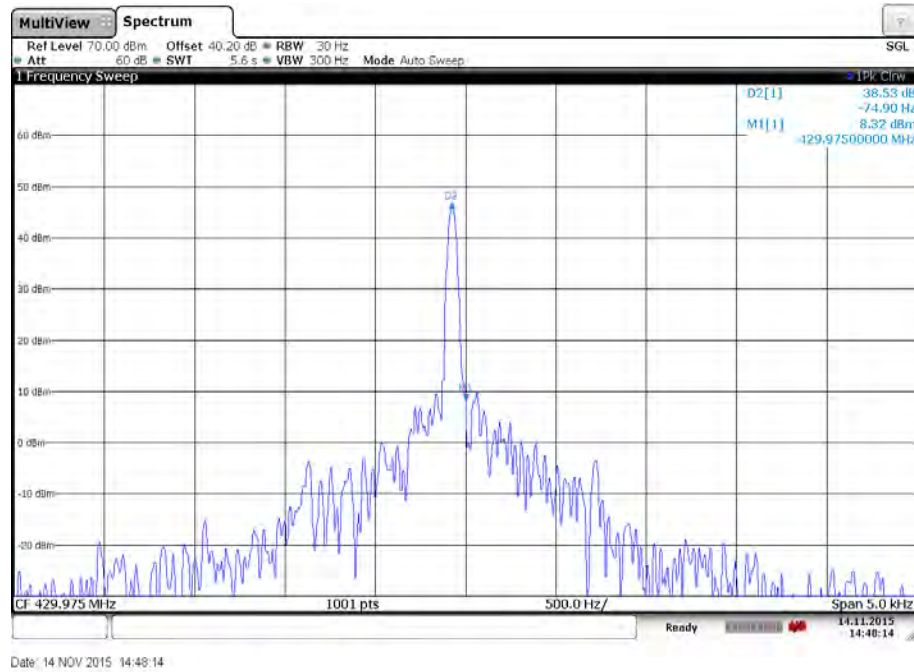
Plot 21: High channel – Temperature: -20°C
