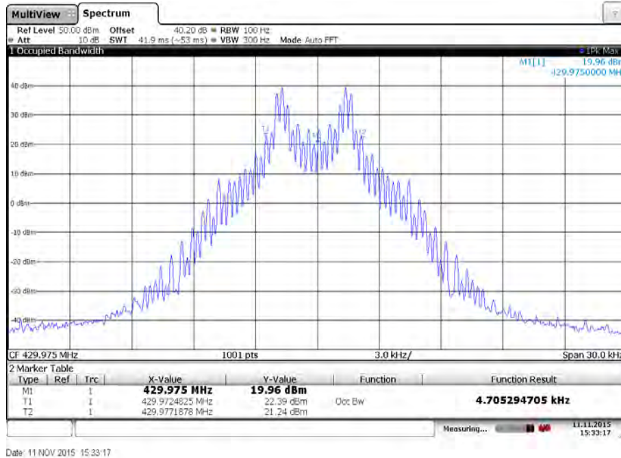
Plot 3: High channel / 512 bits per second
