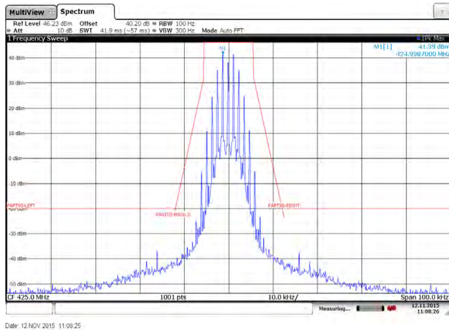
Plot 38: Emission mask D – Mid channel – 2400 bits per second – High power – Carrier modulated
