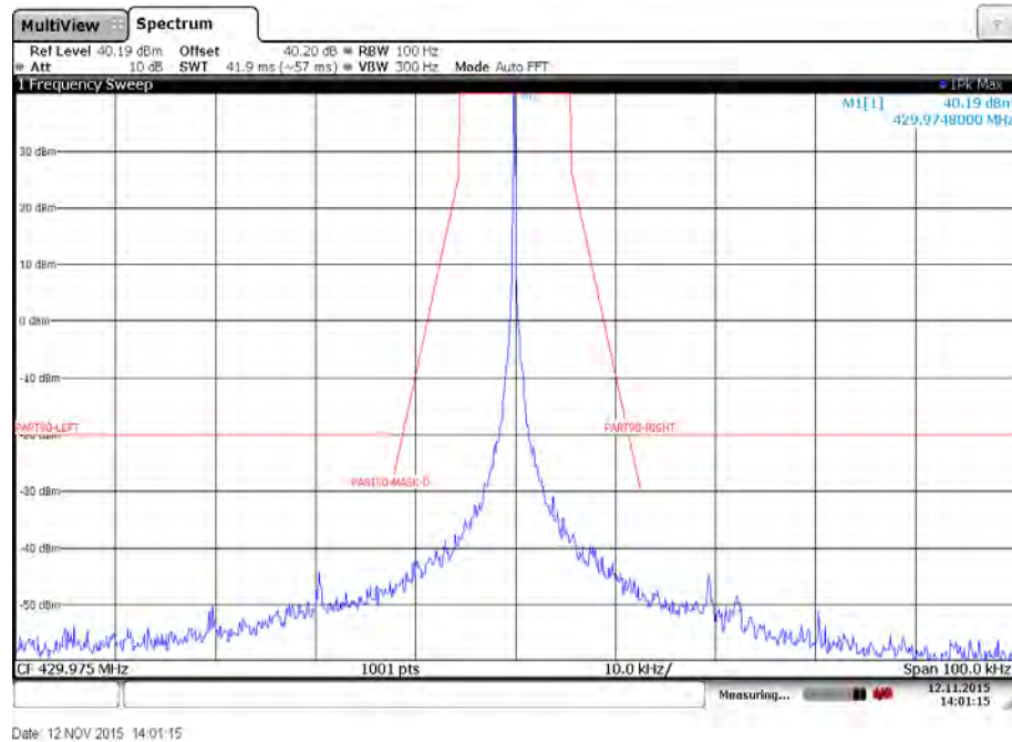
Plot 19: Emission mask D – High channel – 1200 bits per second – Low power – Carrier unmodulated
