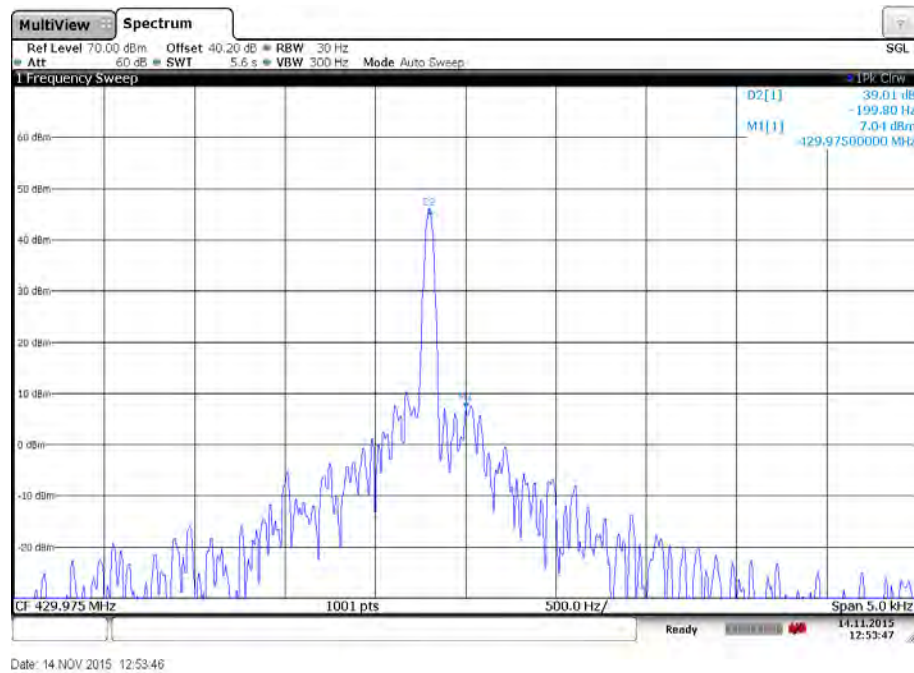
Plot 26: High channel – Temperature: 30°C
