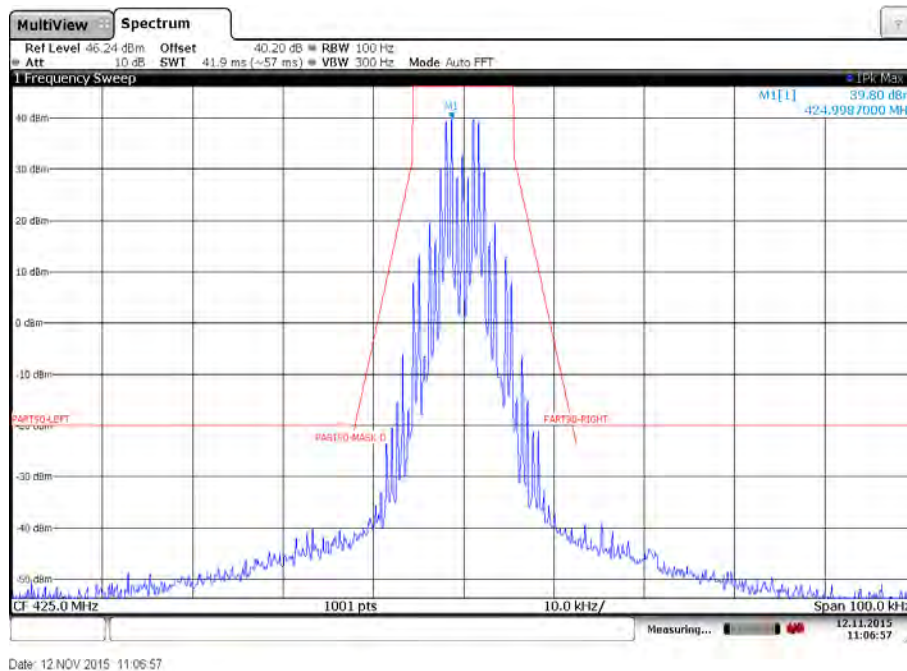
Plot 36: Emission mask D – Mid channel – 1200 bits per second – High power – Carrier modulated
