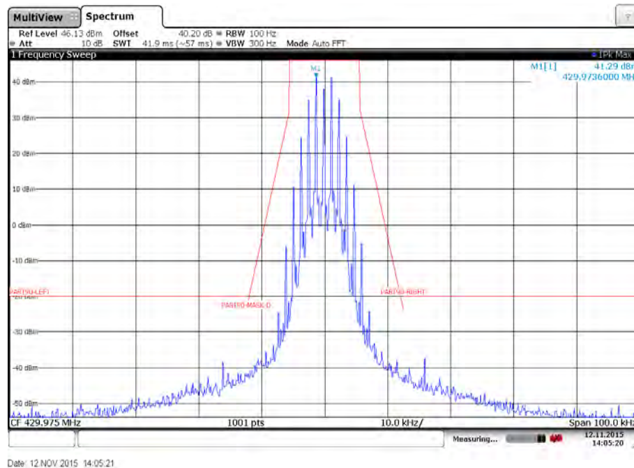
Plot 46: Emission mask D – High channel – 2400 bits per second – High power – Carrier modulated
