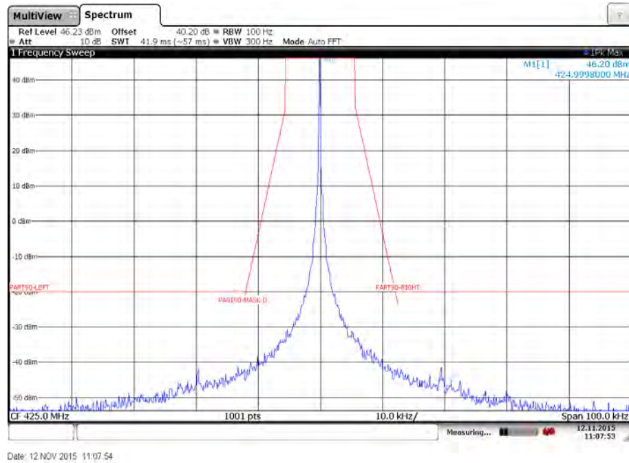
Plot 37: Emission mask D – Mid channel – 2400 bits per second – High power – Carrier unmodulated
