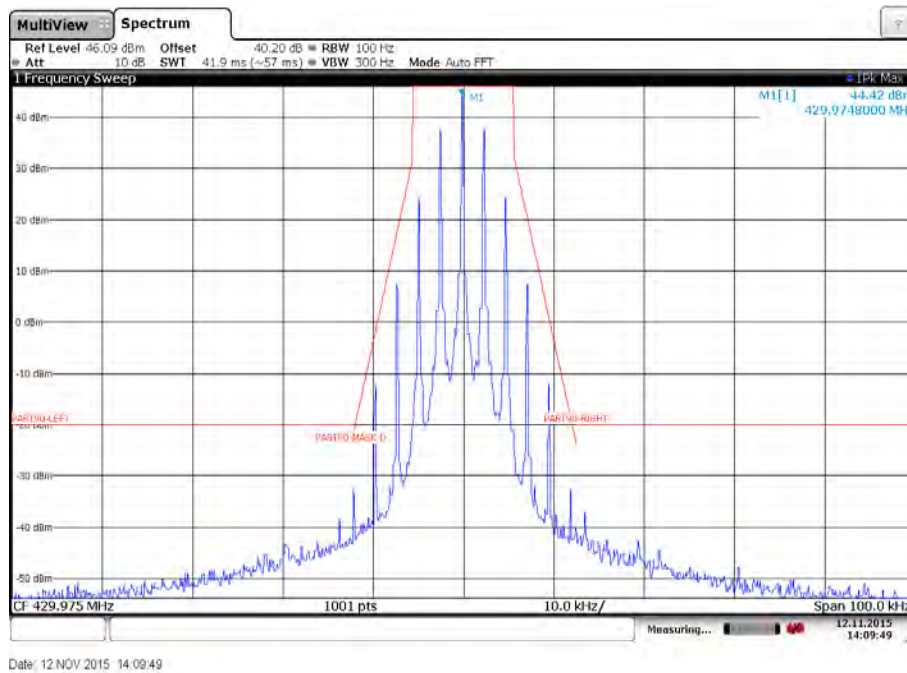
Plot 48: Emission mask D – High channel – 4800 bits per second – High power – Carrier modulated
