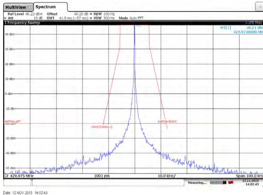
Plot 43: Emission mask D – High channel – 1200 bits per second – High power – Carrier unmodulated
