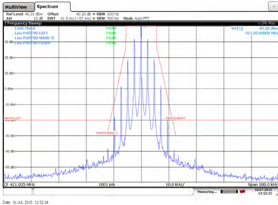
Plot 8: Emission mask D – Low channel – 4800 bits per second – Low power – Carrier modulated
