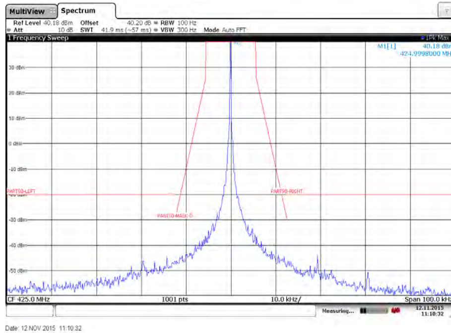
Plot 15: Emission mask D – Mid channel – 4800 bits per second – Low power – Carrier unmodulated
