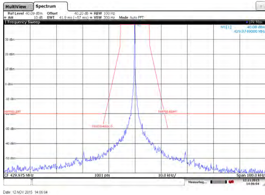
Plot 21: Emission mask D – High channel – 2400 bits per second – Low power – Carrier unmodulated
