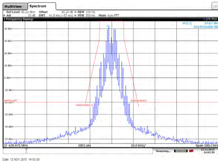
Plot 44: Emission mask D – High channel – 1200 bits per second – High power – Carrier modulated
