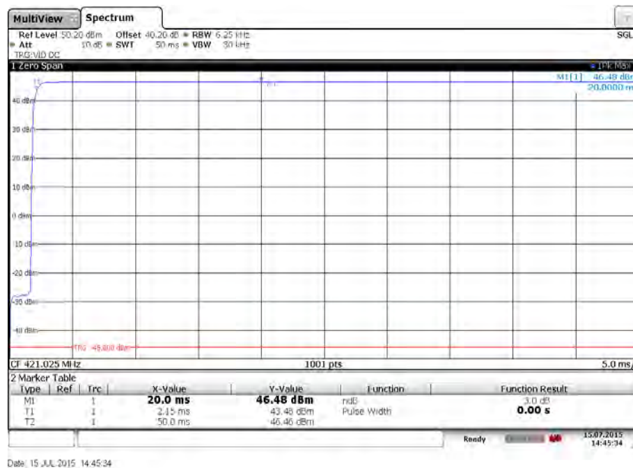
Plot 2: Lowest channel – Switch on (zoomed)
