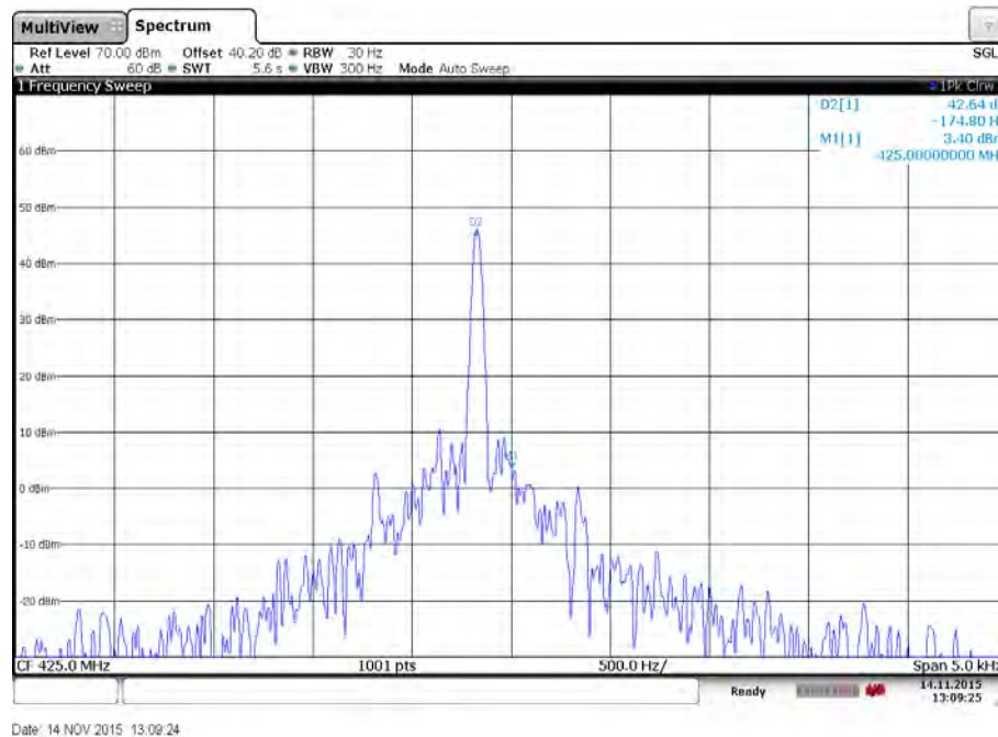
Plot 20: Middle channel – Temperature: 20°C – 115% Voltage
