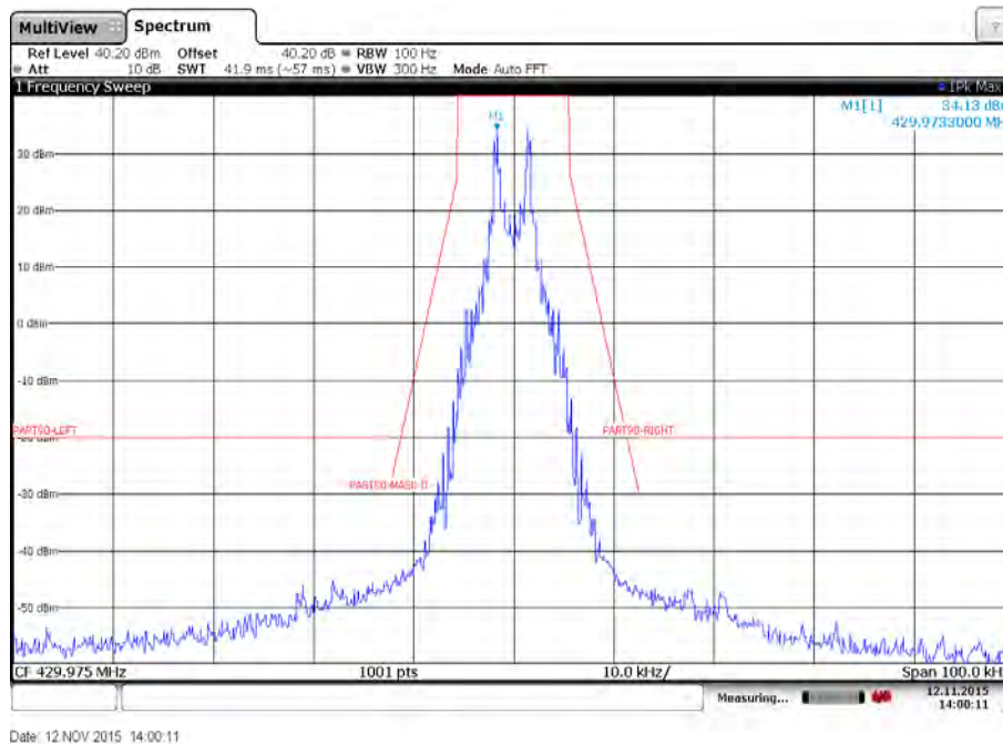
Plot 18: Emission mask D – High channel – 512 bits per second – Low power – Carrier modulated
