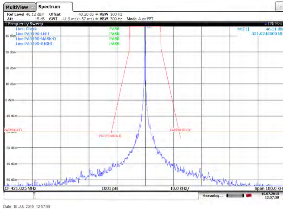
Plot 27: Emission mask D – Low channel – 1200 bits per second – High power – Carrier unmodulated
