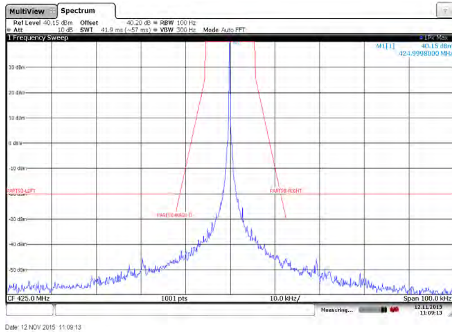
Plot 13: Emission mask D – Mid channel – 2400 bits per second – Low power – Carrier unmodulated
