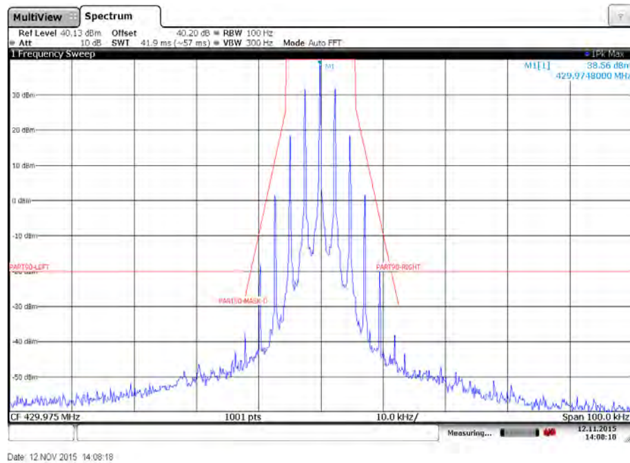
Plot 24: Emission mask D – High channel – 4800 bits per second – Low power – Carrier modulated
