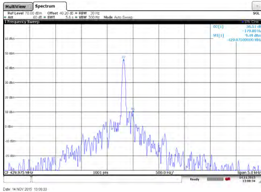
Plot 29: High channel – Temperature: 20°C – 85% Voltage
