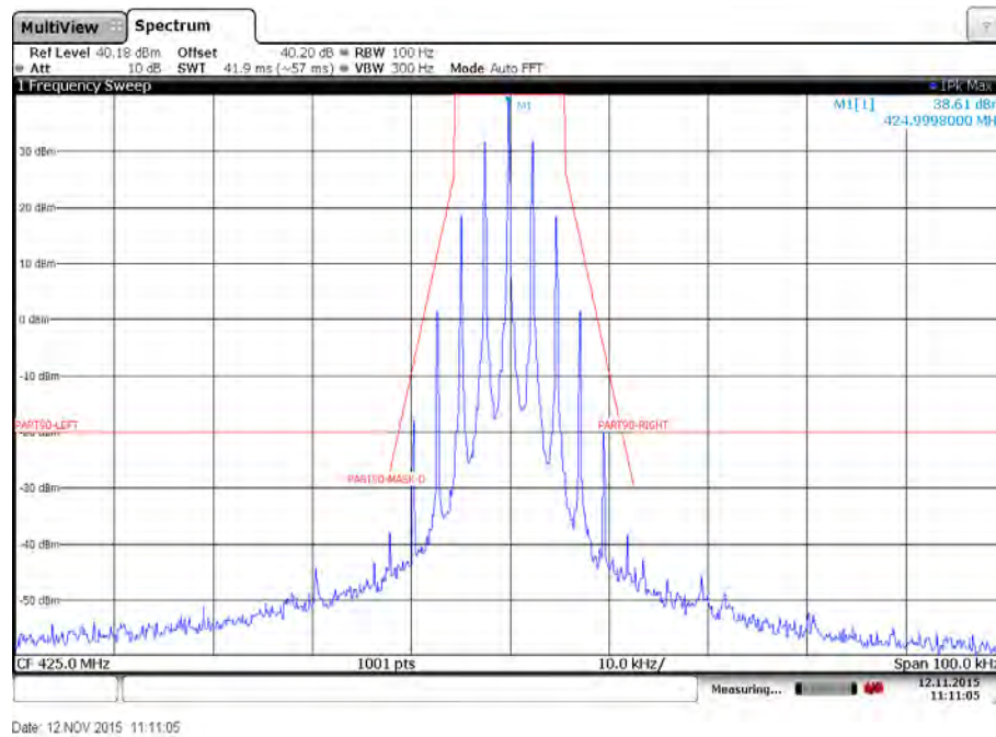
Plot 16: Emission mask D – Mid channel – 4800 bits per second – Low power – Carrier modulated
