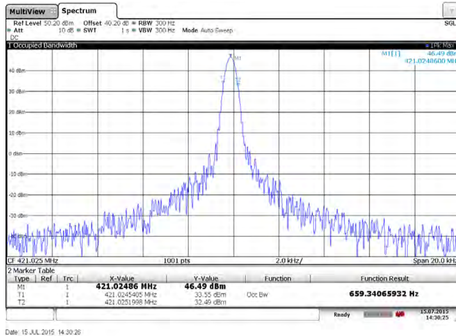
Plot 1: Lowest channel - Carrier
