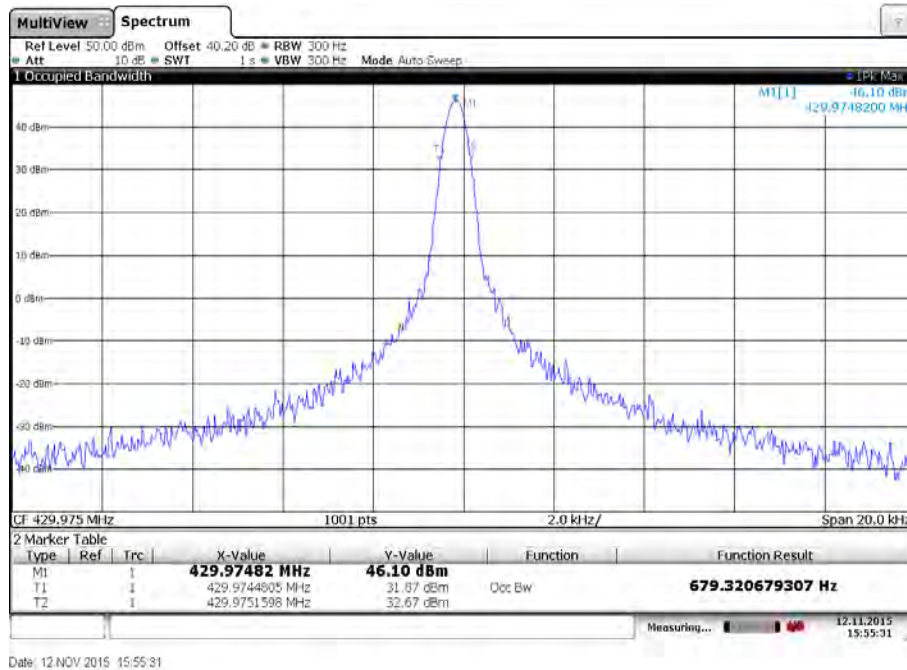
Plot 9: Highest channel - Carrier
