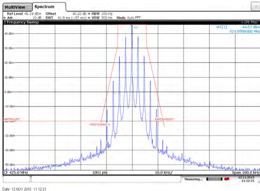
Plot 40: Emission mask D – Mid channel – 4800 bits per second – High power – Carrier modulated
