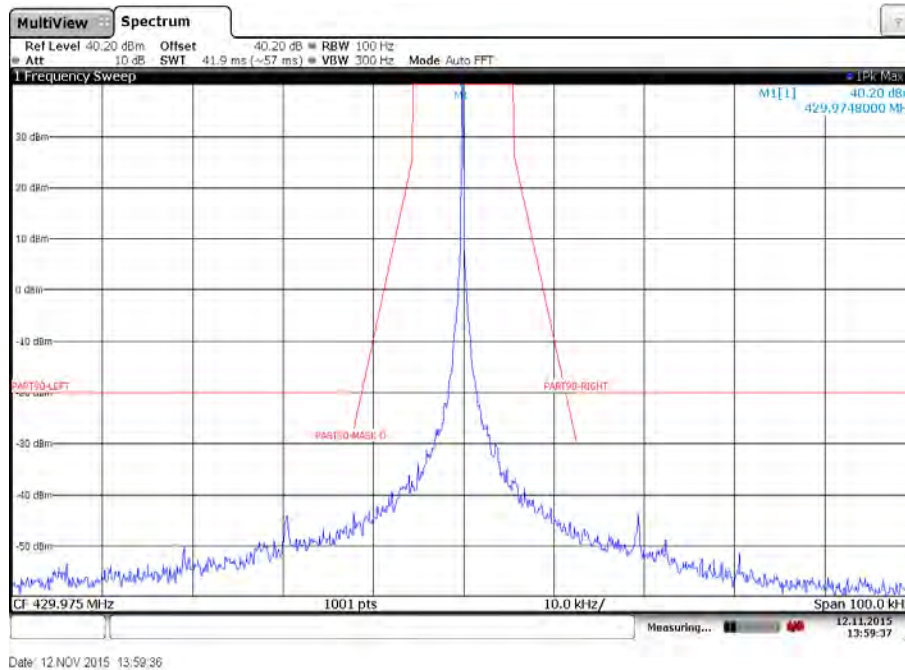
Plot 17: Emission mask D – High channel – 512 bits per second – Low power – Carrier unmodulated
