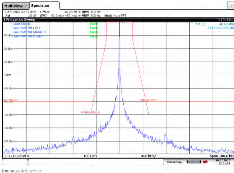
Plot 5: Emission mask D – Low channel – 2400 bits per second – Low power – Carrier unmodulated
