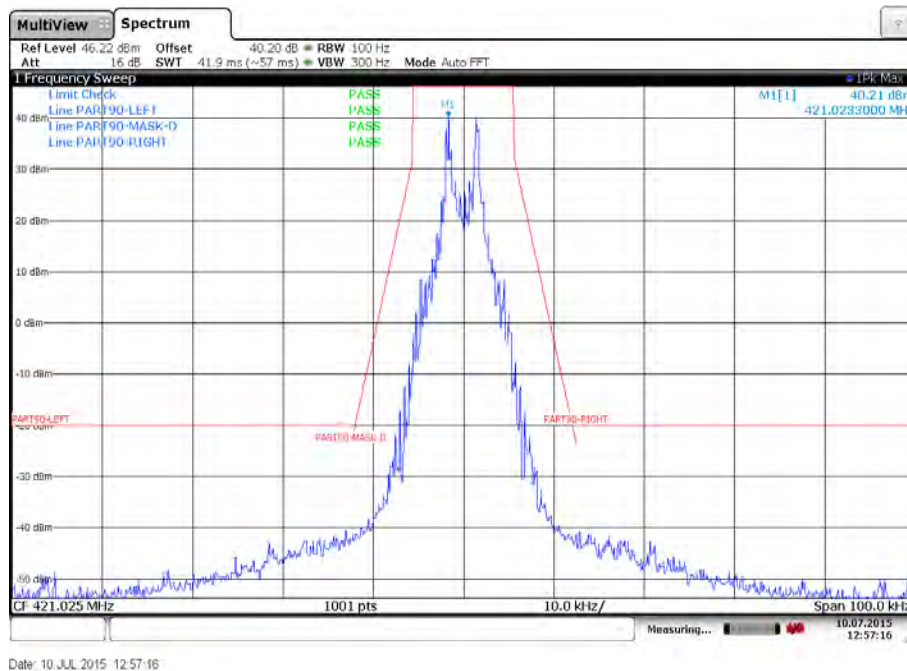
Plot 26: Emission mask D – Low channel – 512 bits per second – High power – Carrier modulated
