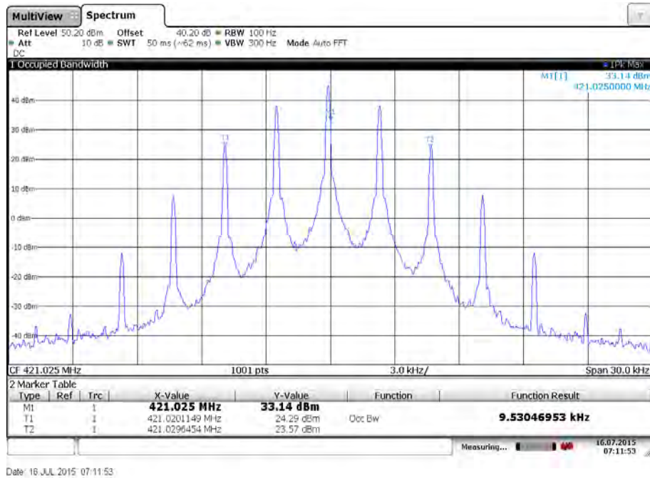
Plot 10: Low channel / 4800 bits per second
