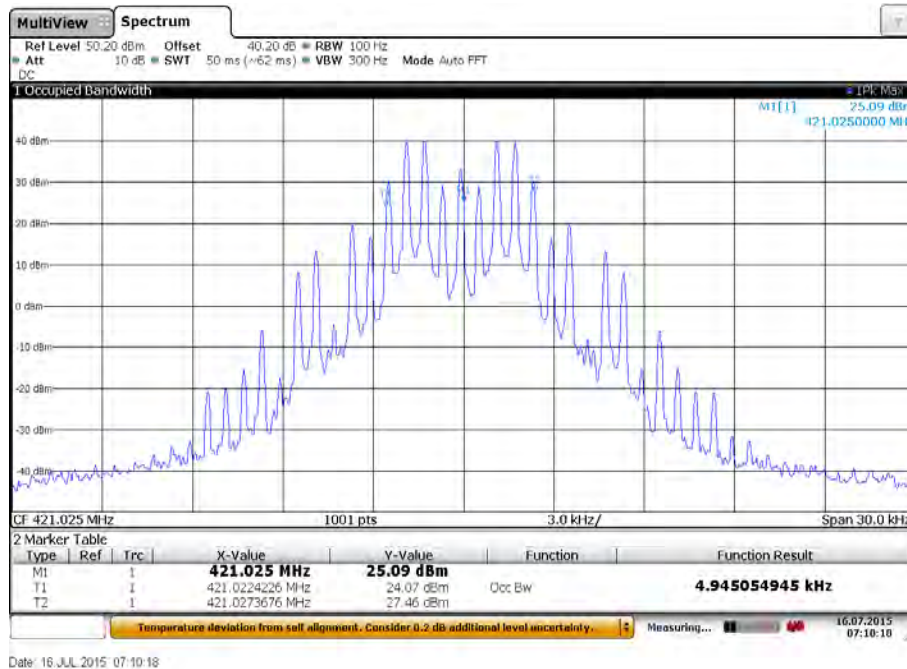
Plot 4: Low channel / 1200 bits per second
