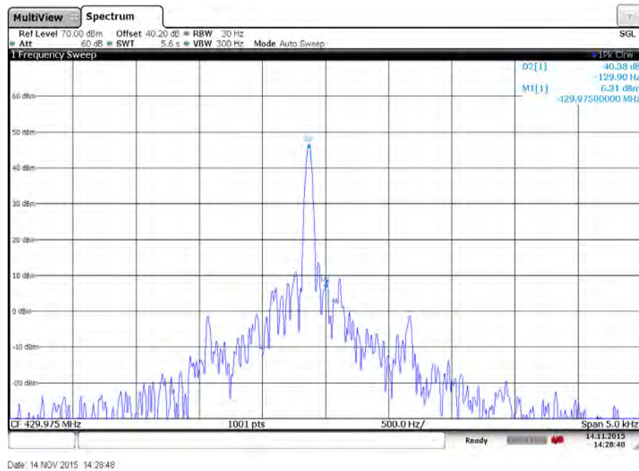
Plot 22: High channel – Temperature: -10°C
