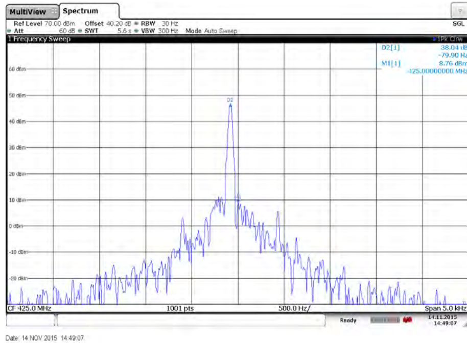
Plot 11: Middle channel – Temperature: -20°C
