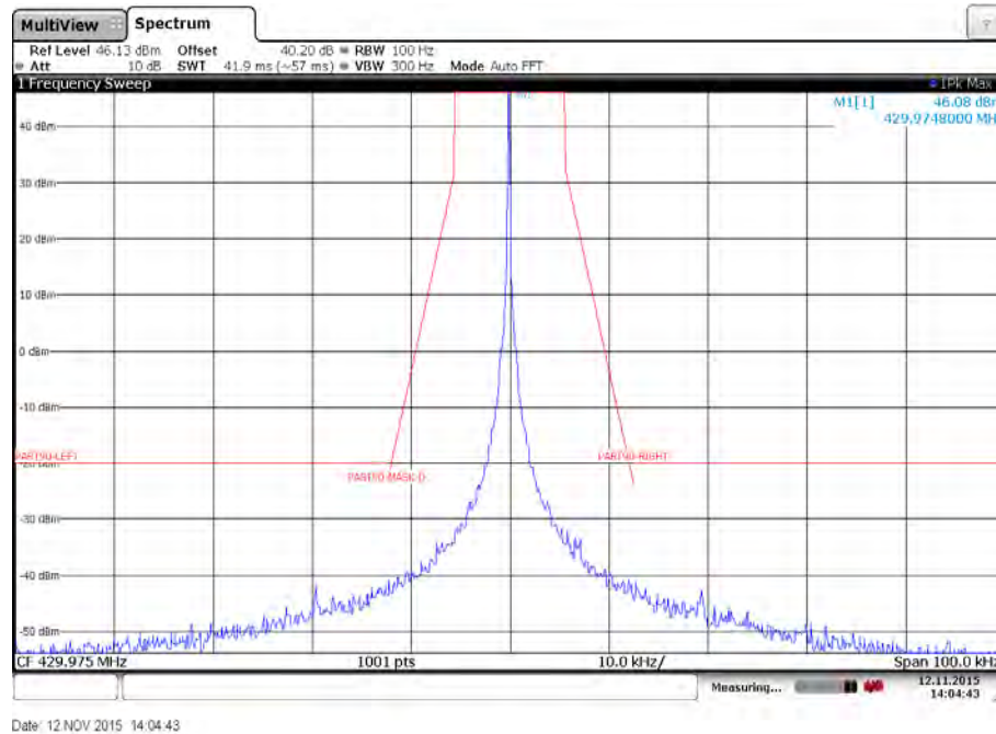
Plot 45: Emission mask D – High channel – 2400 bits per second – High power – Carrier unmodulated
