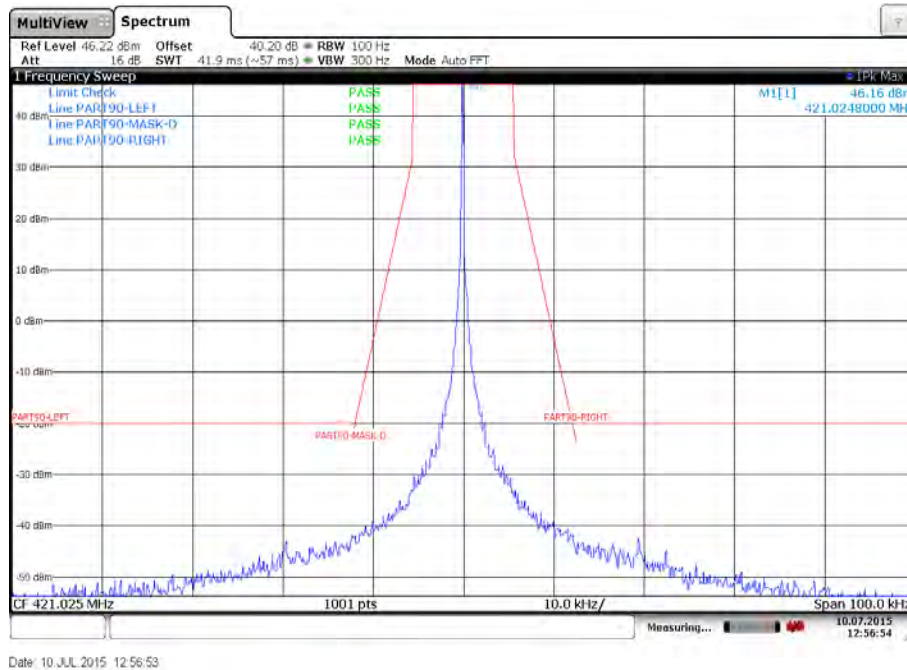
Plot 25: Emission mask D – Low channel – 512 bits per second – High power – Carrier unmodulated
