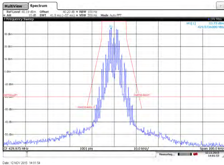
Plot 20: Emission mask D – High channel – 1200 bits per second – Low power – Carrier modulated
