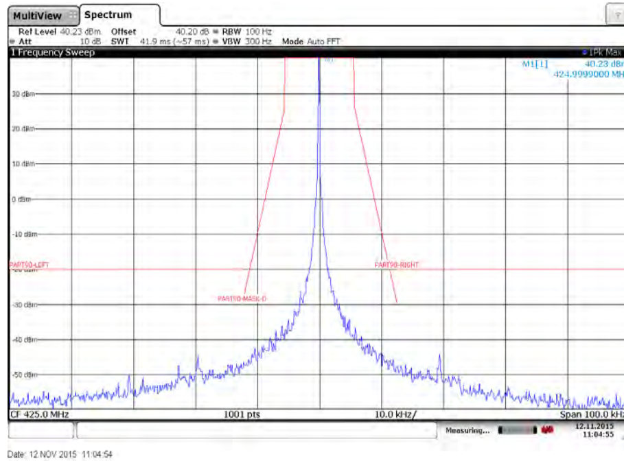
Plot 11: Emission mask D – Mid channel – 1200 bits per second – Low power – Carrier unmodulated
