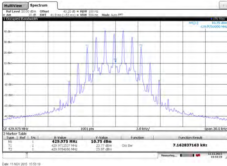
Plot 9: High channel / 2400 bits per second
