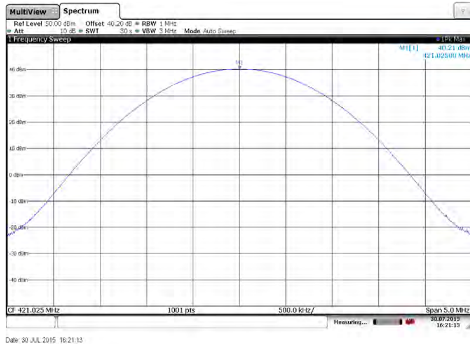
Plot 1: Lowest channel – Low power
