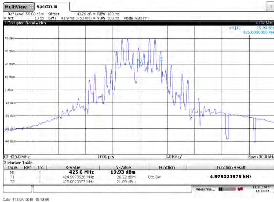
Plot 5: Middle channel / 1200 bits per second
