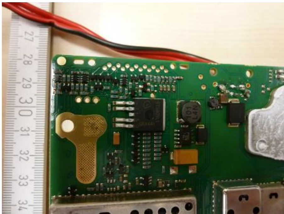
Photo 44: RF module
