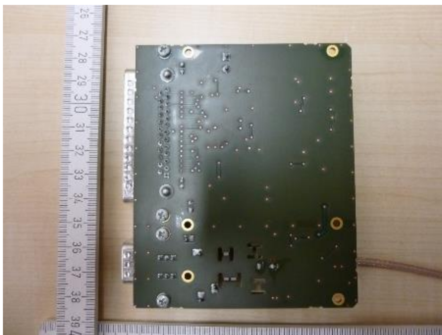
Photo 48: RF module
