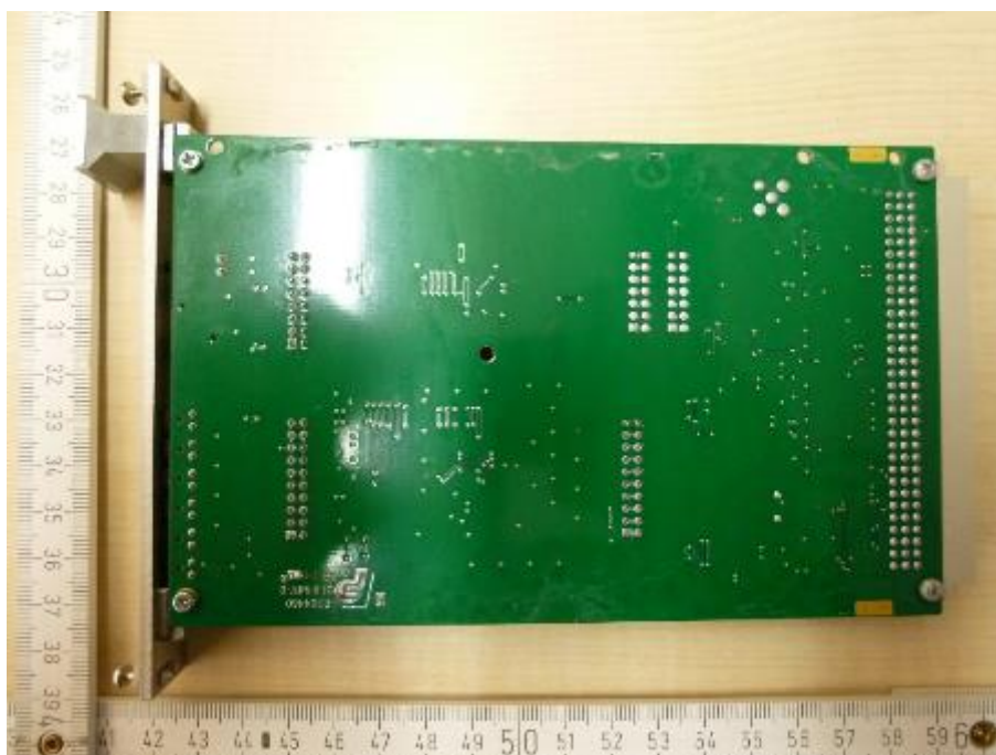
Photo 22: RC09 module
