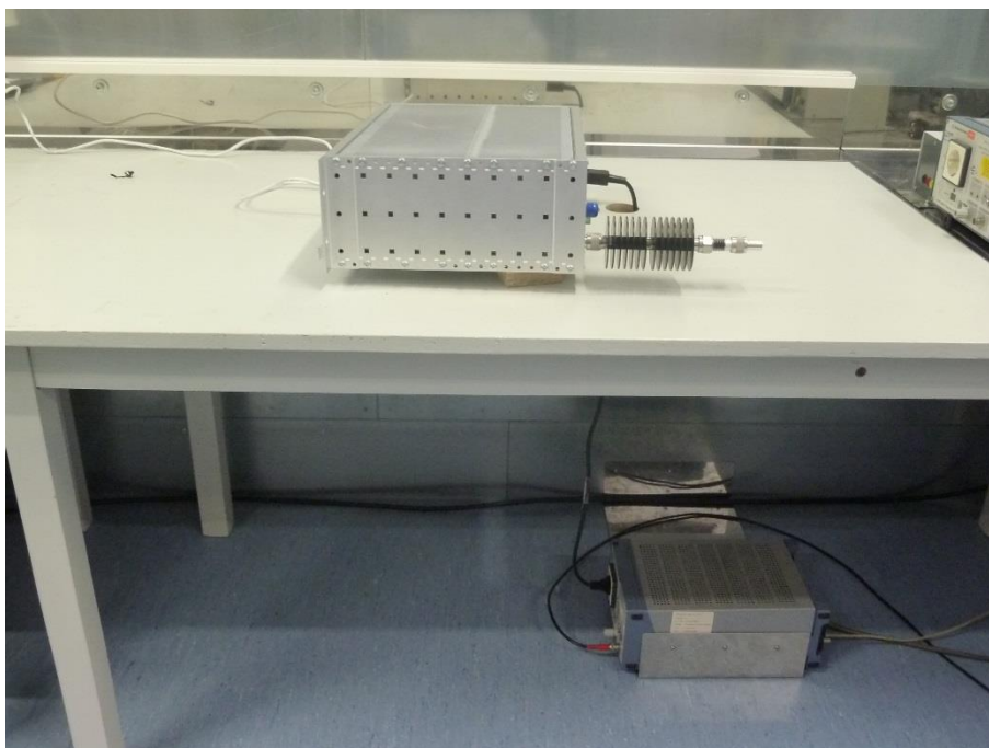
Photo 9: AC-conducted measurements
