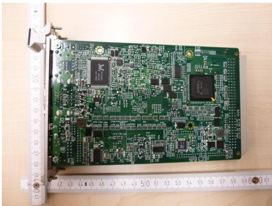
Photo 12: BSC module
