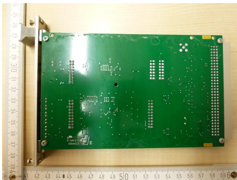
Photo 22: RC09 module
