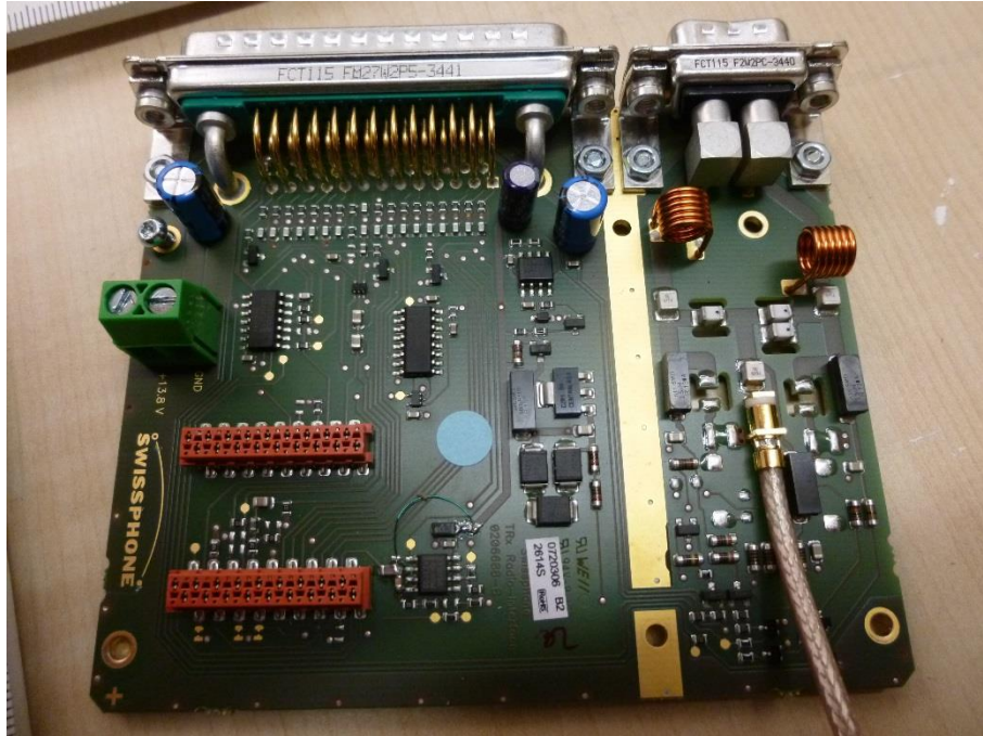
Photo 49: RF module
