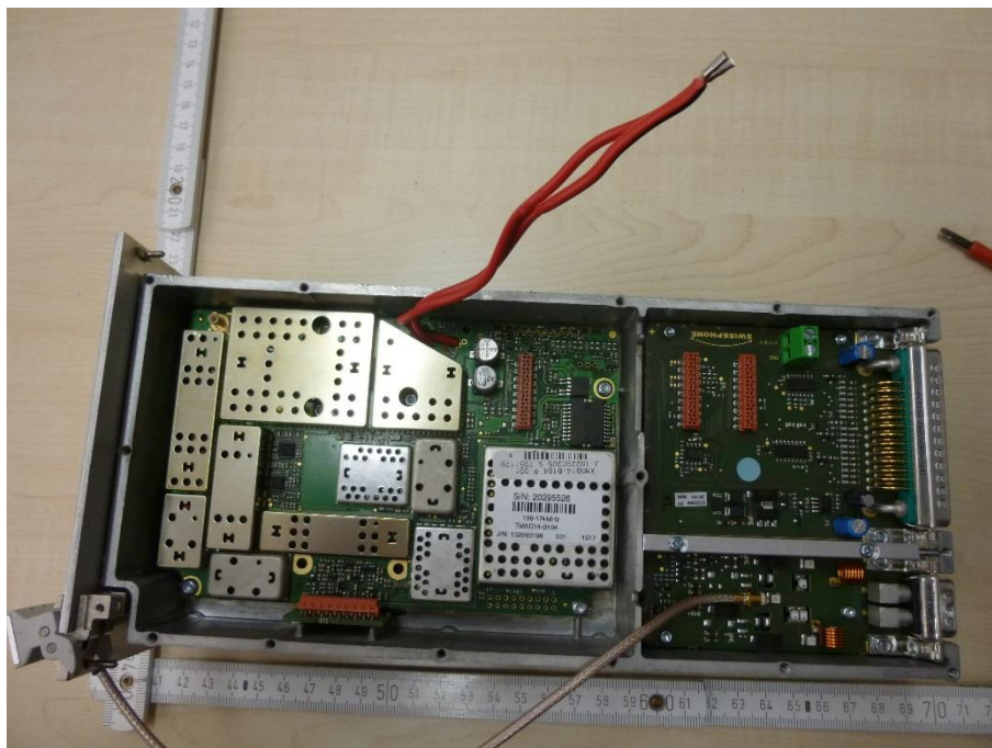
Photo 44: RF module
