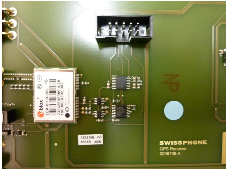
Photo 17: GPS module
