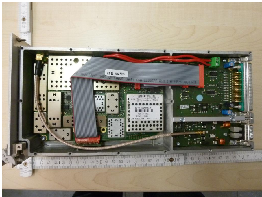
Photo 40: RF module
