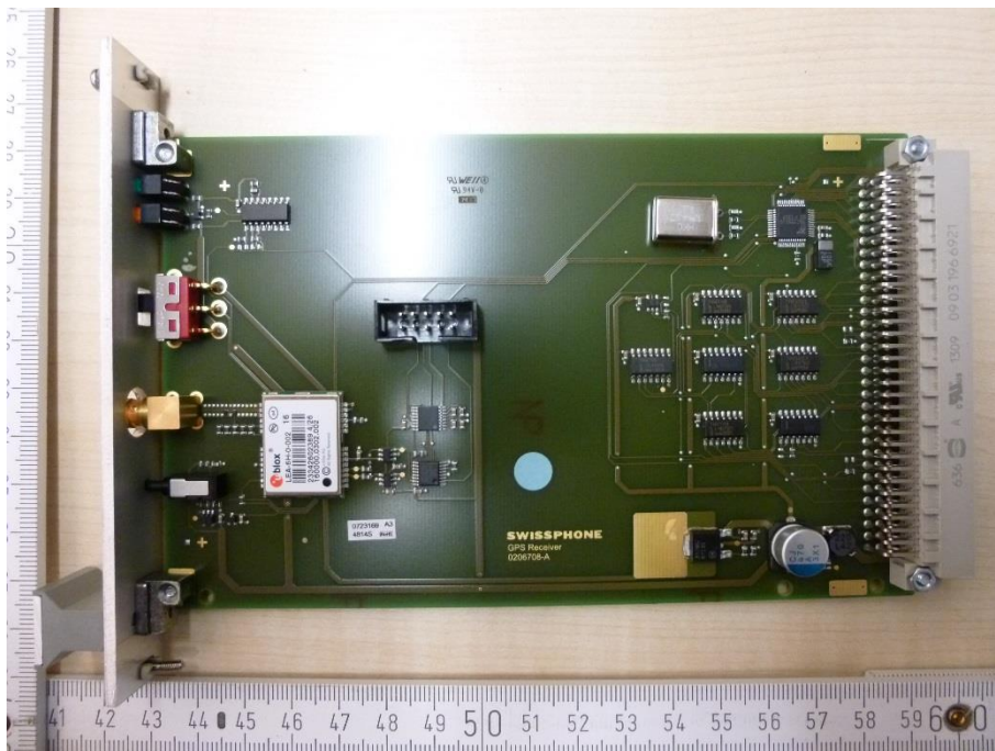
Photo 16: GPS module
