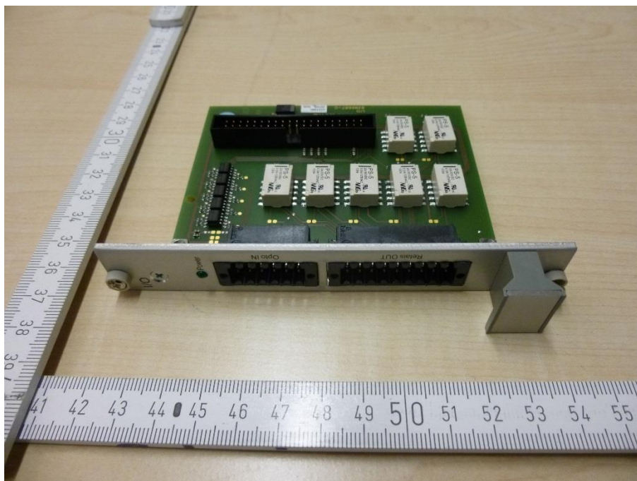
Photo 29: I/O module
