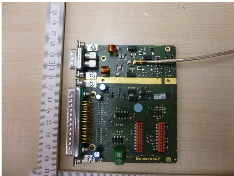
Photo 48: RF module
