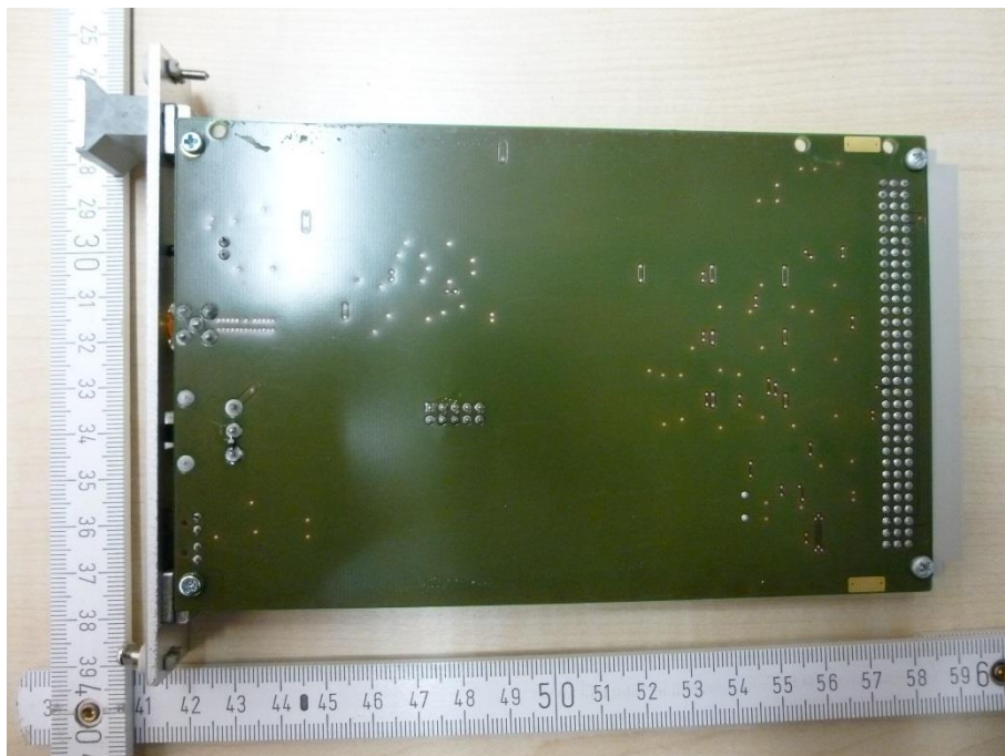
Photo 18: GPS module
