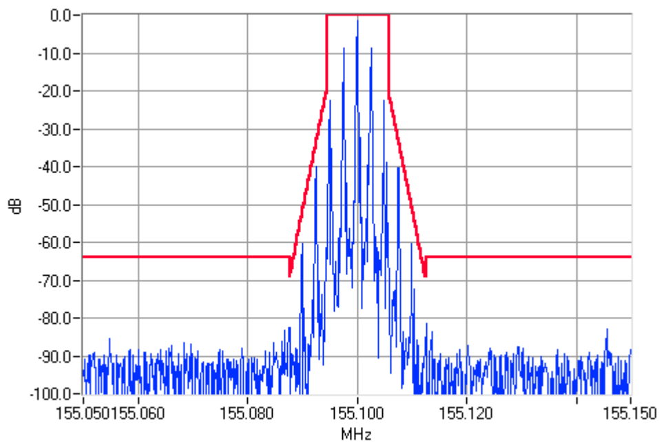
Analogue Modulation 155.1000MHz Mask D 25W Pass
