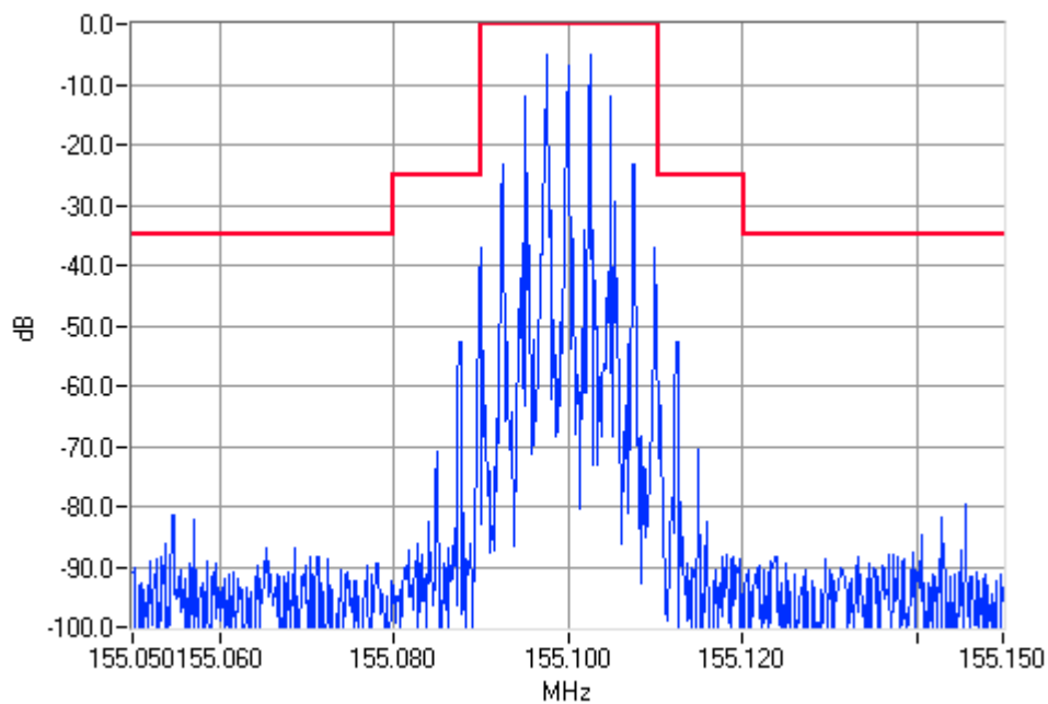
Analogue Modulation 155.1000MHz Mask B 25W Pass
