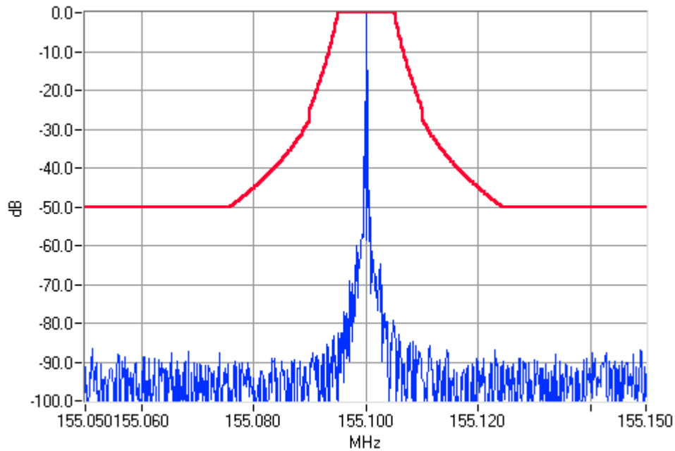
Unmodulated 155.1000MHz Mask C 25W Pass
