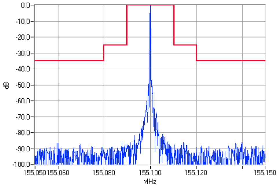
Unmodulated 155.1000MHz Mask B 25W Pass
