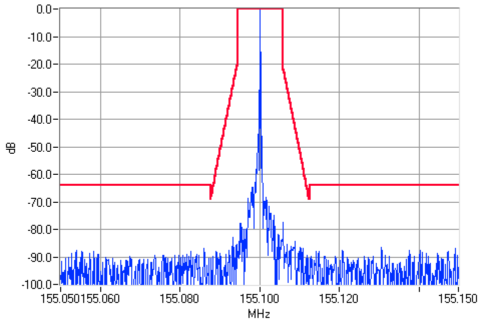
Unmodulated 155.1000MHz Mask D 25W Pass
