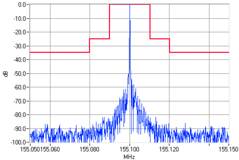
Unmodulated 155.1000MHz Mask B 1W Pass
