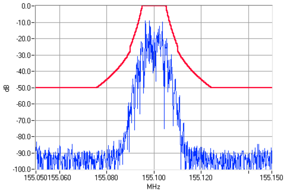
Digital Modulation 155.1000MHz Mask C 1W Pass
