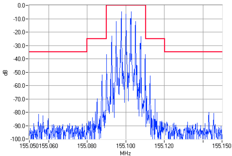
Analogue Modulation 155.1000MHz Mask B 1W Pass
