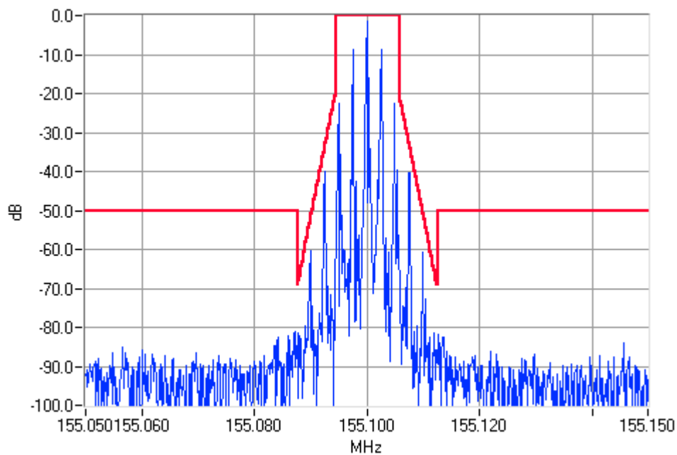
Analogue Modulation 155.1000MHz Mask D 1W Pass
