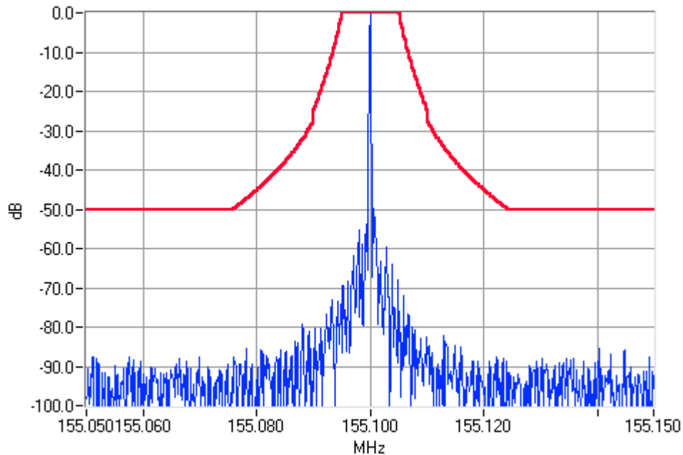
Unmodulated 155.1000MHz Mask C 1W Pass
