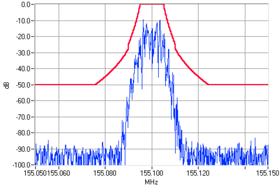
Digital Modulation 155.1000MHz Mask C 25W Pass
