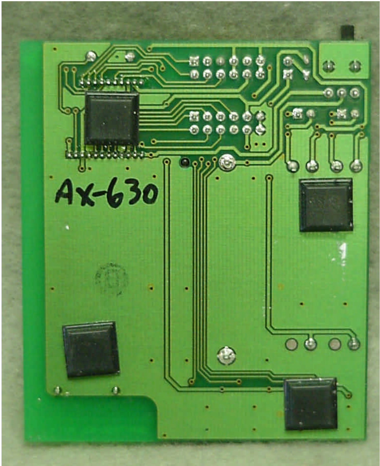
Photo 3. EUT, Bottom View of Test Board
