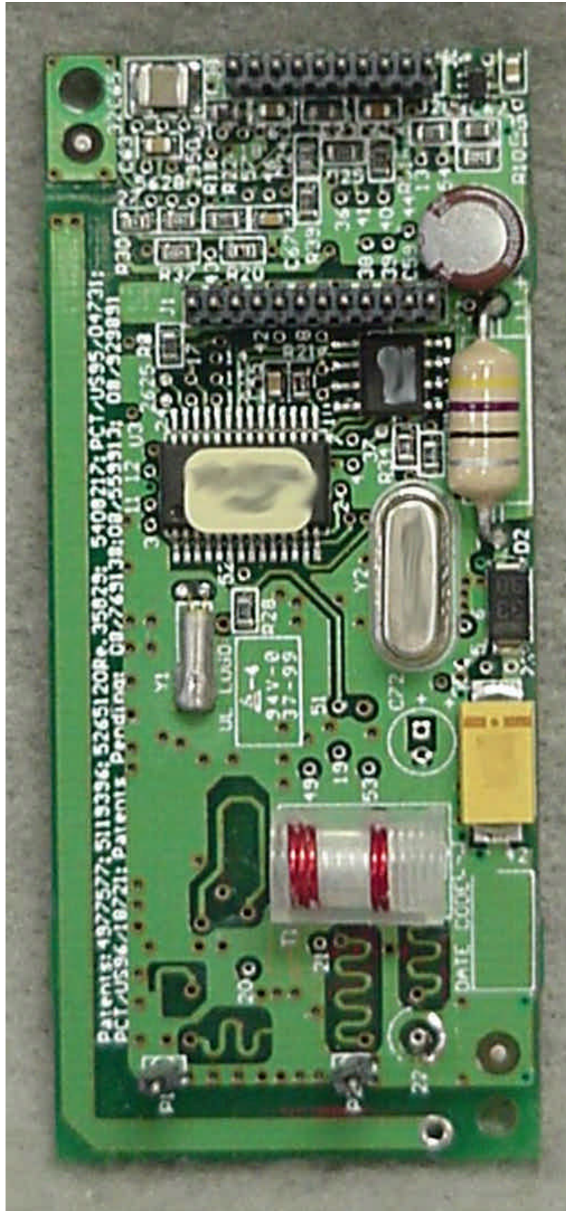
Photo 5. EUT, Bottom View
