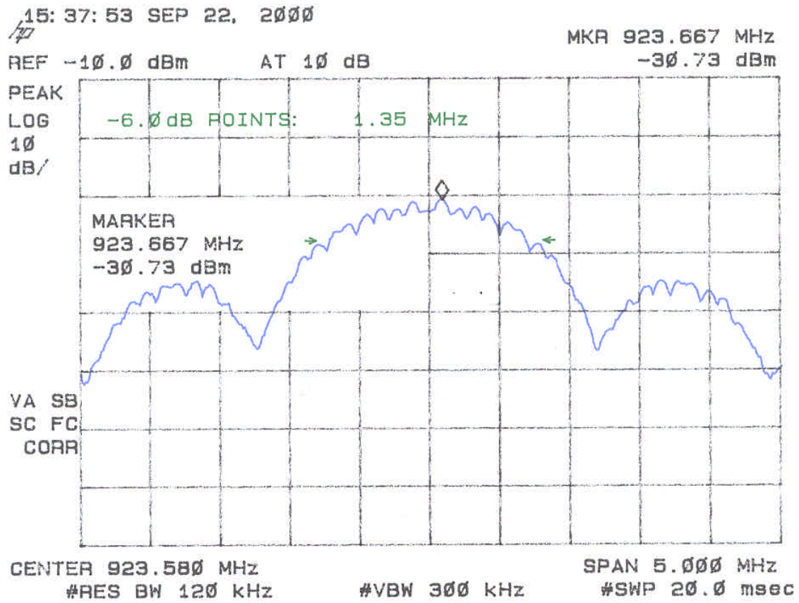
Figure 7 6 dB Bandwidth per FCC Section 15.247(a)(2)
