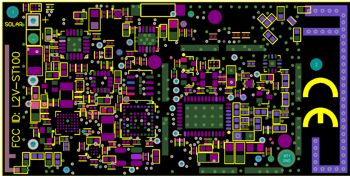
Picture 4 – Component side ST100 PCB with FCC ID and CE Mark
