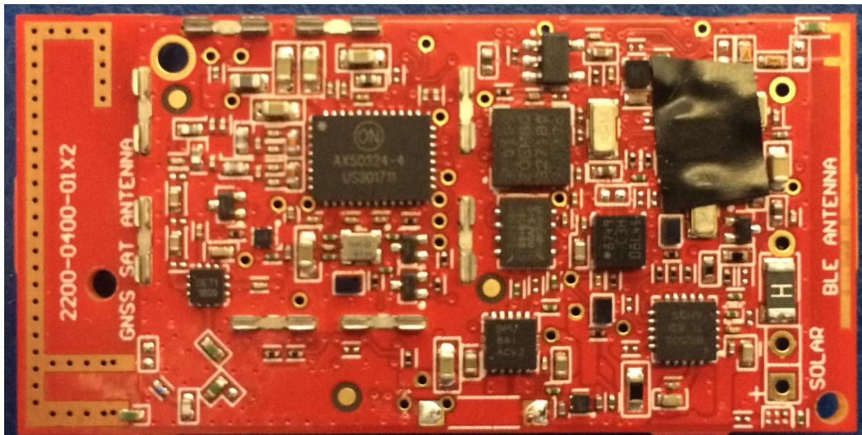
Picture 3 – Component side without shield.
