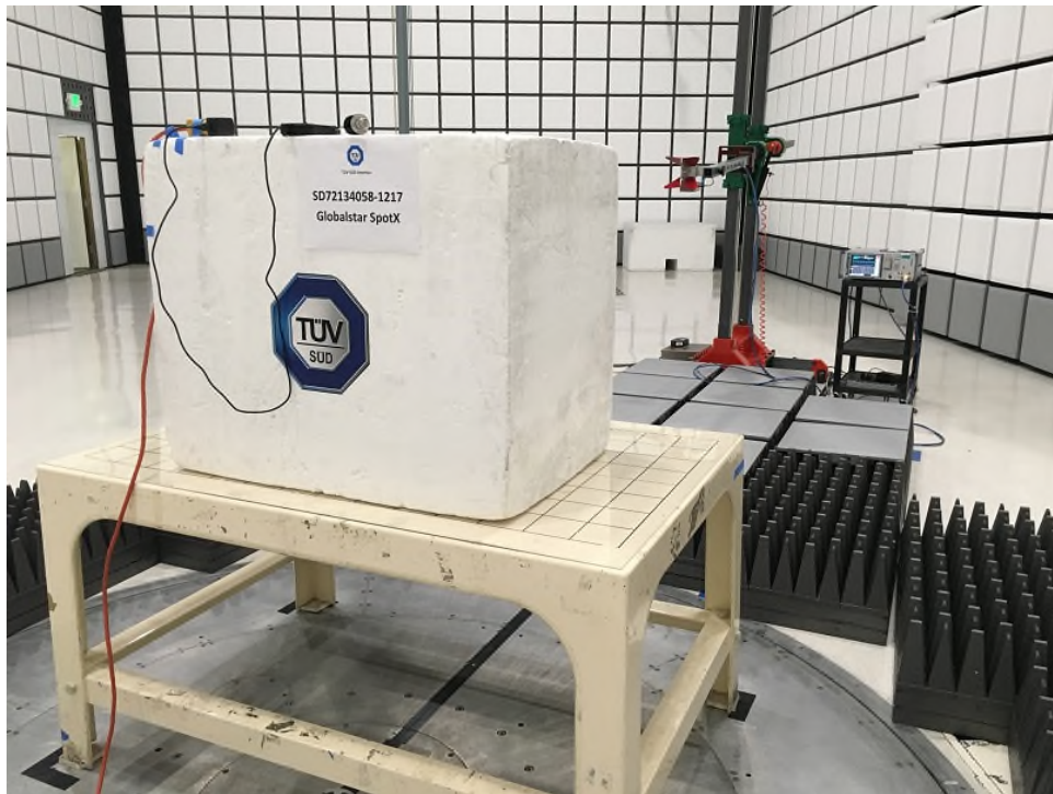
Radiated Emissions Above 1GHz Rear (Transmit Mode)
