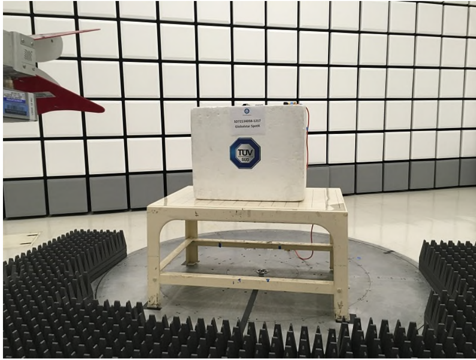
Radiated Emissions Above 1GHz Front (Transmit Mode)
