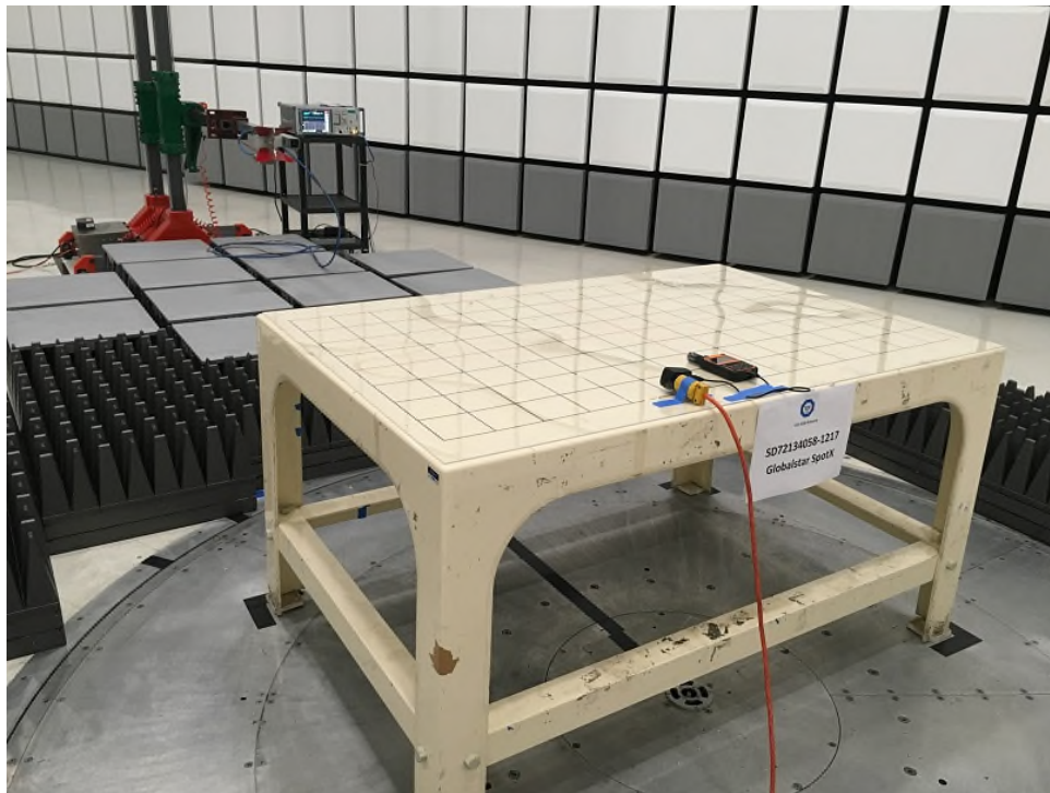
Radiated Emissions Above 1GHz Rear (Standby Mode)
