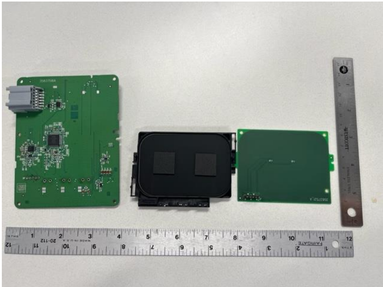
Figure 1 4196 PCBs Top
