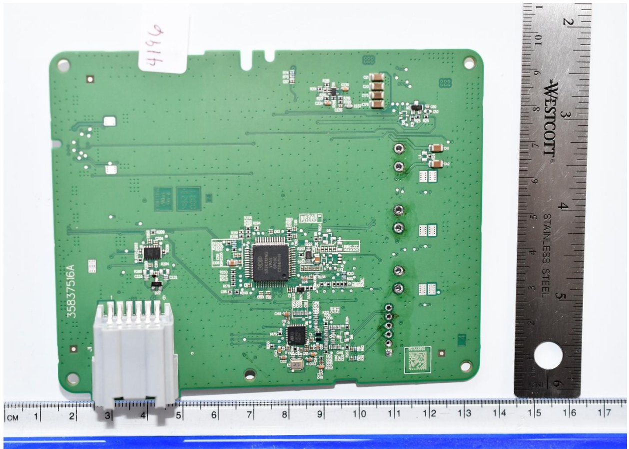
Figure 3 PCB side 1
