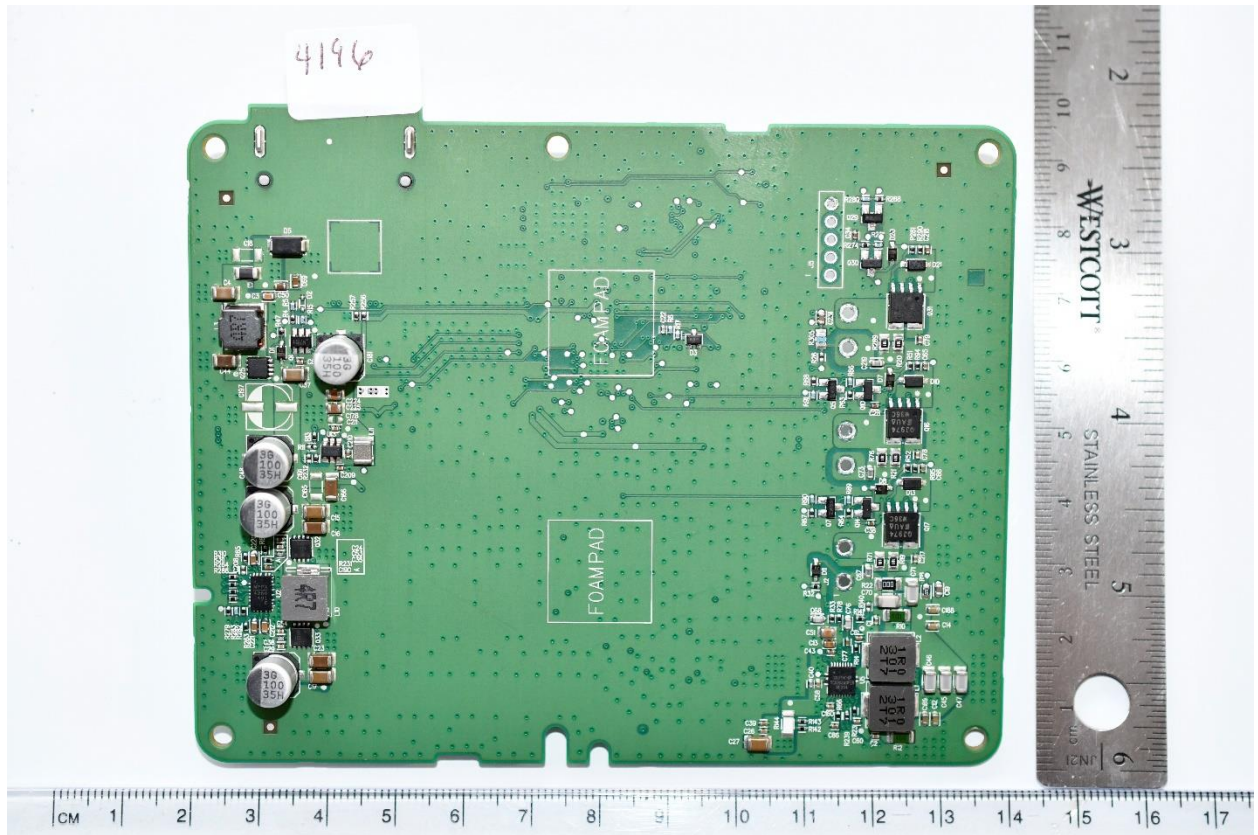
Figure 7 PCB side 2
