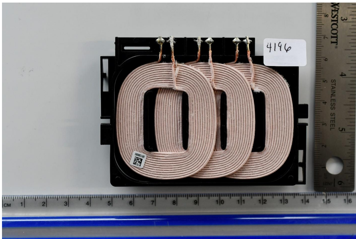
Figure 8 Coil Board side 1
