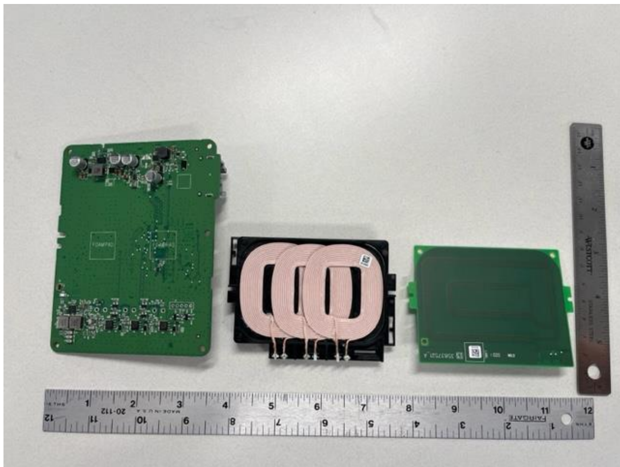
Figure 4 4196 PCBs Bottom
