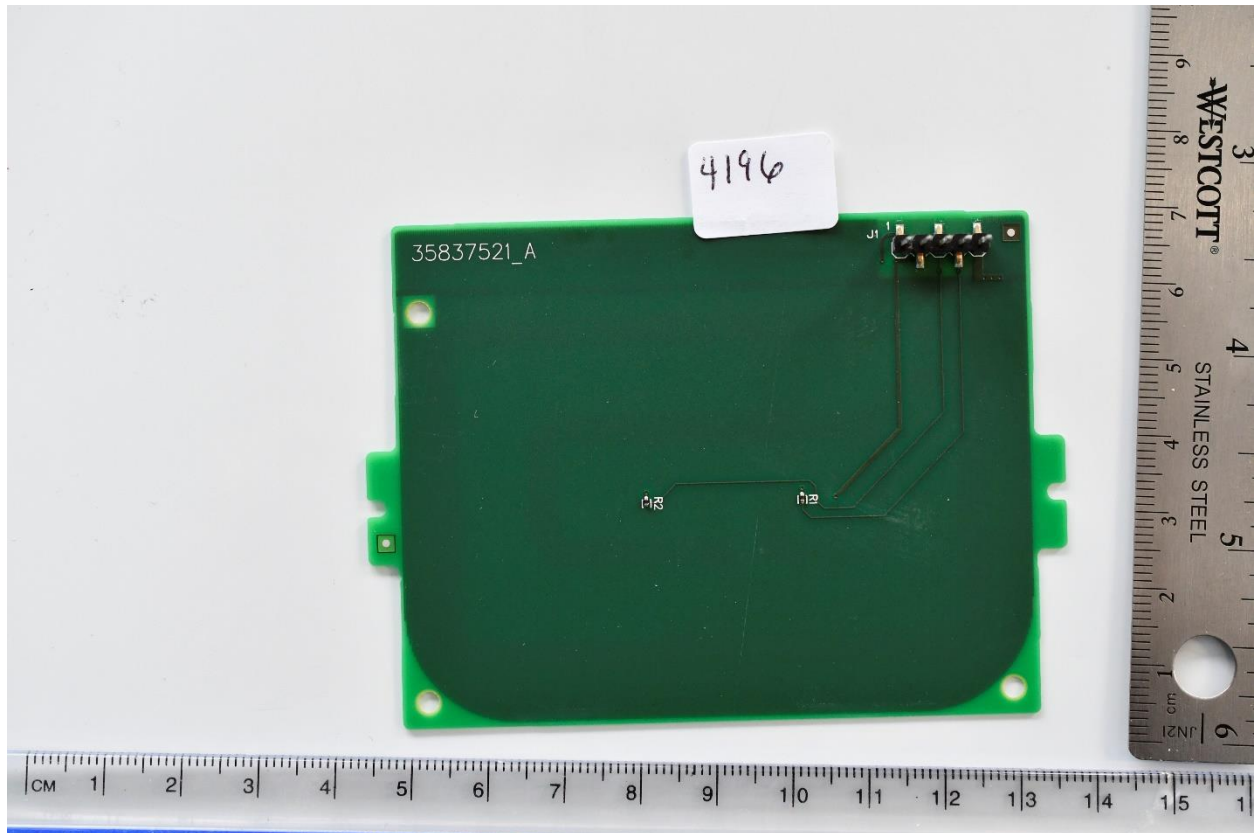
Figure 11 Antenna Board side 2
