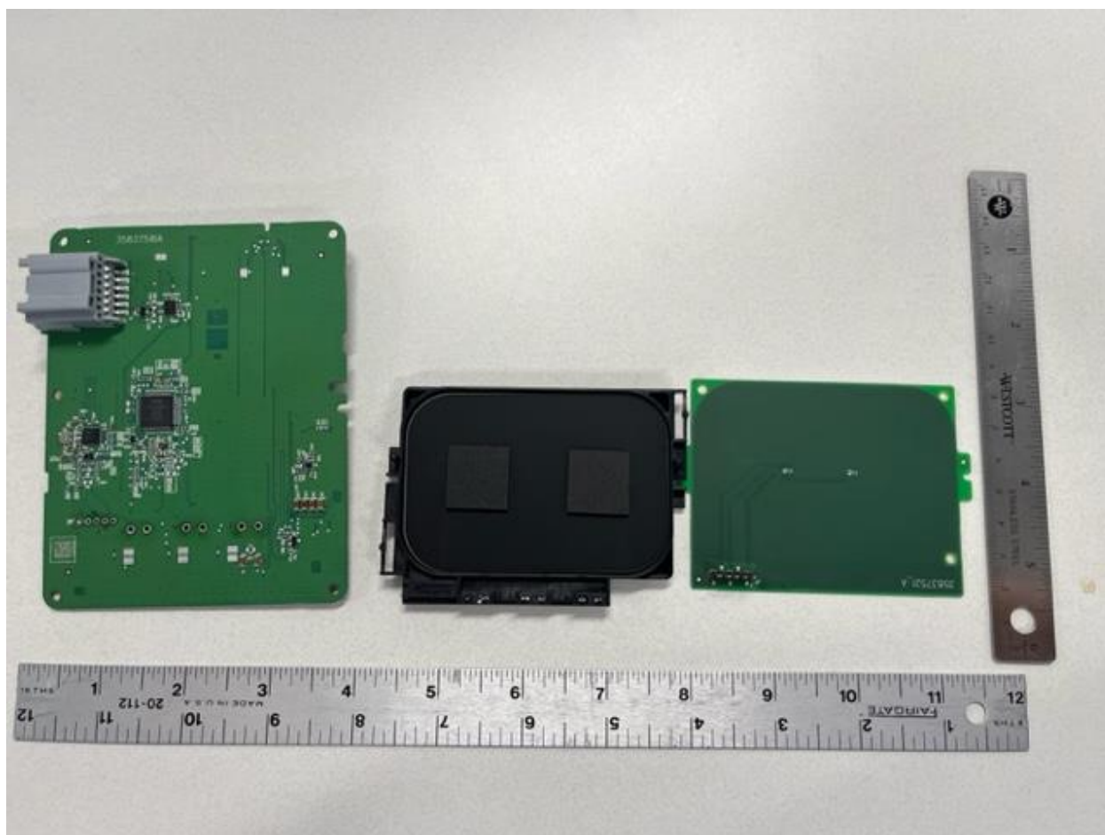
Figure 3 4196 PCBs Top
