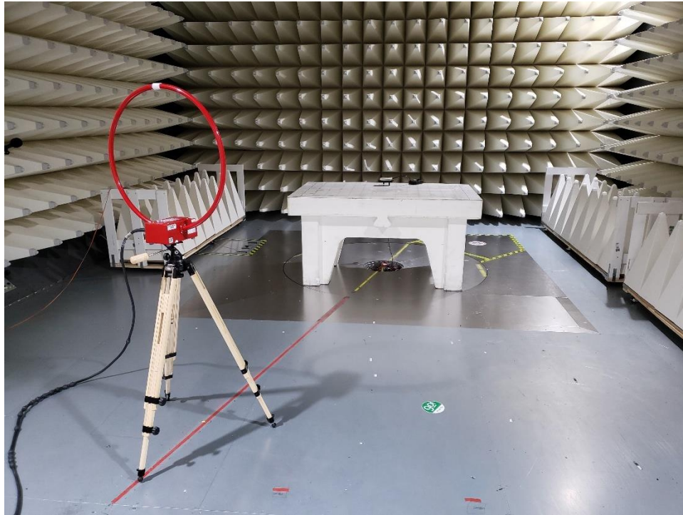
5. Low Range Radiated Emission test setup 9KHz to 30MHz
