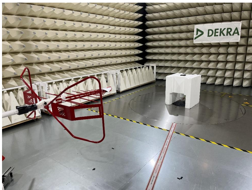
Figure B.6: Radiated Test setup 2
