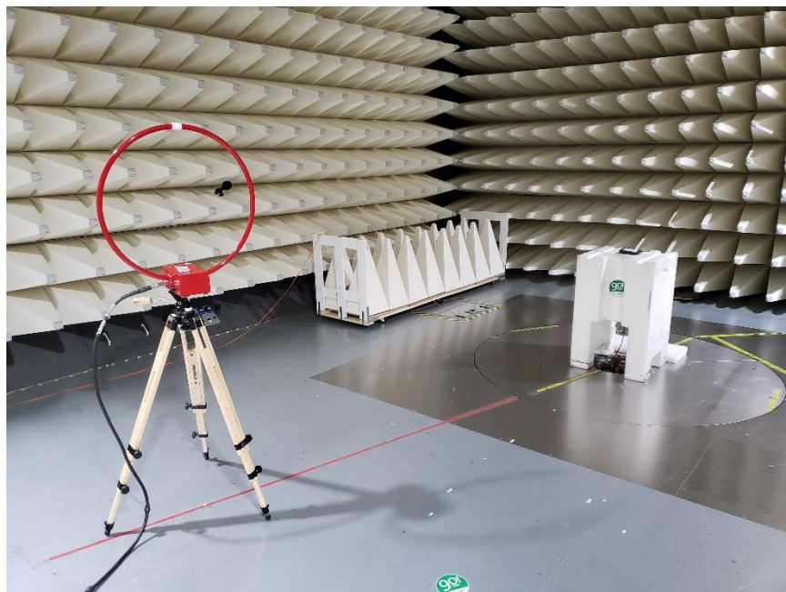
Figure B.5: Radiated Test setup 1
