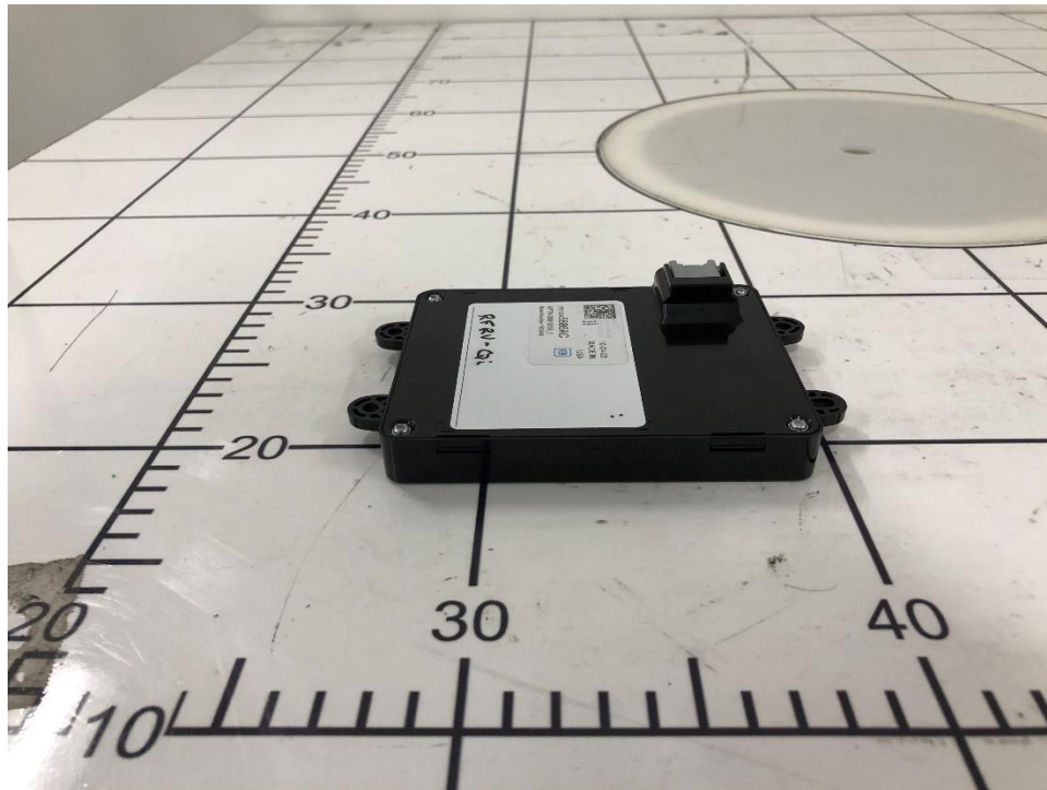
5. Top View of the DUT
