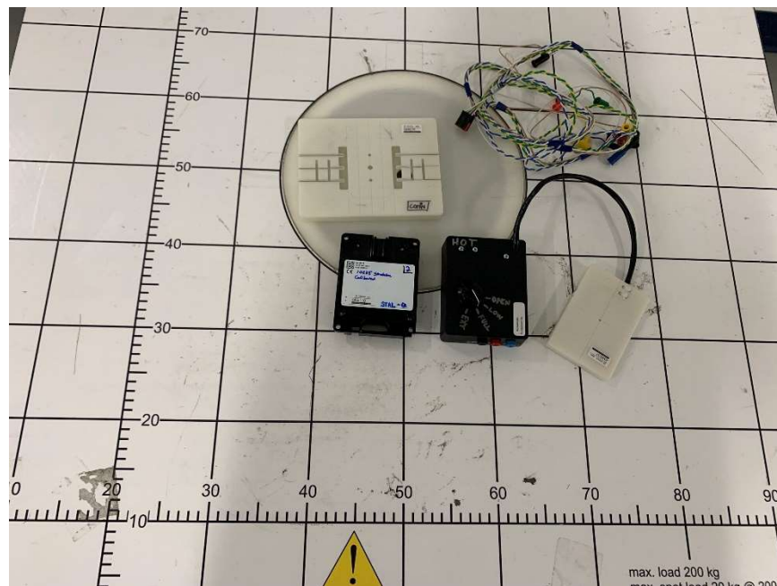
6. View of the DUT and accessories
