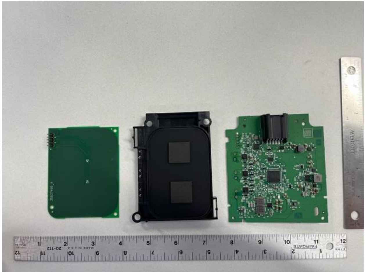
Figure 1 4200 PCBs Top
