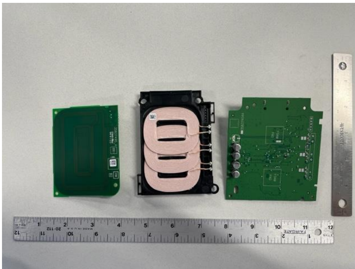
Figure 2 4200 PCBs Bottom
