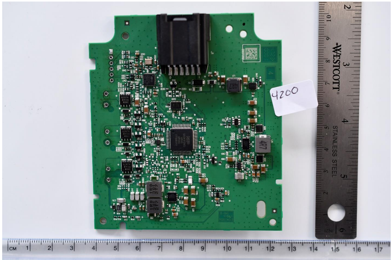
Figure 3 PCB side 1
